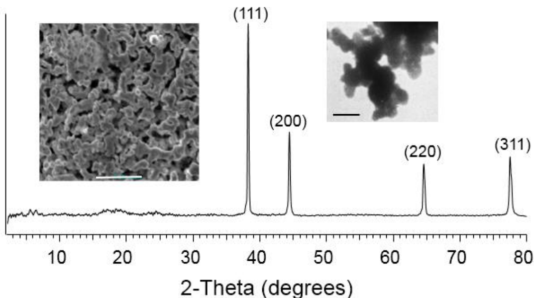
Figure 6. XRD patterns of crystalline porous Au from direct pyrolysis of compound 1 . (Inset left) SEM image of the porous gold morphology, scale bar 5μm. (Inset right) TEM image: agglomerated crystals of the structure of the porous gold, scale bar 1.5μm.
