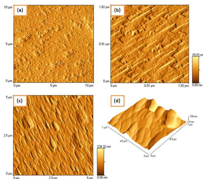
Fig. 8 AFM images of (a,b) the deposited pyrolytic products from (3) on silicon surface and (c,d) the deposited pyrolytic products from (4) on silicon surface.
