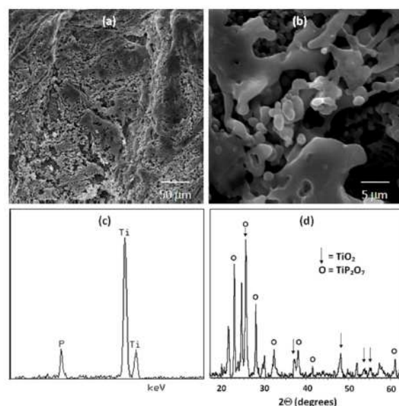
Fig. 3 (a,b) SEM at several magnifications (c) EDAX and (d) XRD pattern, of the pyrolysis product from precursor (5).
