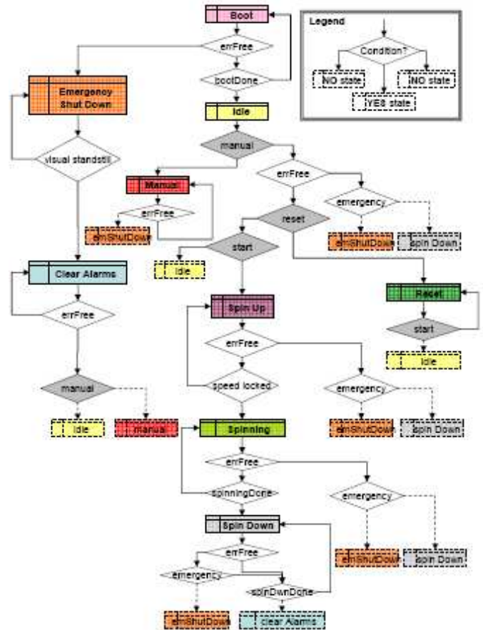
Figure 9 State machine - state diagram
