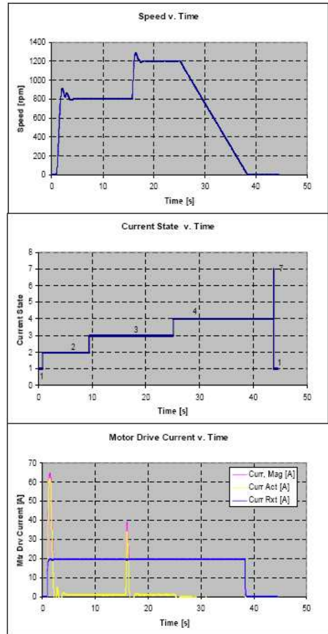
Figure 13 Speed, current state and motor drive current
