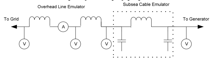
Figure 4 Single line diagram of the line emulator indicating voltage and current measurement points
