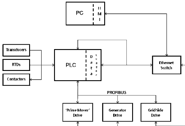
Figure 5 Control system communication diagram
