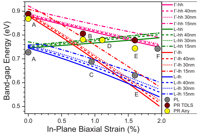
FIG. 8. Theoretical band-gap-strain dependence for Ge calculated using a 30 \times 30 \mathbf{k} \cdot \mathbf{p} model taking into account quantization-induced band-gap enhancement at decreased \varepsilon -Ge layer thicknesses for 40-, 30-, and 15-nm quantum wells. Experimental peaks given by PL and PR data are shown as circles over theoretically predicted transitions from \Gamma and L valley to light (lh) and heavy (hh) holes.
