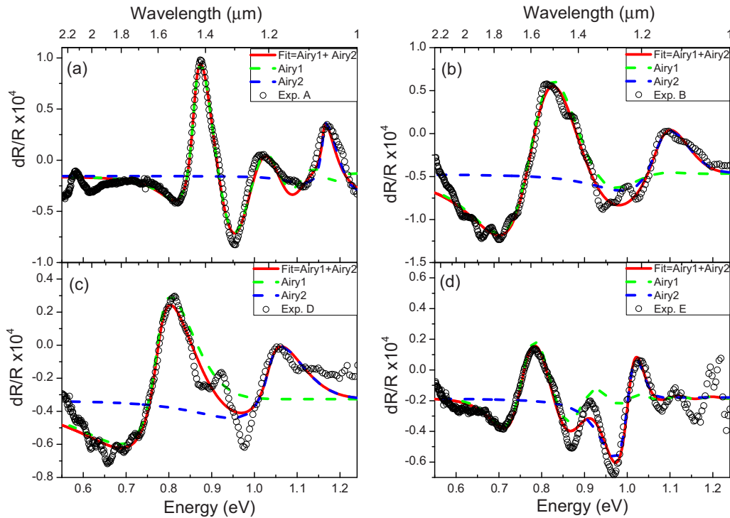
FIG. 7. Photorelectance spectrum of Ge under \varepsilon : (a) 0%, (b) 0.82%, (c) 1.11%, (d) 1.6% biaxial tensile strain at 80 K, fitted with two Airy functions. Dotted lines correspond to the experimental data, red lines are the fit including two Airy functions, depicted in green and blue, respectively.
