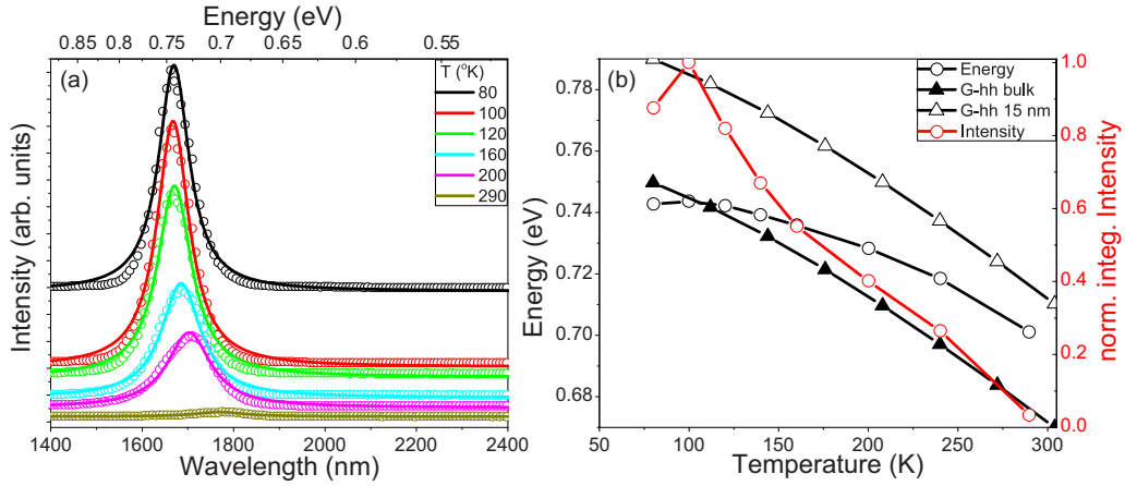
FIG. 4. (a) Photoluminescence spectra of InGaAs/Ge/In 0.29 Ga 0.71 As/GaAs (sample F) under \varepsilon = 1.94\% biaxial tensile strain depending on temperature; (b) experimental (circles) and calculated (triangles) peak energy (black line) and normalized integrated intensity (red line) versus temperature.
