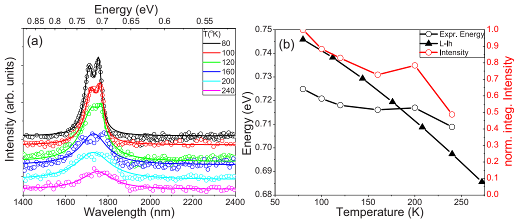
FIG. 1. (a) Photoluminescence spectra of Ge/AlAs (sample A) under \varepsilon = 0\% biaxial tensile strain depending on temperature; (b) experimental (circles) and calculated (triangles) peak energy (black line) and normalized integrated intensity (red line) versus temperature.
