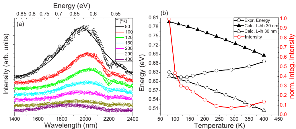
FIG. 3. (a) Photoluminescence spectra of Ge/In 0.24 Ga 0.76 As (sample E) under \varepsilon = 1.6\% biaxial tensile strain depending on temperature; (b) experimental (circles) and calculated (triangles) peak energy (black line) and normalized integrated intensity (red line) versus temperature.
