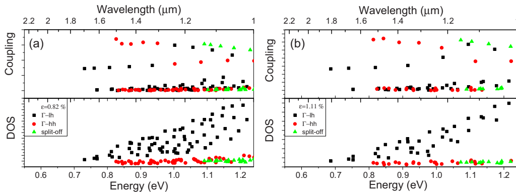
FIG. 11. \mathbf{k} \cdot \mathbf{p} calculations of electron-hole wave-function coupling and density of states (DOS) for subband transition energies in (a) 40-nm Ge quantum well with \varepsilon = 0.82\% biaxial tensile strain; (b) 30-nm Ge quantum well with \varepsilon = 1.11\% biaxial tensile strain.
