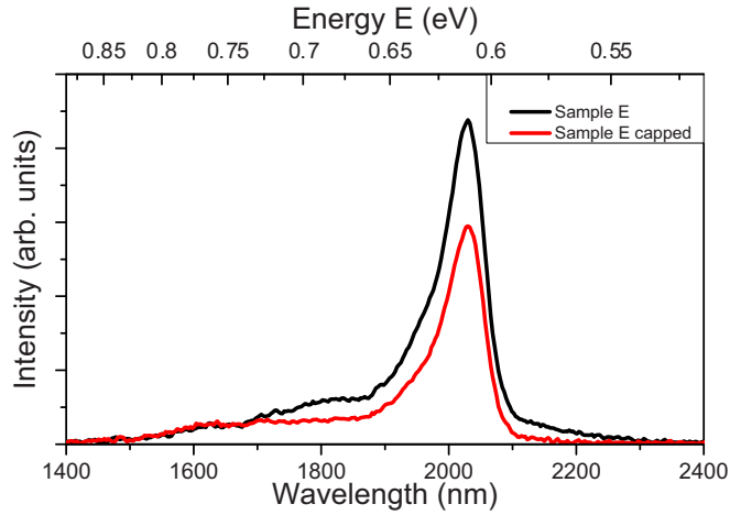
FIG. 10. Photoluminescence spectra of Ge/In 0.24 Ga 0.76 As/GaAs (sample E) and InGaAs/Ge/In 0.24 Ga 0.76 As/GaAs (sample E capped) under \varepsilon = 1.6\% biaxial tensile strain at 8 K.
