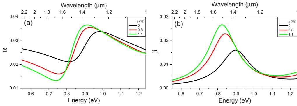
FIG. 12. Calculated (a) \alpha and (b) \beta Seraphin-Bottka coefficients in Ge at 80 K and at 0%, 0.8%, and 1.1% biaxial tensile strain.
