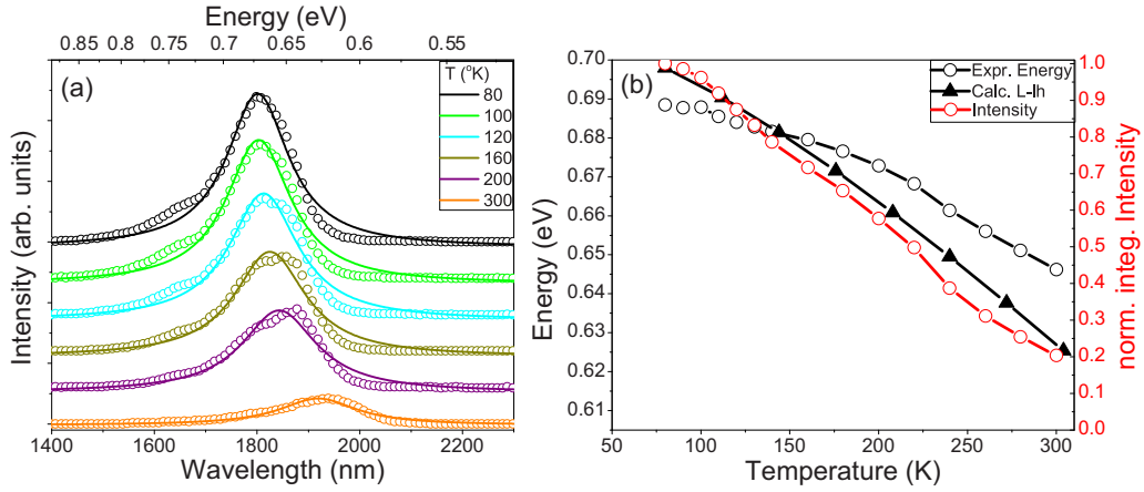
FIG. 2. (a) Photoluminescence spectra of GaAs/Ge/In 0.16 Ga 0.84 As/GaAs (sample C) under \varepsilon = 0.95\% biaxial tensile strain depending on temperature; (b) experimental (circles) and calculated (triangles) peak energy (black line) and normalized integrated intensity (red line) versus temperature.
