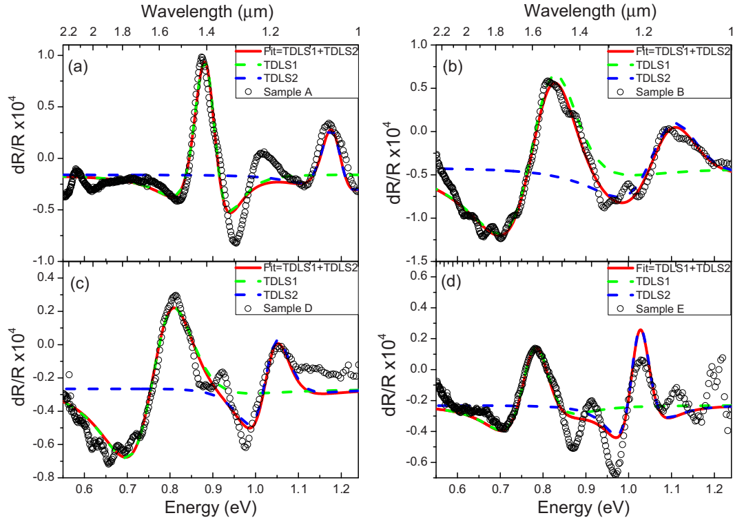
FIG. 6. Photoreflectance spectrum of Ge under \varepsilon : (a) sample A, 0%; (b) sample B, 0.82%; (c) sample D, 1.11%; (d) sample E, 1.6% biaxial tensile strain at 80 K, fitted with two TDLS functions. Open circles correspond to the experimental data, red lines are the fit including two TDLSs, depicted in green and blue, respectively.
