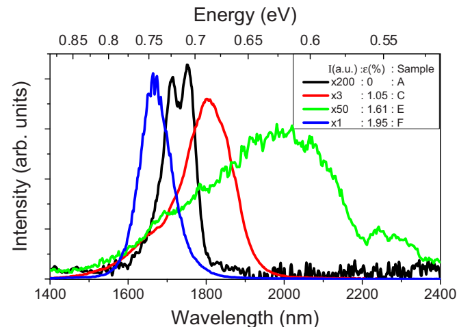
FIG. 5. PL spectra at different biaxial tensile strain (samples A, C, E, F) at 80 K.
