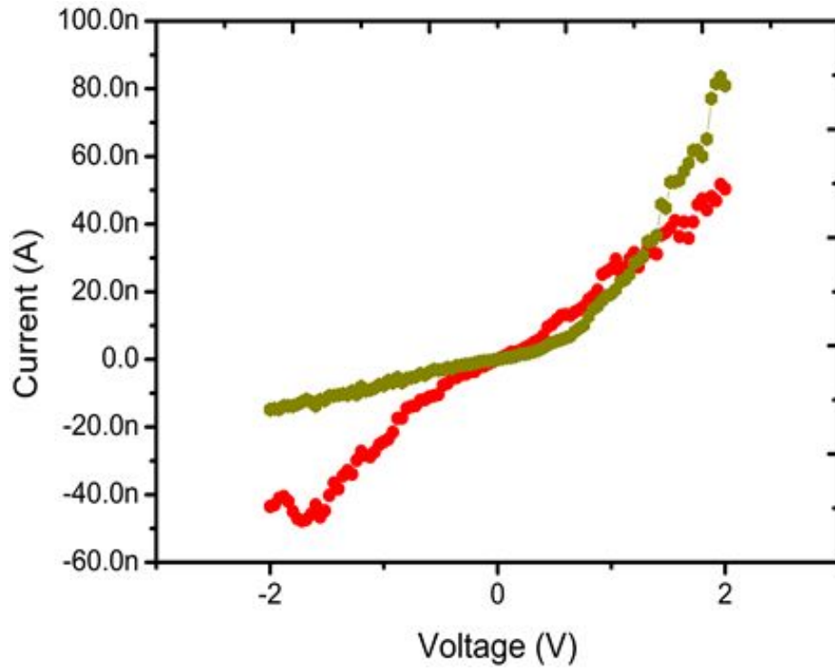
Figure S9: : Representative I_d - V_d curve for \text{Ge}_{0.90}\text{Sn}_{0.10} nanowire devices. To perform the transfer characteristics (Figure 4 in the main manuscript) nanowire FET device with red curve was selected. Transfer characteristics were performed in the linear region of V_{ds} (-1V to 1V).
