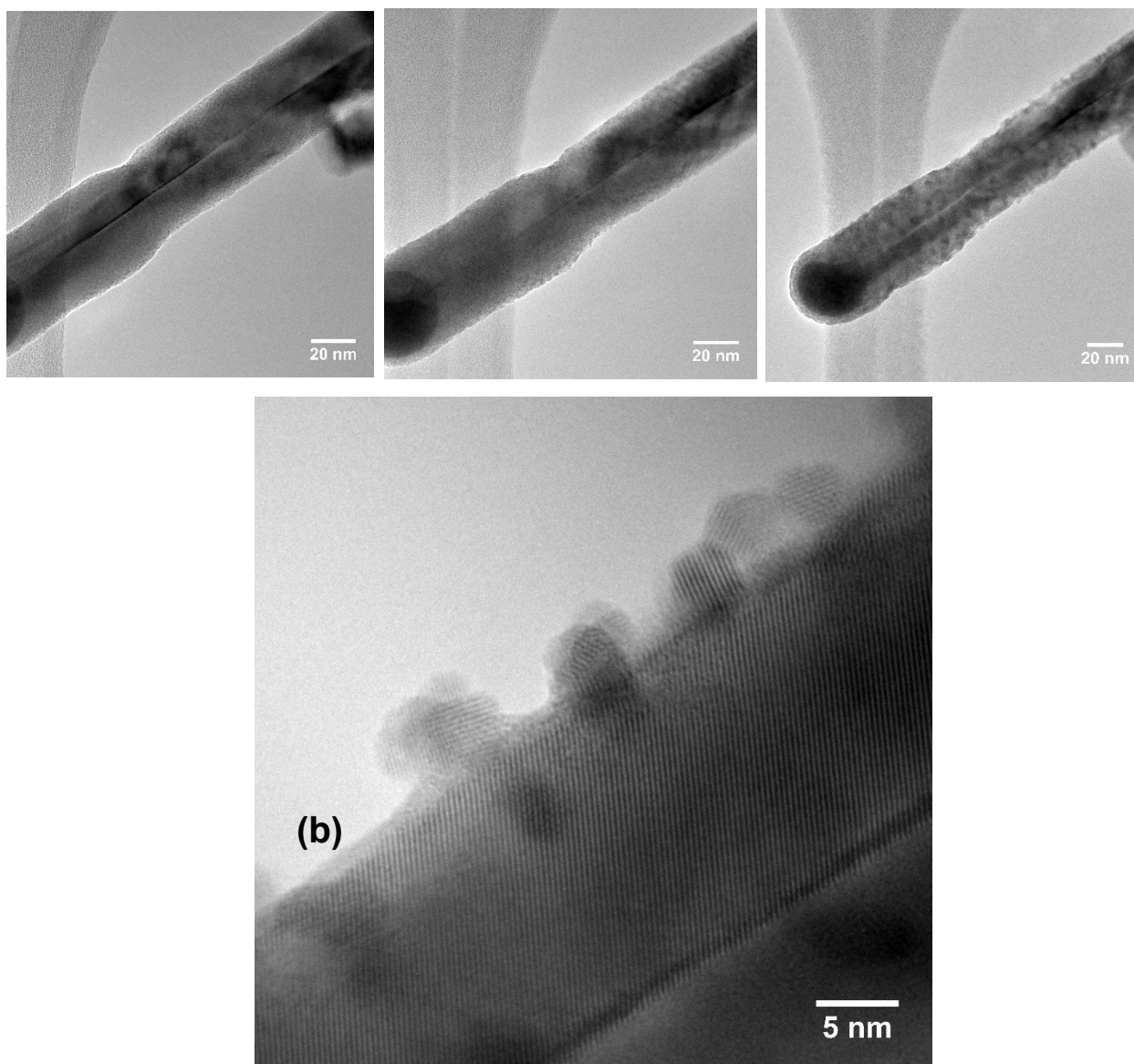
Figure S8: (a) TEM images of \text{Ge}_{1-x}\text{Sn}_x nanowires show deformation with time (with 1 min interval). (b) No apparent change in the crystal lattice was observed for the deformed and non-deformed area of the nanowire.
