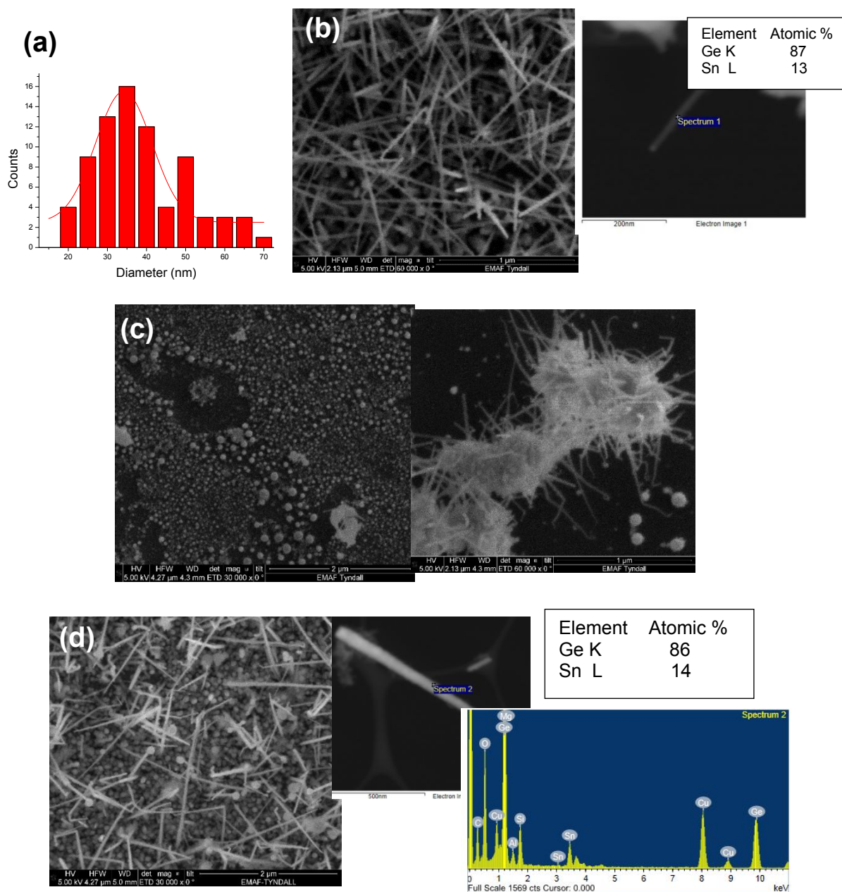
Figure S1: (a) Diameter distribution of GeSn nanowires. (b) SEM image and corresponding EDX analysis of \text{Ge}_{1-x}\text{Sn}_x nanowires grown at 430 °C, with other growth parameters similar to the standard growth parameters (21 MPa pressure, AuAg alloy catalysts, DPG and ATBS as Ge and Sn source). (c) SEM images show \text{Ge}_{1-x}\text{Sn}_x nanowires (or lack of it) grown with Au catalyst. (d) SEM image and corresponding EDX analysis of the \text{Ge}_{1-x}\text{Sn}_x nanowires grown with TET Sn precursor. Sample shows large amount of spherical segregation, tapered nanowires and nanowire with 8-15 at.% Sn.
