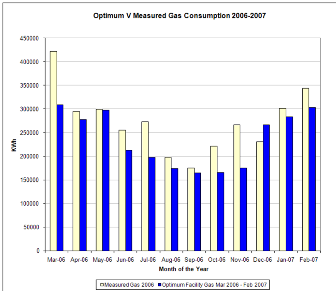
Figure 7.8: Example of Building Gas Consumption for the Profiled Energy Manager
