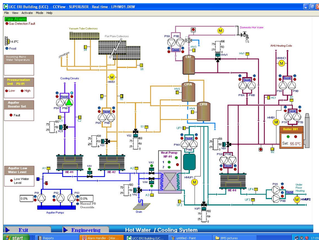
Figure 9.2: Screen Shot Image of the ERI BMS Illustrating the Integrated Hybrid Heating and Cooling System
