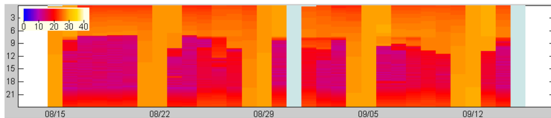
Figure 7.9: Sample Carpet Plot that is to display Performance Metrics for the Profiled Energy Manager (Courtesy of Isakson 2004)
