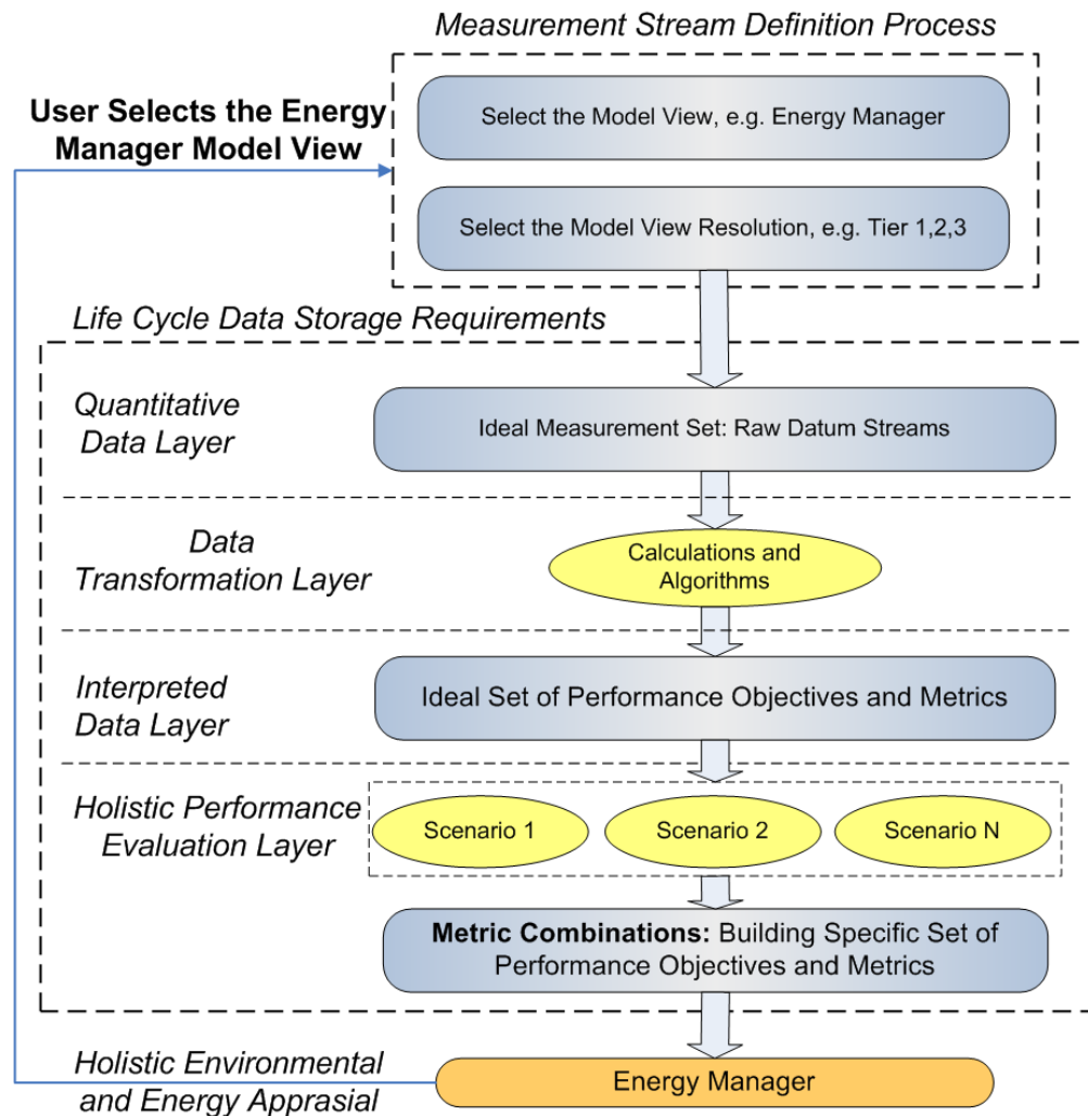
Figure 6.2: High Level Overview of the Automated Process and Rule Set Relationships as applied with the Ideal Building Framework
