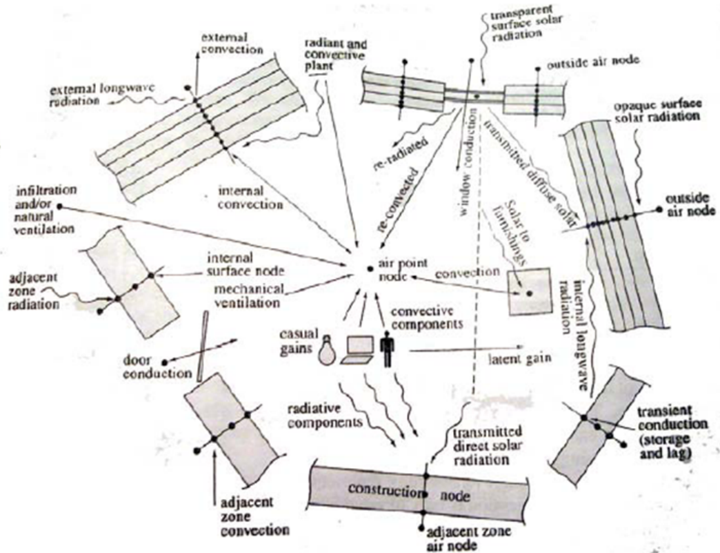
Figure B.1: The Complexity of Building Energy Flows (Courtesy of (Clarke 2001))
