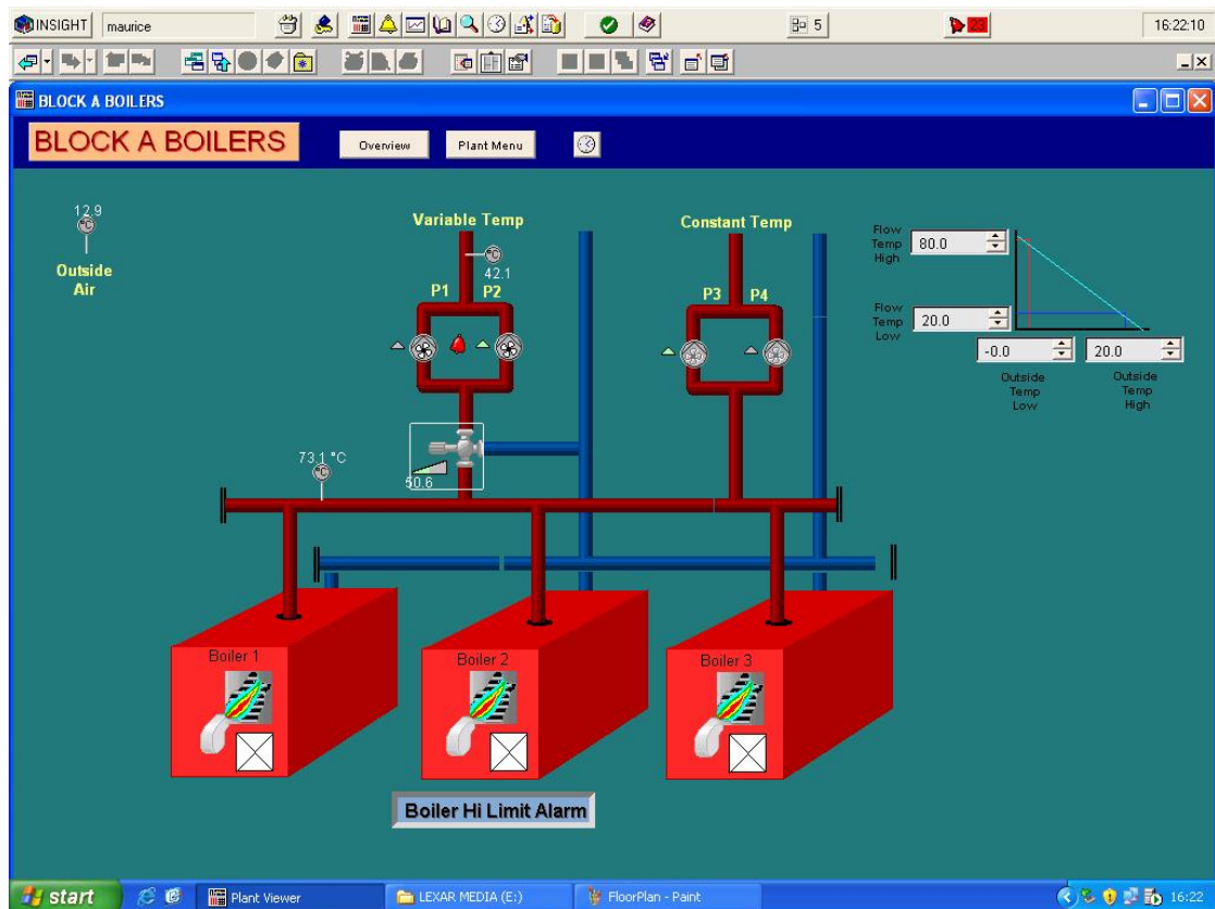
Figure 2.5: Siemens BMS Screen Shot of Block A Boilers System at the University College Cork Student Center
