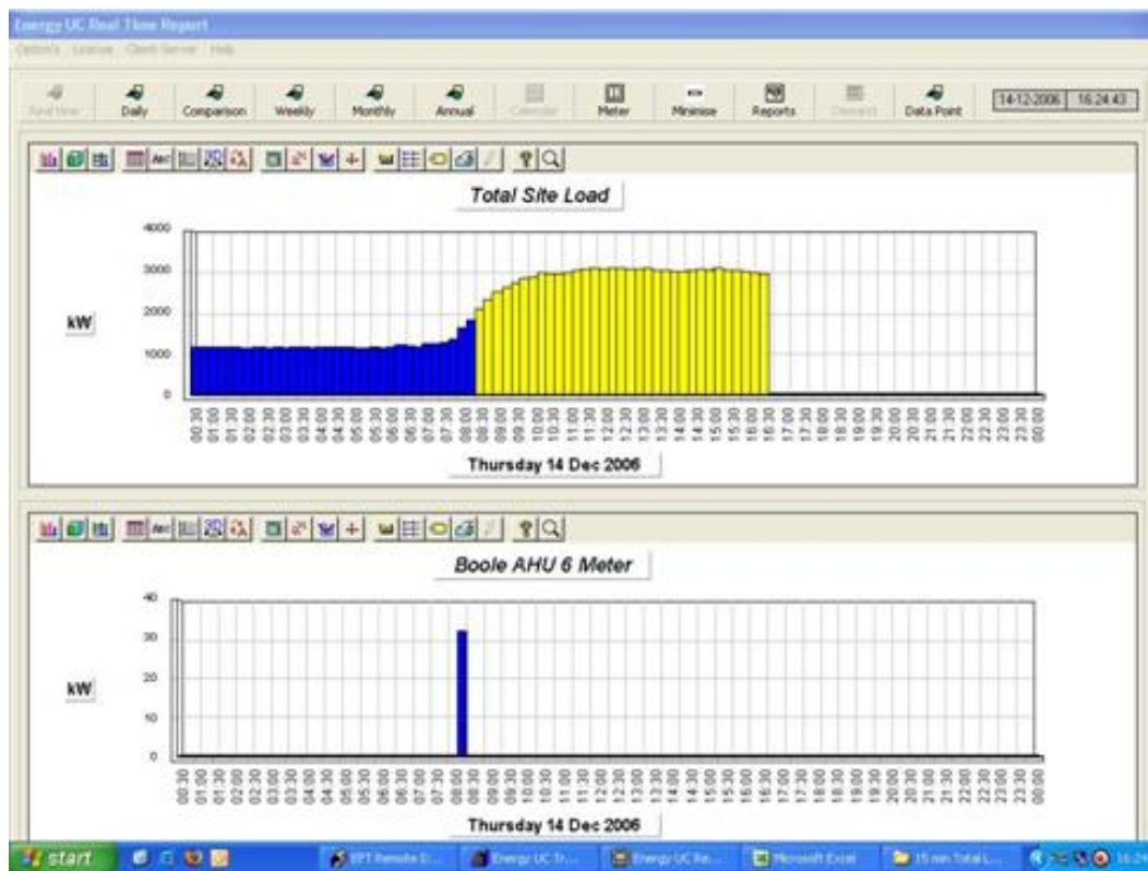
Figure A.2: Typical College Weekday Electricity Load Profile for UCC Site. Displayed by the EnergyFocus EMS.
