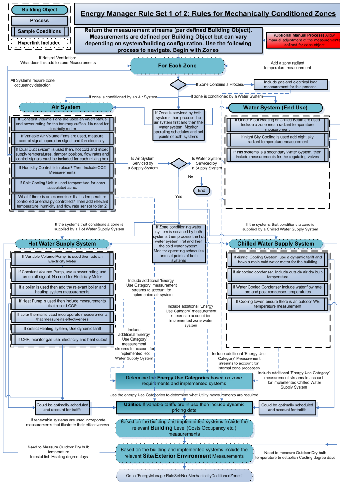
Figure 6.4: Energy Manger Rule Set for Mechanically Conditioned Spaces. Appendix G contains a fully interactive image.
