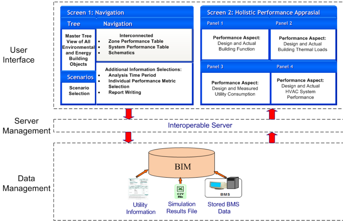
Figure C.1: Information Delivery Tool: System Architecture
