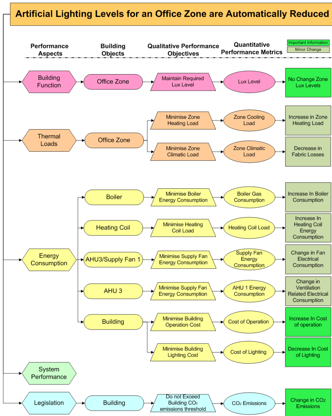
Figure 3.8: Scenario Illustration Depicting the Effects of an Automated Reduction in Zone Lighting while maintaining Zone Lux Setpoints
