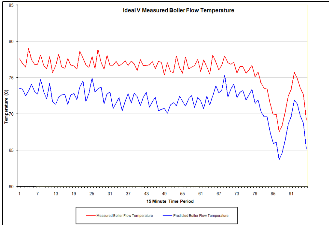
Figure 7.7: Example Plot of a Boiler Flow Temperature Performance Metric for the Profiled Energy Manager
