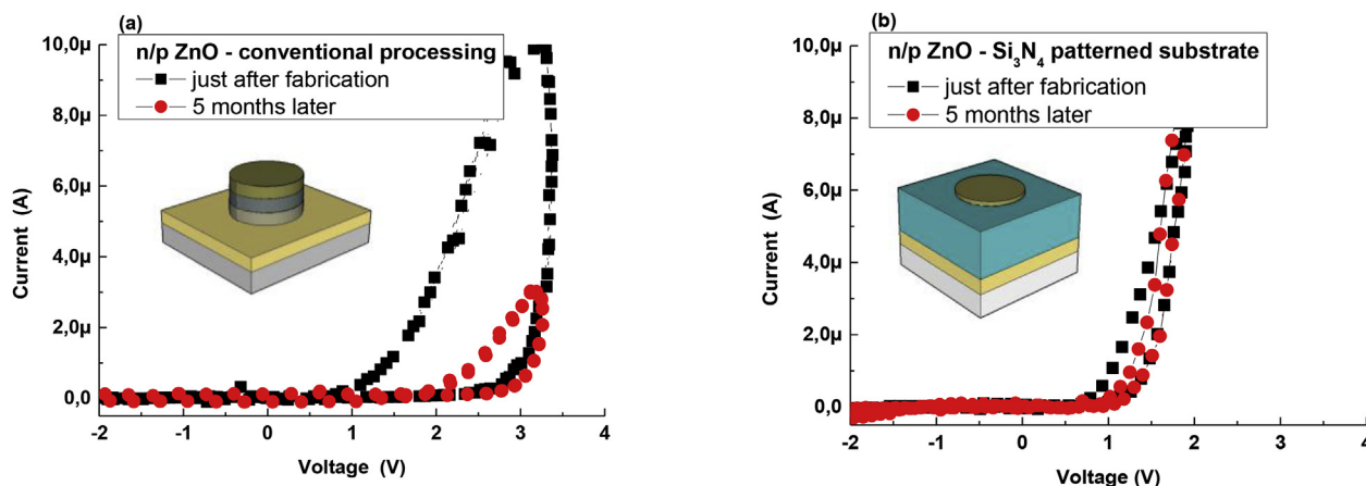
Fig. 4. I-V characteristics of n/p ZnO homojunctions processed (a) 'conventional' non-patterned substrate and (b) on Si 3 N 4 -patterned substrate just after fabrication and after five (5) months. The inset shows schematic representations of the diodes, the cross-section of which are seen Fig. 1.
