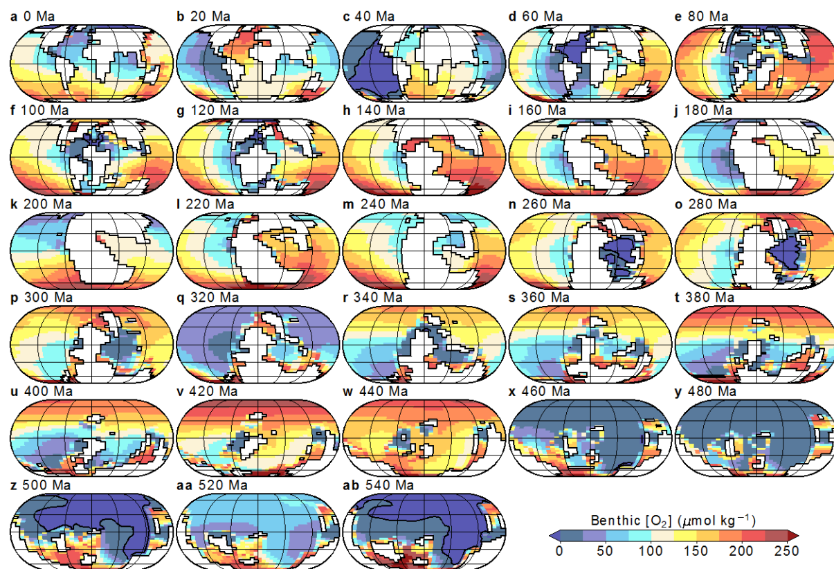
Extended Data Figure 6. Benthic oxygen concentrations for simulations at 2240 ppm CO 2 (like #1) but with no mid-ocean ridges (see Extended Data Fig. 7). Results are averaged over the last 5000 years. Emerged continental masses are shaded white. Eckert IV projection.
