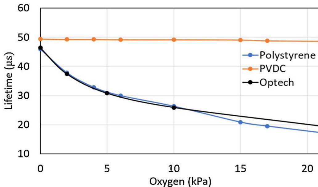
Figure 4.8: Lifetime response to O_2 partial pressure for the polystyrene, PVDC and Optech (Mocon) sensors/coatings at 25 °C (Sen, Zhdanov, Hirvonen, et al., 2020b).
