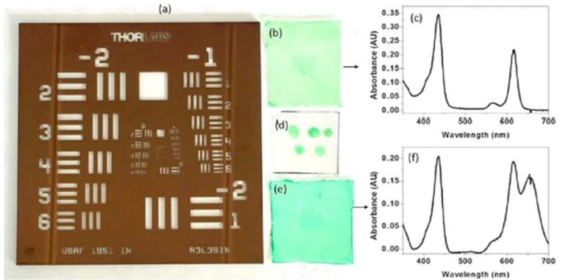
Figure 3.2: Samples used to characterize the imager: (a) USAF resolution test target; (b) Planar PtBP-RL100 based O_2 sensor film and (c) its absorption spectrum; (d) PtBP-RL100 sensor spots on PVDF membrane, (e) Sensor film with PtBP and aza-Bodipy dyes in RL100, and (f) its absorption spectrum. Spectra were measured on an 8453UV-Visible spectrophotometer (Agilent). Adapted from (Sen, Hirvonen, et al., 2020).
