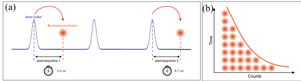
Figure 1.6: (a) Measurement and (b) histogram of start-stop times in time-resolved fluorescence measurement with TCSPC (Wahl, 2014).
