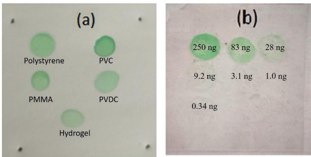
Figure 4.1: Exemplary photographs of arrays of the phosphorescent coatings with 250 ng of PtBP dye in the different polymers (a) and with decreasing PtBP concentration in one polymer (seven serial 1:3 dilutions) (b), spotted on planar solid support. Spot size is 2-3 mm across (Sen, Zhdanov, Hirvonen, et al., 2020b).
