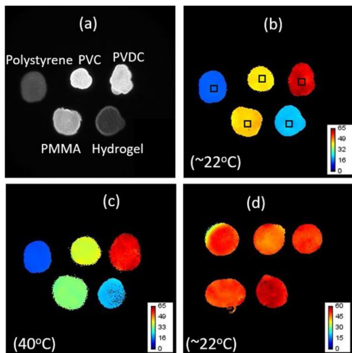
Figure 4.2: Images of the different phosphorescent coatings spotted on polyester film. (a) Grey scale intensity images; (b) PLIM images at room temperature; (c) PLIM images of the sensors obtained at 40 °C; (d) PLIM images of the sensors obtained under zero \text{O}_2 condition at room temperature (Sen, Zhdanov, Hirvonen, et al., 2020b). Images were acquired for 20 seconds with LED at 4V with pulse width of 50 ns.
