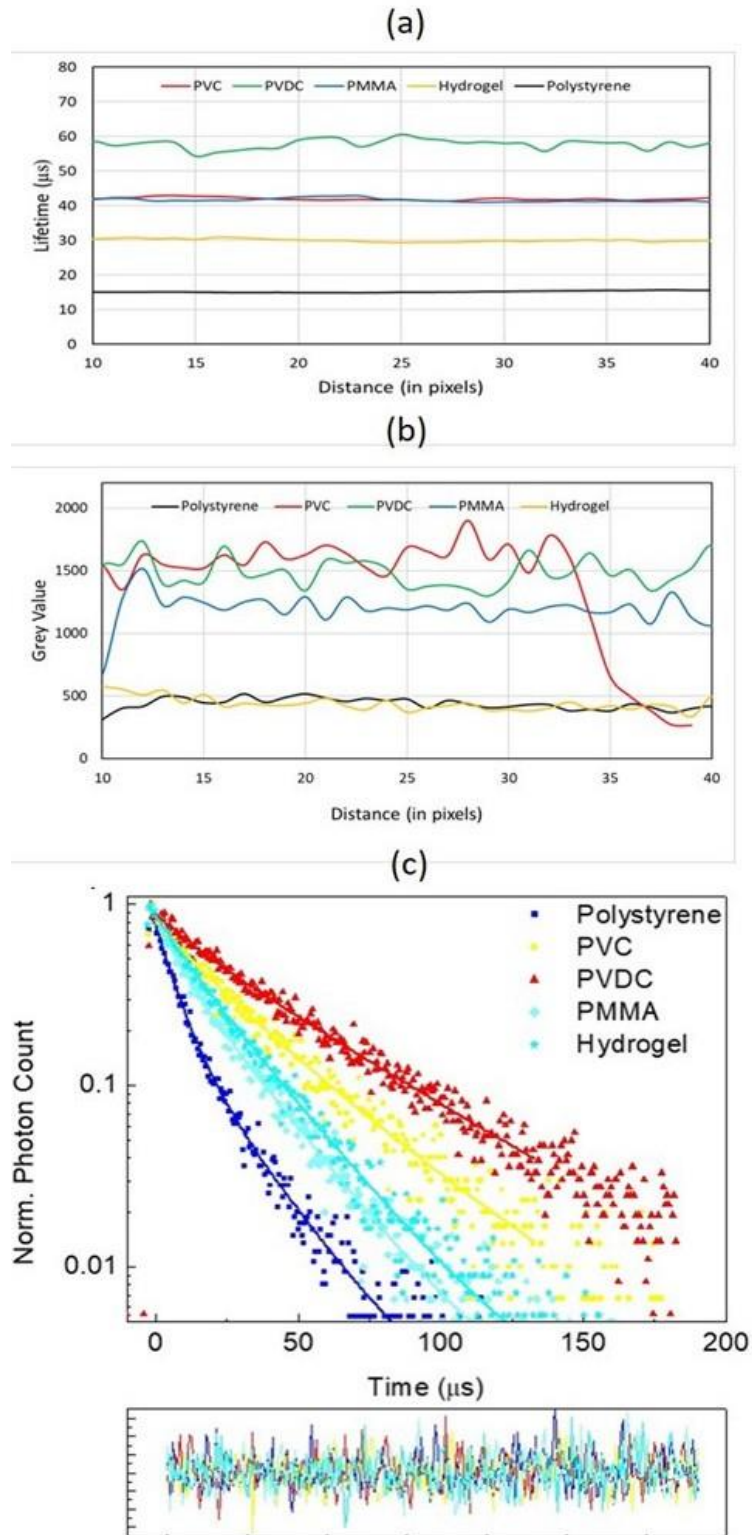
Figure 4.3: Graphs representing (a) line profile across the sensor spots for the PLIM images shown in Figure 4.2b; (b) line profile across the sensor spots for the intensity images shown in Figure 4.2a; (c) Phosphorescence decays with bi-exponential fits for the different ROIs marked in Figure 4.2b (Sen, Zhdanov, Hirvonen, et al., 2020b).
