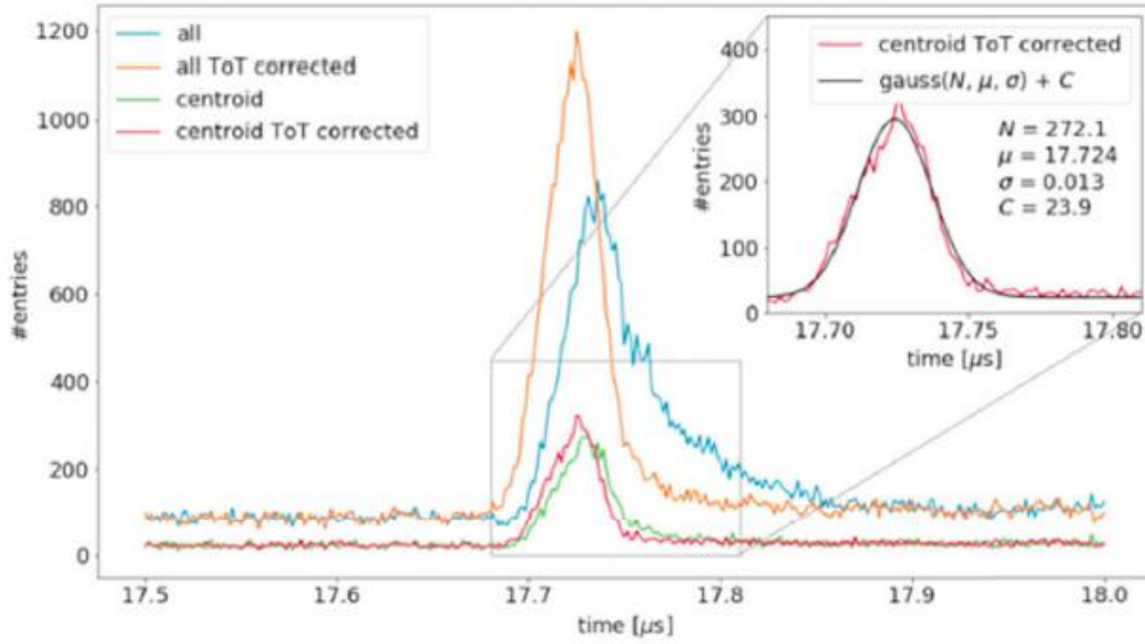
Figure 3.5: Instrument Response Function (IRF) position in the measurement time interval is shown for all hit pixels and for the centroided pixels. In both cases the distributions are shown before and after the TOT correction. Gaussian fit of the centroided and TOT corrected distribution corresponds to the IRF FWHM of 30.6 ns. Background was described with a constant in the fit (Sen, Hirvonen, et al., 2020).
