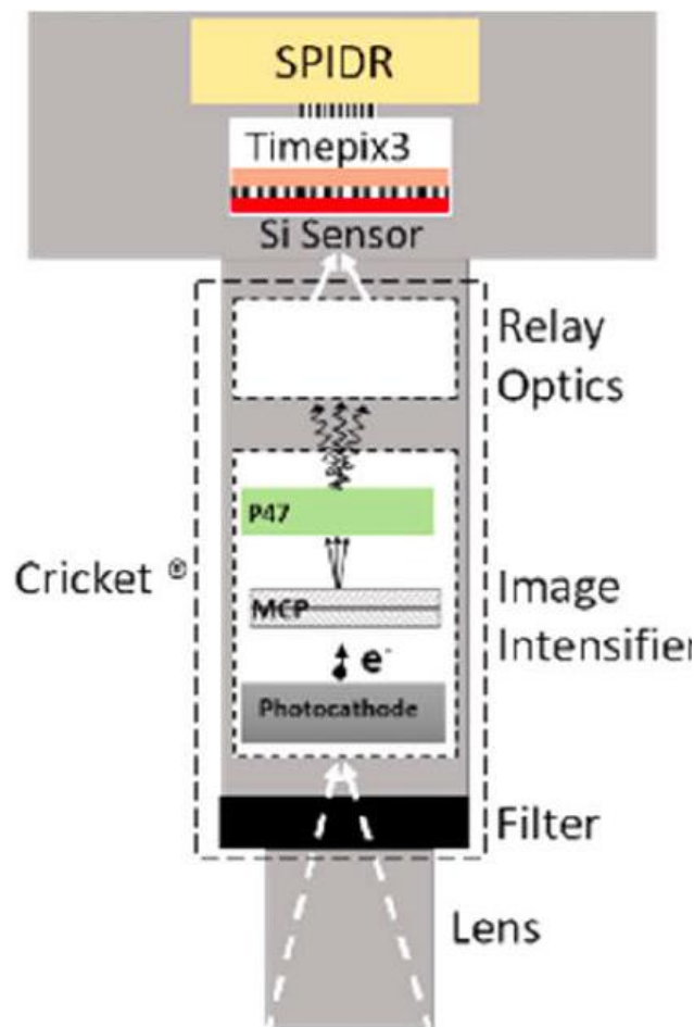
Figure 1.9: Schematic layout of the intensified Tpx3Cam camera (Sen, Hirvonen, et al., 2020).
