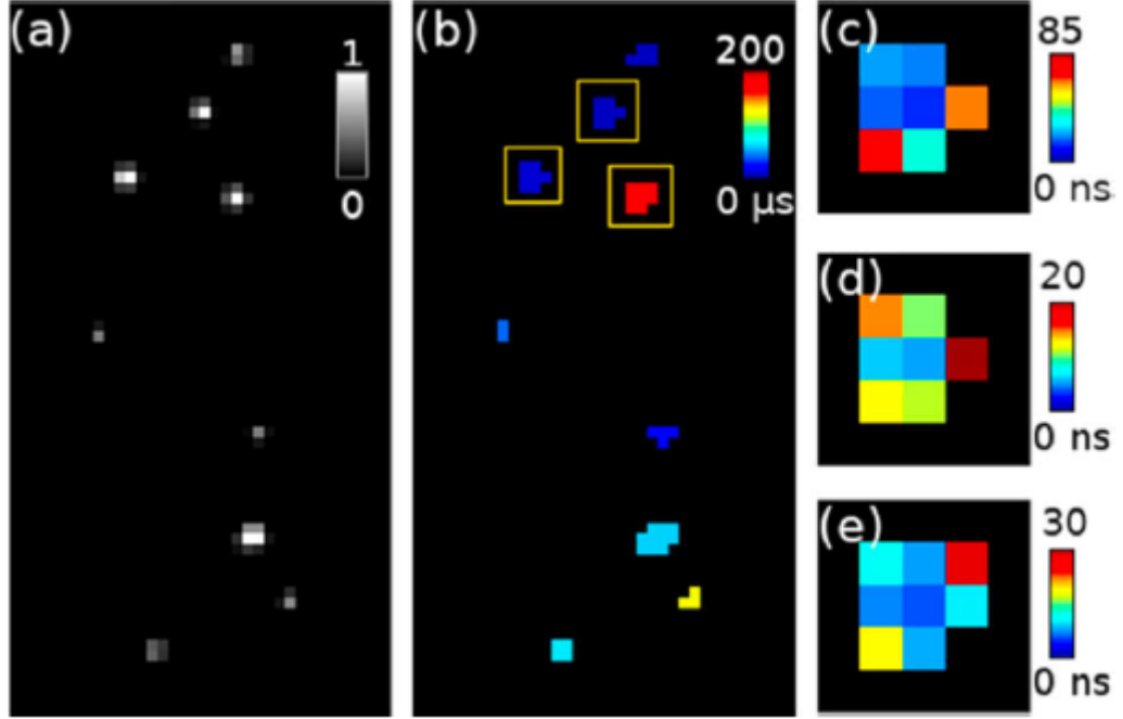
Figure 3.3: Single photon events detected with the Tpx3Cam setup. (a) TOT, i.e., intensity, (b) arrival time, (c-e) Re-scaled arrival time for individual photon events showing the “timewalk” effect (Sen, Hirvonen, et al., 2020).
