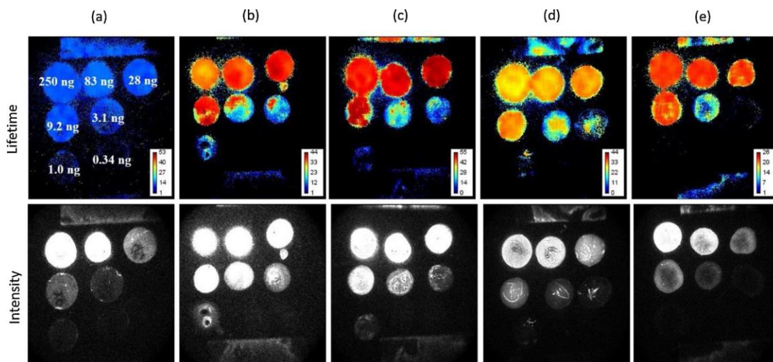
Figure 4.9: PLIM (top row) and intensity (bottom row) images of the sensor palettes prepared using the cocktails with 1:3 serial dilutions of PtBP dye in: (a) Polystyrene, (b) PVC, (c) PVDC, (d) PMMA and (e) Hydrogel D4 (Sen, Zhdanov, Hirvonen, et al., 2020b).
