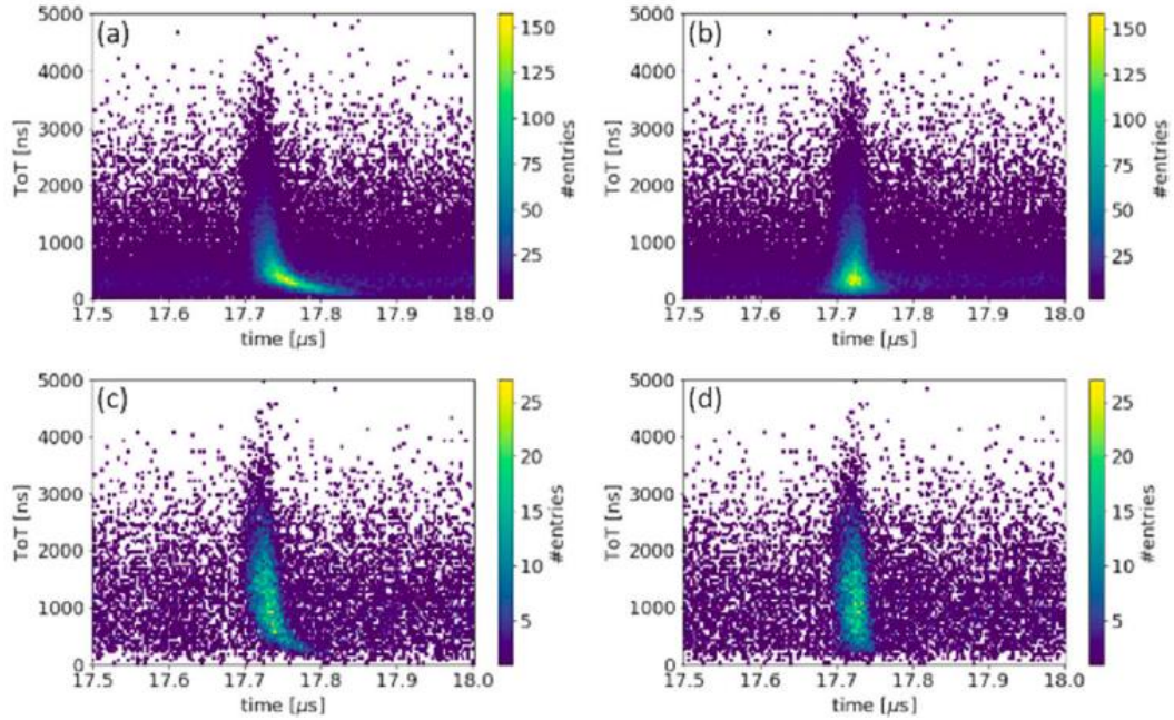
Figure 3.6: Two-dimensional distributions of time, in microseconds, versus TOT, in nanoseconds, for four cases: (a) all hit pixels; (b) all hit pixels with TOT correction applied; (c) centroided pixels; (d) centroided pixels with TOT correction applied (Sen, Hirvonen, et al., 2020).
