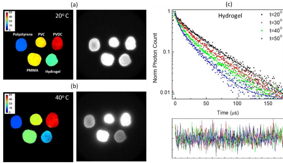
Figure 4.4: Images of the polymeric phosphorescent coatings on polyester support taken on the Tpx3Cam imager at 20°C (a) and at 40°C (b) and presented in lifetime (left) and Intensity (right) scale; (c) Normalised phosphorescence decays for the Hydrogel sensor at different temperatures (Sen, Zhdanov, Hirvonen, et al., 2020b).
