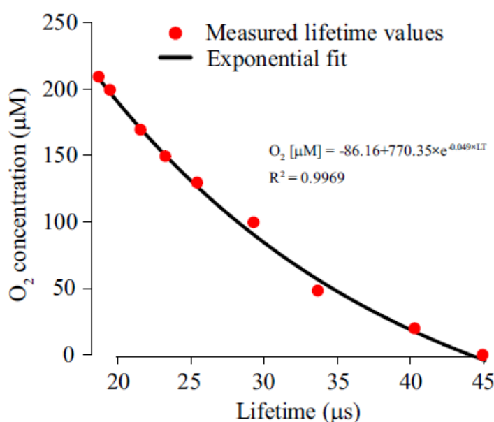
Figure 5.2: \text{O}_2 calibration of NanO2-IR probe under physiological conditions. Lifetime values were measured with a handheld reader Optech (Mocon, USA) in liquid samples (DMEM media) equilibrated with 0%, 2.0%, 5.0%, 10.0%, 12.0%, 15.0%, 17.0%, 20.0% and 21.0% \text{O}_2 gas standards produced on a gas mixer, at 37 °C. Exponential fitting was performed using https://mycurvefit.com/ (Sen, Zhdanov, Bastiaanssen, et al., 2020).
