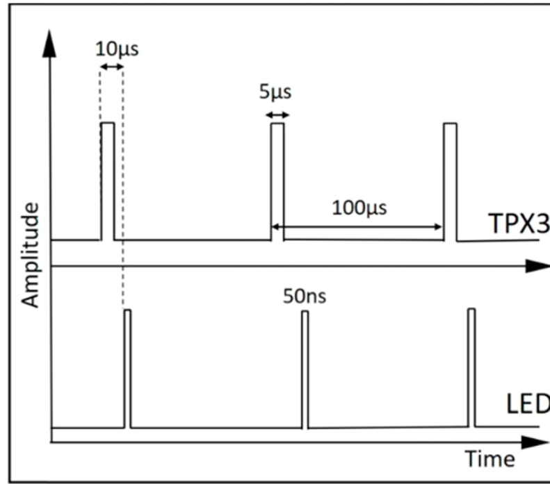
Figure 2.2: Pulsing scheme of the imager. The LED is pulsed every 100\ \mu\text{s} with 50\ \text{ns} duration of the pulse. Tpx3Cam is provided with a synchronous pulse 10\ \mu\text{s} before the LED, which is time-stamped and included into the data stream. The camera records the photon hits for 100\ \mu\text{s} until the next LED pulse (Sen, Hirvonen, et al., 2020).
