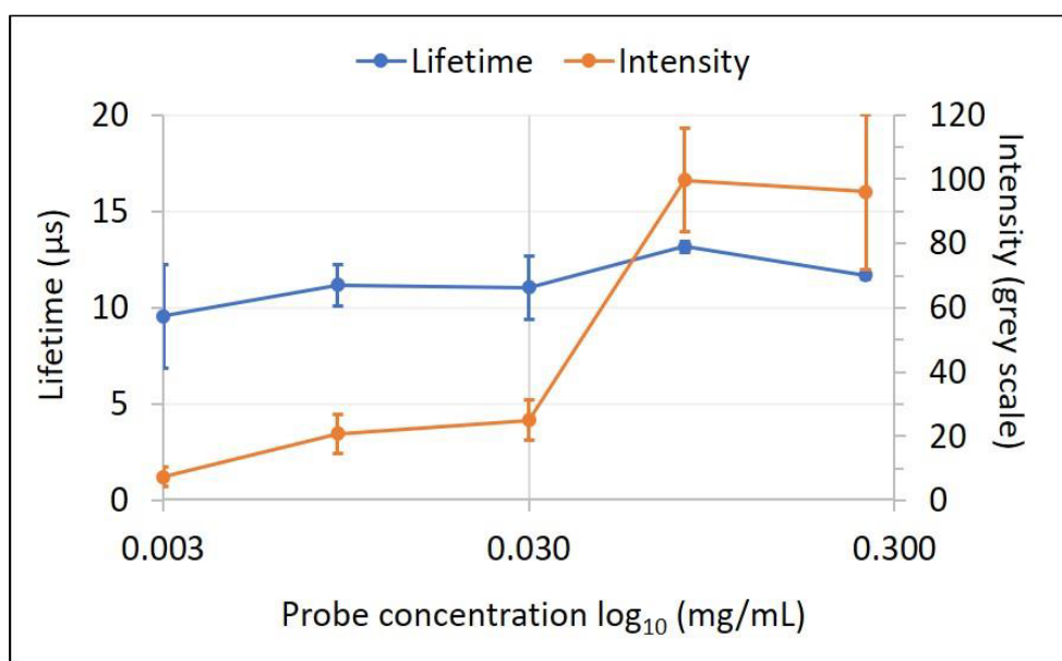
Figure 4.10: Variation of the intensity and lifetime for Polystyrene based PtBP dye with increasing dilutions (Sen, Zhdanov, Hirvonen, et al., 2020a).
