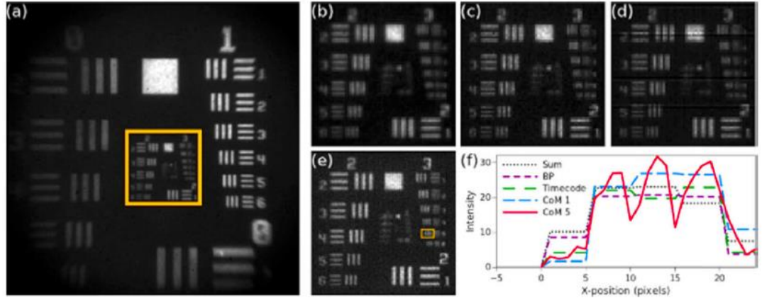
Figure 3.4: Images of 1951 USAF resolution test target overlaid on top of a phosphorescent O_2 sensor foil. (a) Sum image showing the PLIM imager field of view. (b-e) images of the area indicated in (a) centroided with different methods: (b) sum, (c) brightest pixel (BP), (d) earliest timecode, (e) center-of-mass with 1/5-pixel accuracy (CoM 5). (f) Cross-sections of the bars in the area indicated in (e), where the sub-pixel centroiding can still resolve lines with \sim 40 \mu m spacing, that cannot be resolved with the other centroiding methods (Sen, Hirvonen, et al., 2020).
