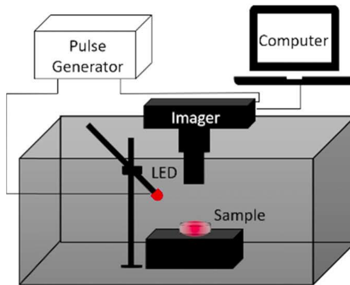
Figure 3.1: Experimental setup of the PLIM macro-imager based on Tpx3Cam (Sen, Hirvonen, et al., 2020).
