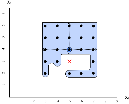
Figure 2. Neighbours of the highlighted solution.
