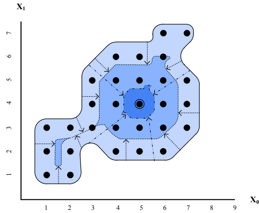
Figure 1. Restrictions over the bounds of the solution space.
