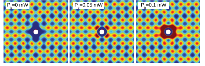
FIG. 4. (Color online) Same as Fig. 3, with the fiber placed at a maximum of intensity of the lattice. Each plot spans an area of 4.2 \mu\text{m} \times 4.2 \mu\text{m} .
