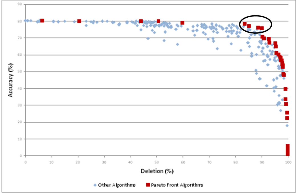
Figure 3.2: Results for twenty-five different datasets, highlighting the Pareto front
