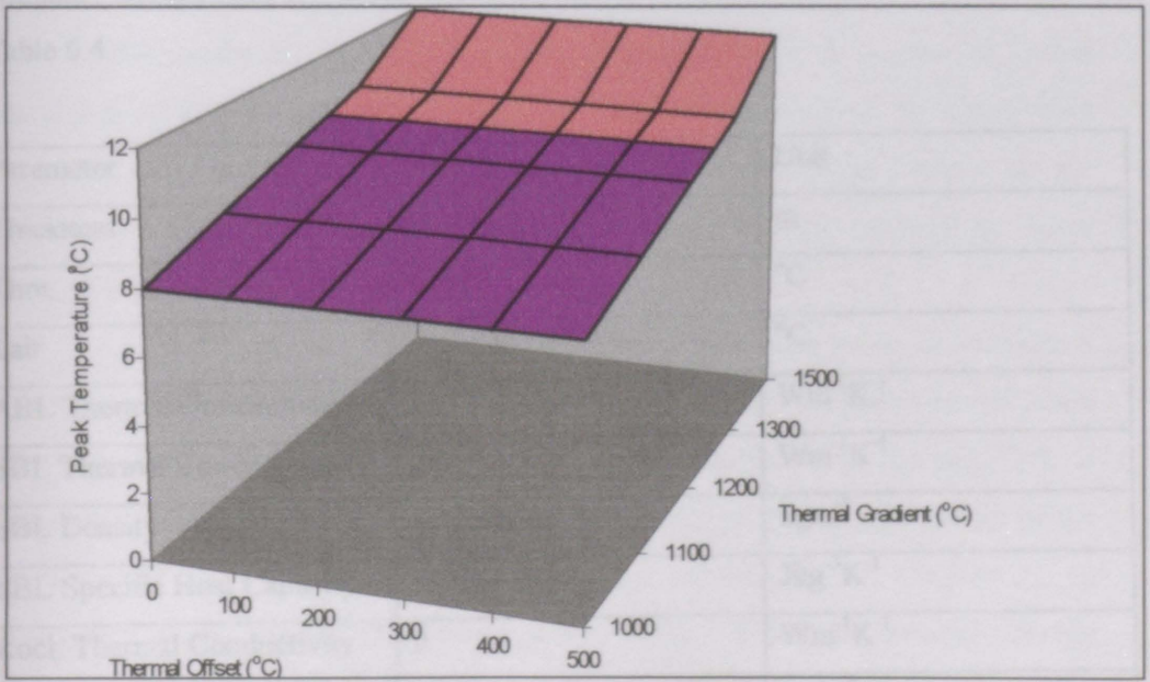
Figure 6.8 Peak Temperature vs. Gross Thermal Gradient. This figure demonstrates how a heat sources at 1400^{\circ}\text{C} ( T_{\text{hot}} ) and an atmosphere at 400^{\circ}\text{C} ( T_{\text{air}} ) will generate the same increase in surface temperature above background as a heat sources at 1000^{\circ}\text{C} ( T_{\text{hot}} ) and an atmosphere at 0^{\circ}\text{C} ( T_{\text{air}} ).
