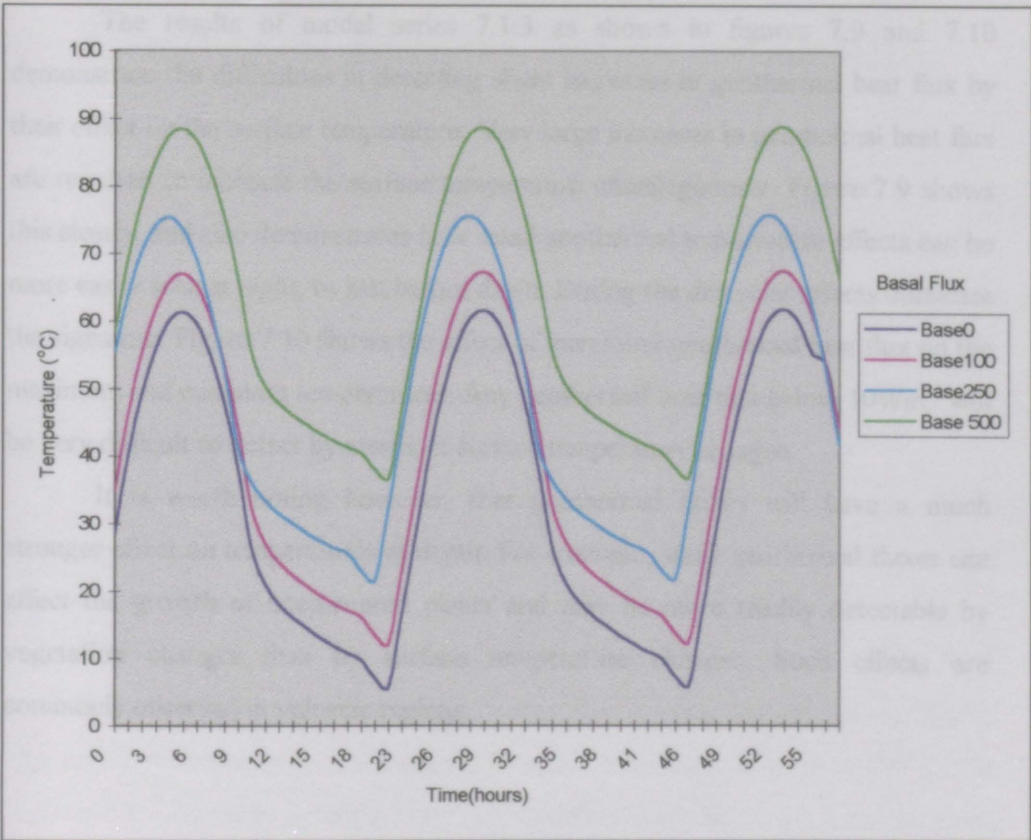
Figure 7.9 Variation in the surface temperature for identical surface loads and varying basal fluxes (0 to 500 Wm -2 )
