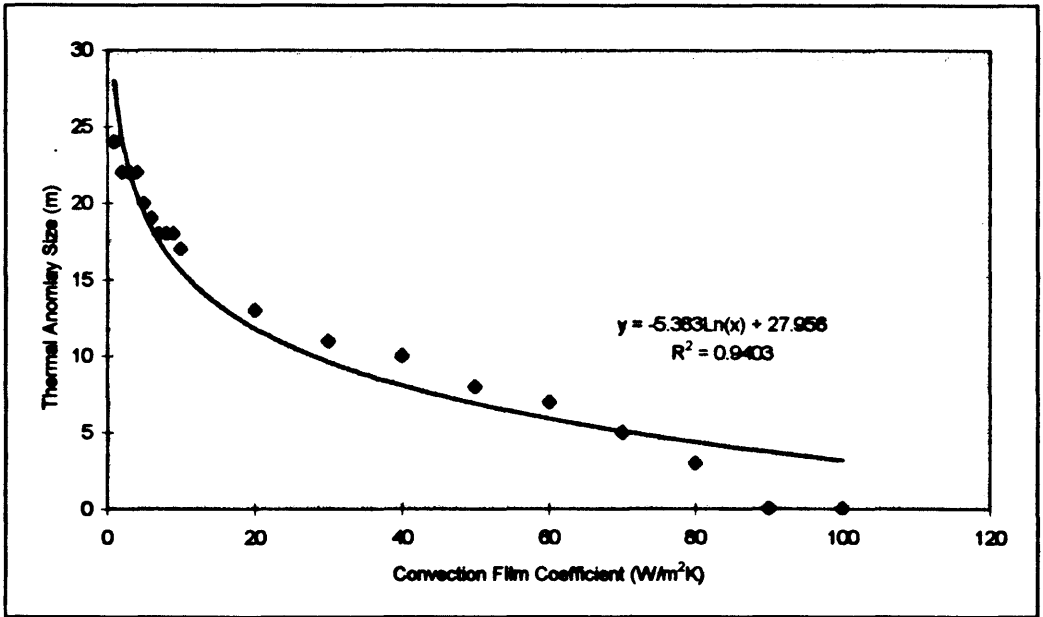
Figure 6.39 The thermal anomaly size as a function of the convection film coefficient. Note the steady reduction in the thermal anomaly size as the convection film coefficient increases.
