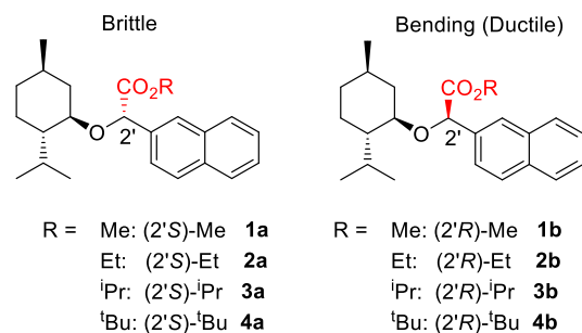
Fig. 1 The two epimeric series of substituted menthyloxy-2'-esters examined in this study.
