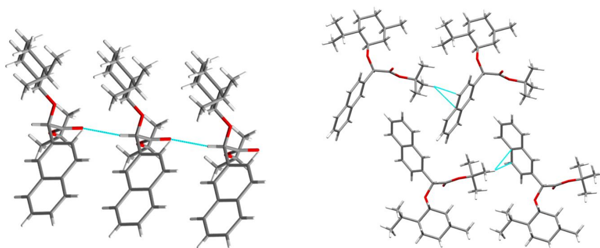
Fig. 5 Weak C-H...O interactions in (2'S)-Pr ( 3b ) crystals viewed down the b axis, left, and C-H... \pi contact in (2'S)- t Bu ( 4b ), right.
