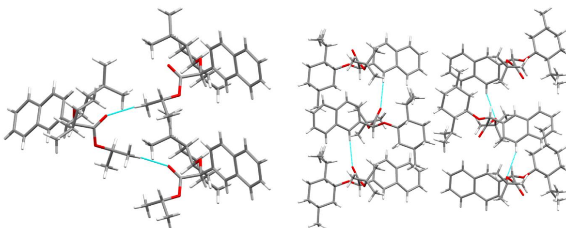
Fig. 3 Weak C-H...O interactions in (2'S)-iPr ( 3a ) crystals viewed down the c -axis, left. H...H close contacts in (2'S)-tBu ( 4a ) viewed down the a -axis, right. The two symmetry independent molecules in 4a have close contacts only with their symmetry equivalent neighbours. This view of 4a , coloured by symmetry equivalence, is in the ESI † . Minor disorder in one molecule of 4a omitted for clarity.
