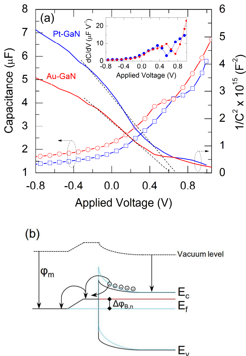
Figure 7. (a) Interface capacitance and Mott-Schottky ( 1/C^2 - V ) profile for Pt and Au catalyzed porous GaN layers. (b) Proposed band structure model for intermetallic interface phase formation acting as the effective ohmic contact. The barrier with (solid line) and without (dashed line) the presence of the intermetallic is shown.
