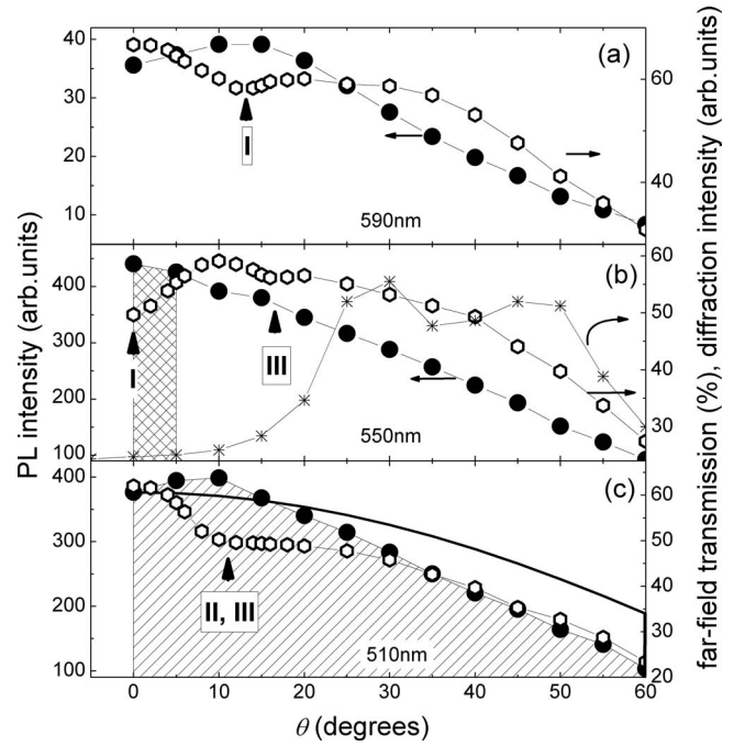
FIG. 6. Angle diagrams of emission intensity (solid circles) at \lambda=590 , 550, and 510 nm in comparison to diagrams of transmission at the same wavelengths (open hexagons). These diagrams are compared to the angle diagram of diffraction intensity at \lambda=550 nm (stars) in panel (b) and the Lambert diagram (line) in panel (c). Shaded areas show the emission power between (b) 0^\circ and 5^\circ — S_{550}^{60} and (c) 0^\circ and 60^\circ — S_{510}^{60} . Arrows mark the angle position of transmission minima. Numbers at arrows indicate the dispersion branch as indicated in Fig. 3(b).
