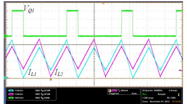
Fig. 10. Experimental waveforms of CCM. The Q1 voltage (green) is 100V/div, while the phase 1 current (blue) and phase 2 current (purple) are 1A/div each [10].
