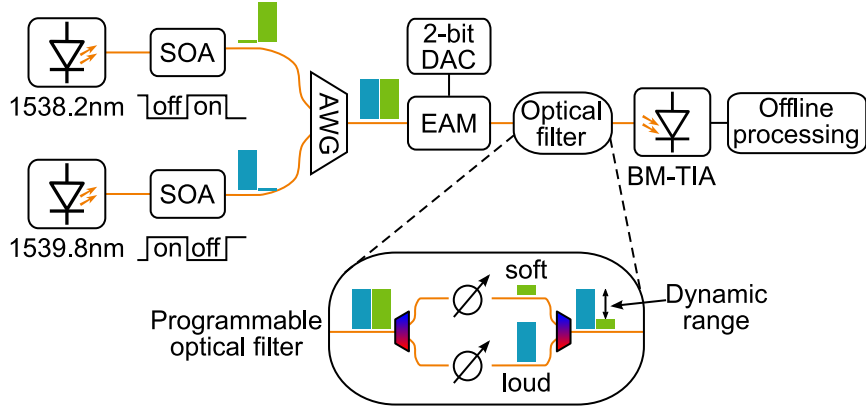
Figure 3.28: Experimental setup for BM-TIA characterisation.
