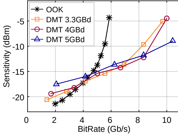
Figure 3.9: Experimental sensitivities in optical B2B for DMT signals at various Baud-rates and NRZ-OOK.
