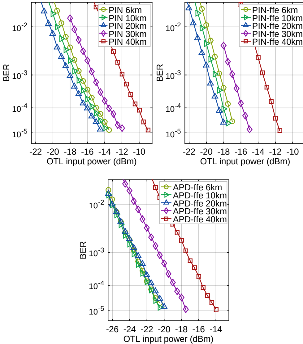
Figure 5.23: BER curves for the 25 Gb/s PAM4 system for various fibre lengths and three receivers type.
