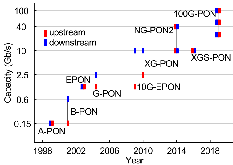
Figure 2.3: Evolution of PON standards capacities in 20 years.
