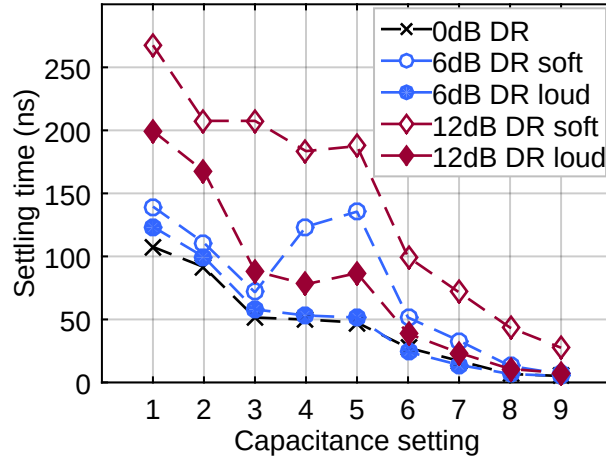
Figure 3.29: Settling time of BM-TIA for different restoration-loop bandwidths.
