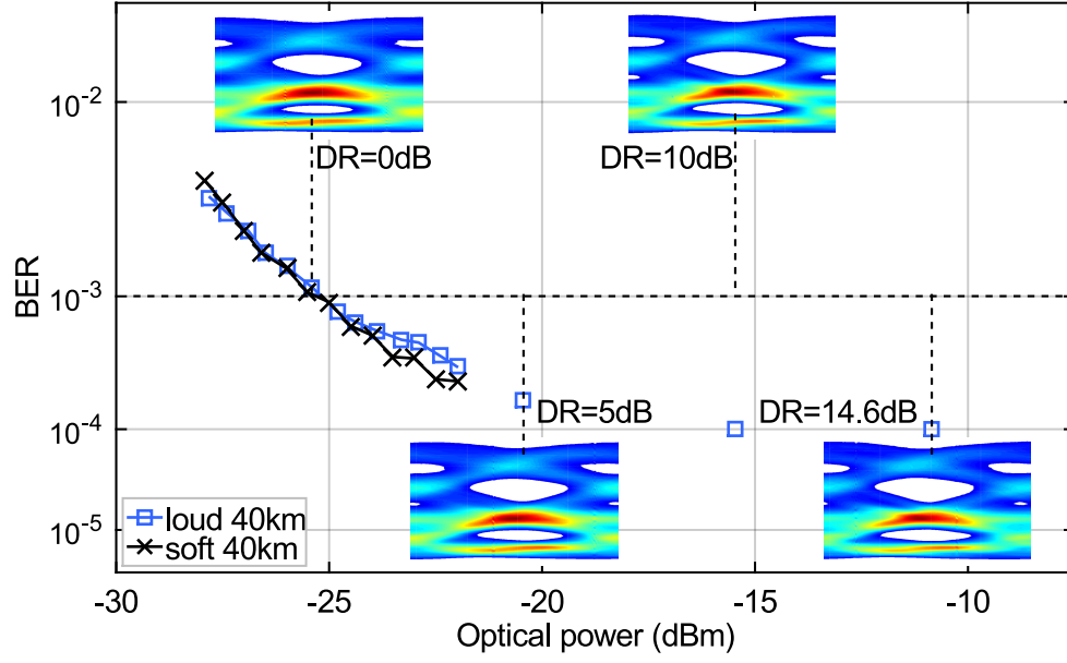
Figure 5.49: BER curves of soft and loud bursts and eye diagrams of the loud burst under different DR conditions for NRZ-EDB with 40 km of SMF.
