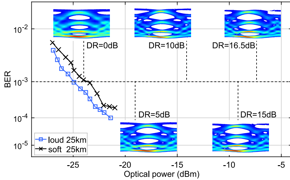
Figure 5.54: BER curves of soft and loud bursts and eye diagrams of the loud burst under different DR conditions for PAM4 with 25 km of SMF.
