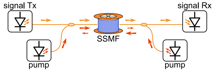
Figure 5.3: Schematic of a Raman optical amplifier.
