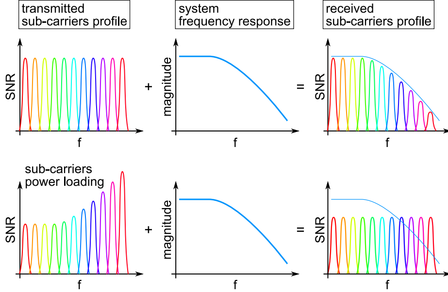
Figure 3.2: DMT sub-carriers SNR profile without and with power loading adjustment at the transmitter.
