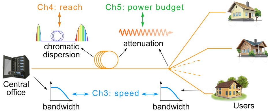
Figure 1.5: Major impairments in PON systems addressed in this thesis.
