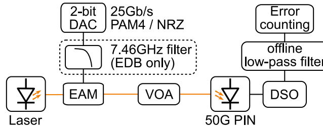
Figure 3.14: Experimental setup for receiver bandwidth requirements measurements.
