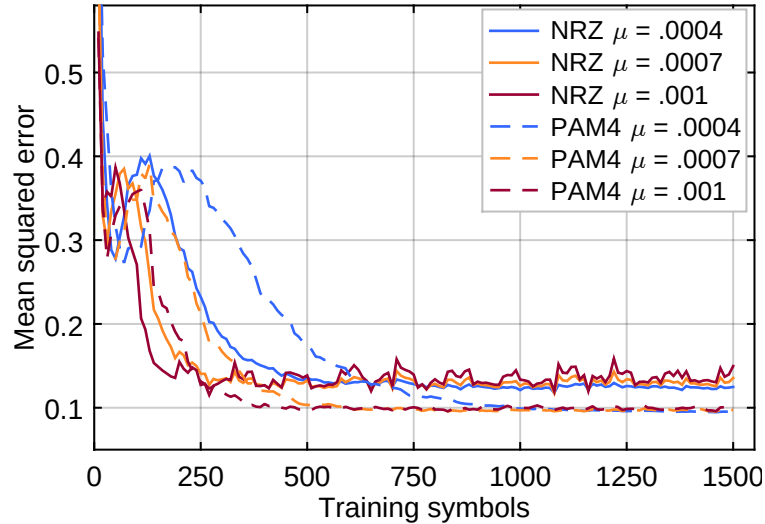
Figure 4.17: MSE measured for various training sequence lengths and LMS gains using binary or multi-level training.
