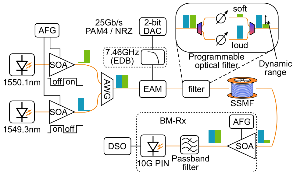
Figure 5.43: Experimental setup for for burst-mode traffic analysis with SOA based pre-amplified receiver performing optical equalisation.
