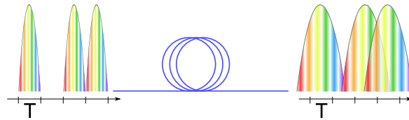
Figure 2.10: Inter-symbol interference caused by pulse spreading over dispersive fibre.
