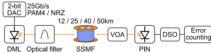
Figure 4.41: Experimental setup for characterisation of CML transmitters.
