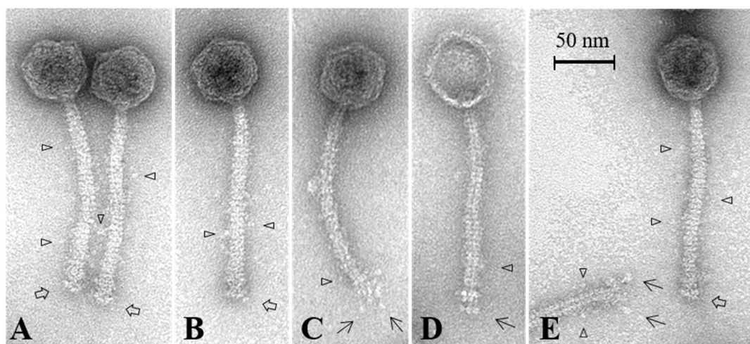
Figure 4. Representative micrographs of Phi4.2. ⇨ highlights the less compact baseplate of the phage. → highlights the elongated protein, thought to be RBP1 Phi4.2 , protruding from the baseplate of the phage (C,D,E). ▷ highlights the globular appendages which appear to coat the tail of the phage (A–E). Phages were stained using 2% uranyl acetate.
