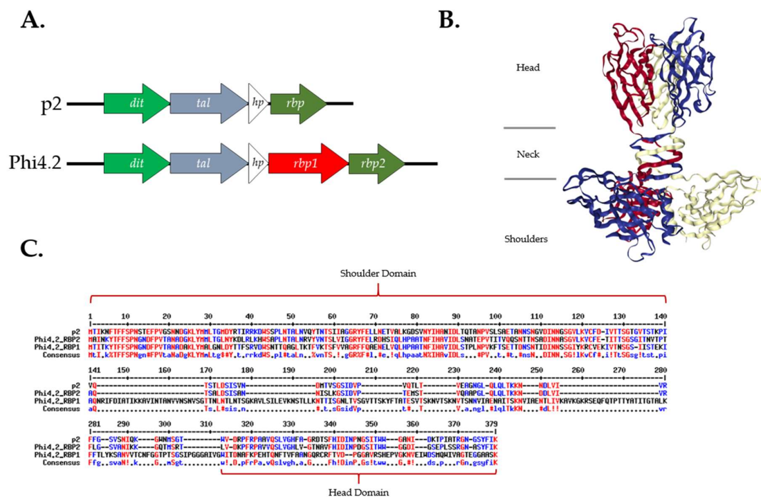
Figure 2. Sequence analysis of the RBPs of Phi4.2 and p2. (A) Genomic architecture of the baseplate regions of p2 and Phi4.2. (B) Ribbon structure of the RBP trimer of p2, as previously determined [14,23], highlighting the “shoulder”, “neck”, and “head” domains. Ribbon structure retrieved from the PDB database (PDB ID: 1ZRU). (C) Alignment of the amino acid sequences of the RBPs of Phi4.2 and p2, highlighting the elongated “neck” domain of RBP1 Phi4.2 . Conserved amino acids are in red, and partially conserved in blue. Alignment created using Multalin [43].
