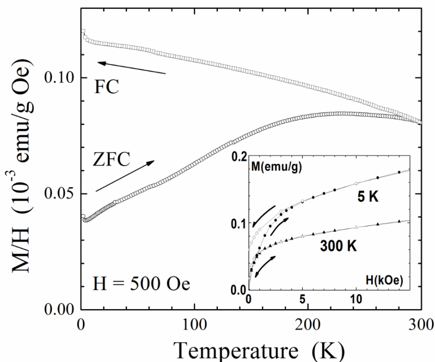
Fig. 12 Temperature (main panel) and field (insert) dependence of the magnetization for the pyrolytic product obtained from a chitosan- (\text{CuCl}_2)_n precursor prepared in a molar ratio of 5:1.
