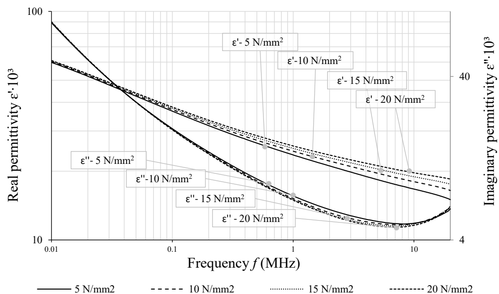
Figure 54. 3F36 ferrite complex permittivity vs. frequency and tension.
