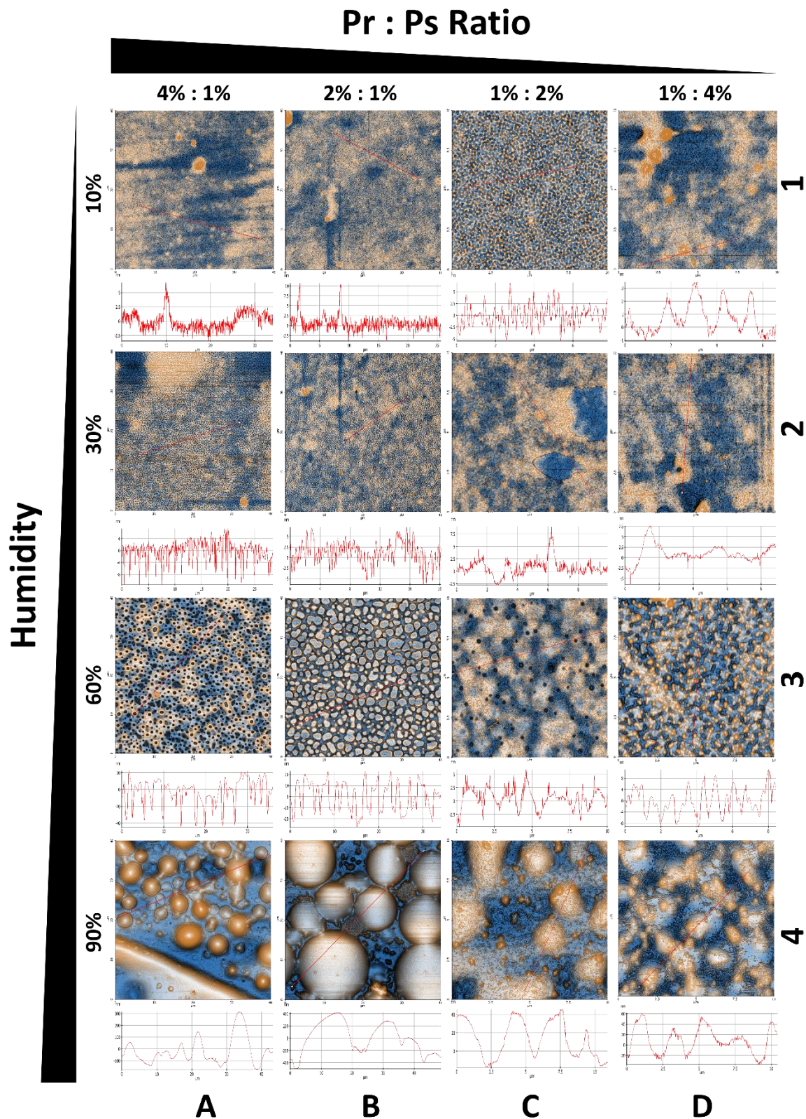
Figure 2.4: AFM image grid and associated line profiles showing results of casting thin-films at 12 \mu m from specific Pr-Ps-S solutions of PG-Ch-FA at specific humidities. Each image in column A and column B is 40 \mu m \times 40 \mu m area. Each image in column C and column D is 10 \mu m \times 10 \mu m area. Column A = 4 w/v% PG 1 w/v% Ch (4:1), column B = 2 w/v% PG 1
