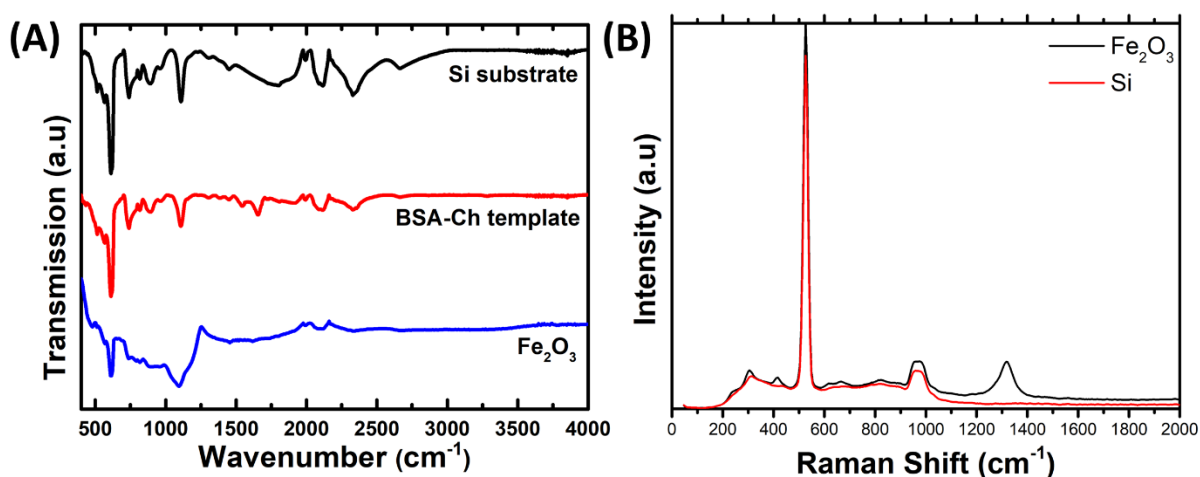
Figure S4.6: (A) FTIR spectra of Si substrate, biopolymer template and Fe 2 O 3 porous matrix after annealing and calcination. (B) Raman spectra of Si substrate and Fe 2 O 3 porous matrix after annealing and calcination.
