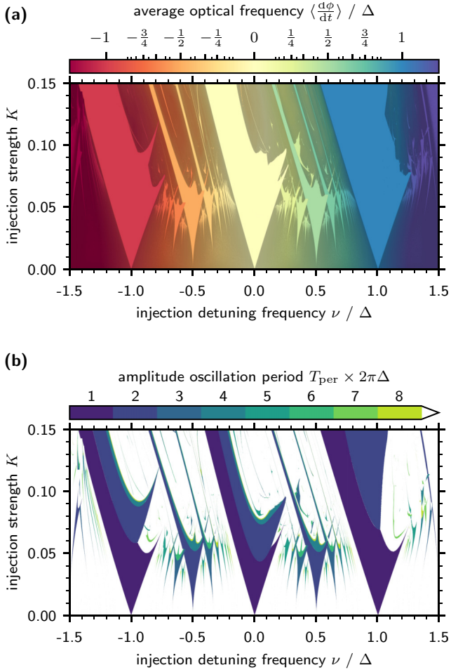
FIG. 4. Two-dimensional resonance diagrams for the semiconductor laser model, showing (a) the average optical frequency \langle \nu_{\text{opt}} \rangle and (b) the period T_{\text{per}} of the intensity oscillations, depending on the injection strength K and the laser detuning \nu from the center comb line with respect to the free-running secondary laser frequency (cf. Fig. 2). Simulated without spontaneous emission noise, \beta = 0 . All frequencies are normalized to the comb spacing \Delta .
