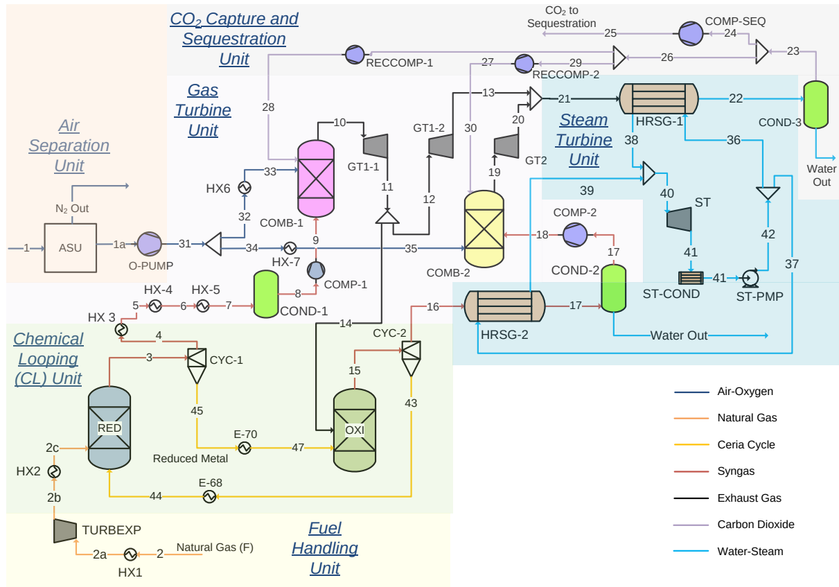
Figure 12. Process layout of oxy-fired power plant OXY-CC-CL[55]
