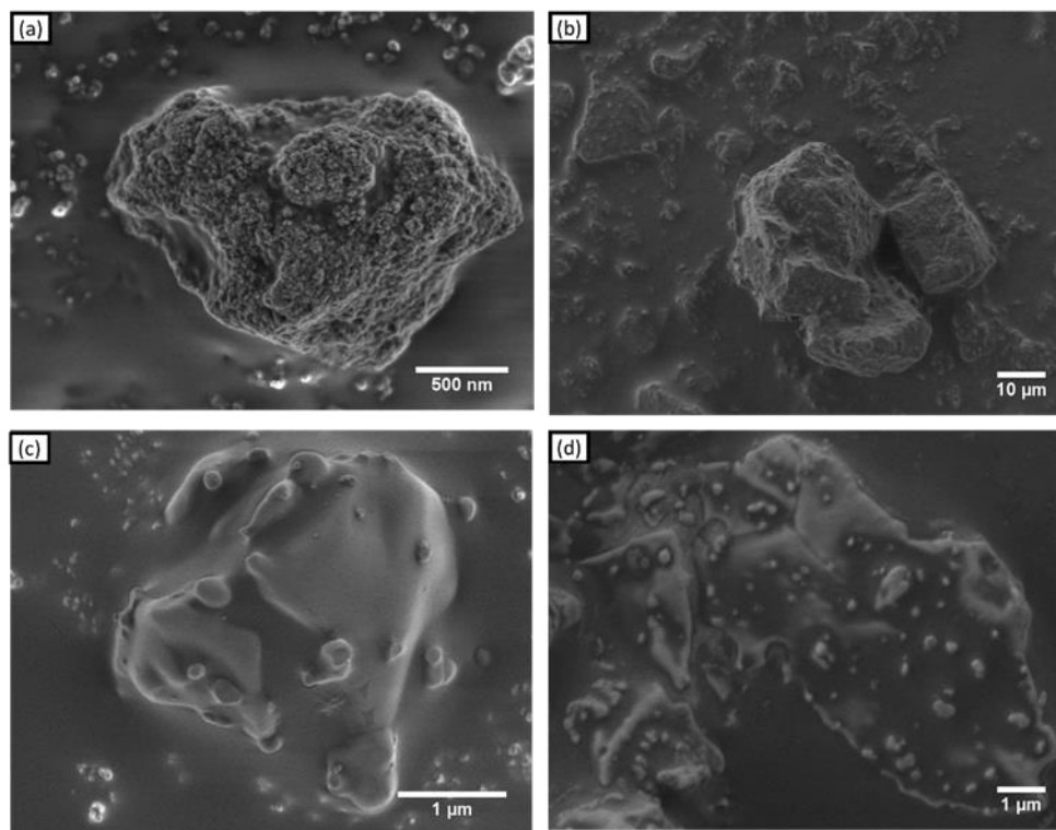
Figure 7 Phases, and compositions in the samples of ceria (a) 900°C (b) 1000°C (c) 1100°C at 30% CH 4 (d) 1000°C at 30% CH 4
