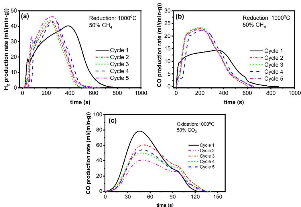
Figure 3 (a) H_2 and (b) CO production rate from the reduction of CeO_2 over 50% CH_4 and (c) oxidation of the reduced metal oxide with 50% CO_2 over five cycles each.
