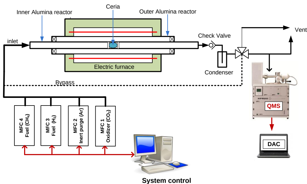
Figure 2. Experimental set-up for testing in micro-reactor configuration
