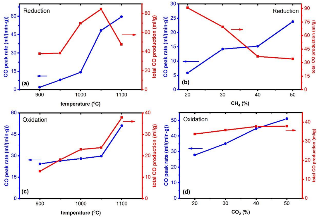
Figure 6 CO peak rate and total CO production for varying temperatures and feed concentrations with CH 4 of 30% and CO 2 of 50% during reduction and oxidation respectively and 1100°C during oxidation.
