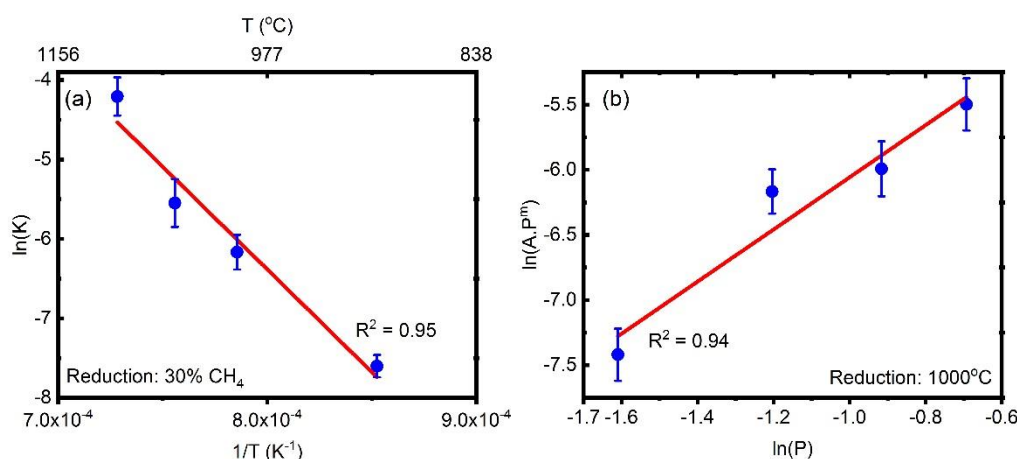
Figure 8 (a) \ln(K) vs (1/T) Arrhenius plot of the reduction reaction for AE3 model; (b) \ln(AP^m) vs \ln(P) plot for reduction reaction order determination.
