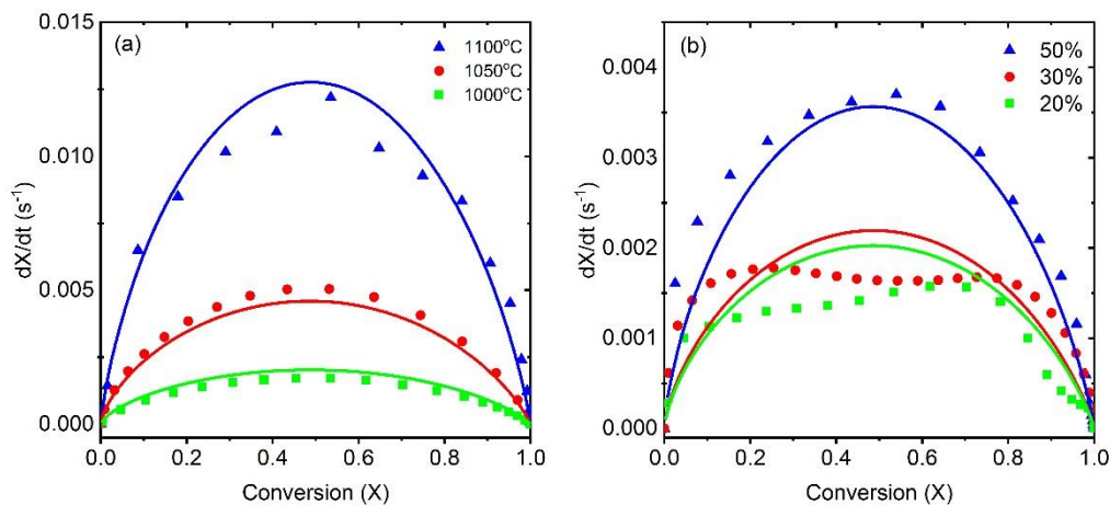
Figure 9 Comparison of the kinetic model and the experimental data for methane reduction of ceria (a) with the variation in temperature, 1000°C, 1050°C, 1100°C and (b) with the concentration of CH 4 of 20%, 30% and 50% for reactor pressure of 1 atm. The symbol represents experimental data and lines represent the kinetic model
