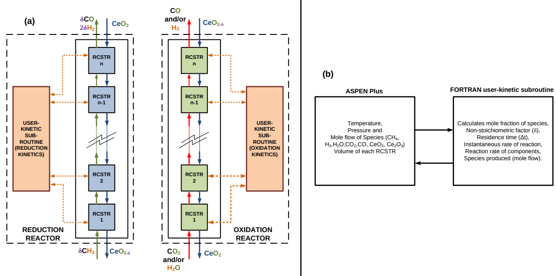
Figure 13 Moving bed reactor model for methane reduction and \text{CO}_2/\text{H}_2\text{O} oxidation reactors in ASPEN Plus hooked with user kinetics written in an external FORTRAN Code
