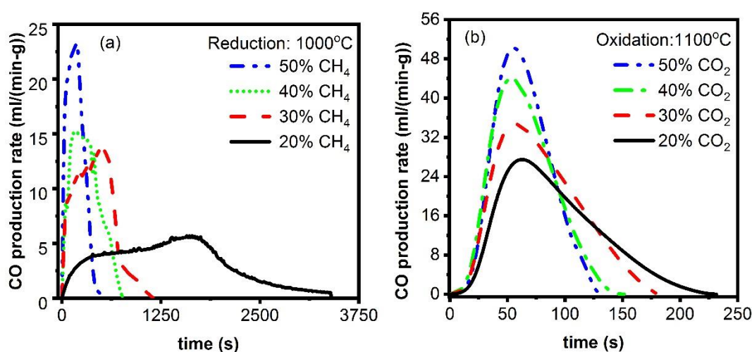
Figure 5 Variation of yield rates of CO in (a) methane reduction of ceria at 1000°C and (b) oxidation of reduced ceria at 1100°C with the variation of concentration of the gaseous reactants at a reactor pressure of 1 atm
