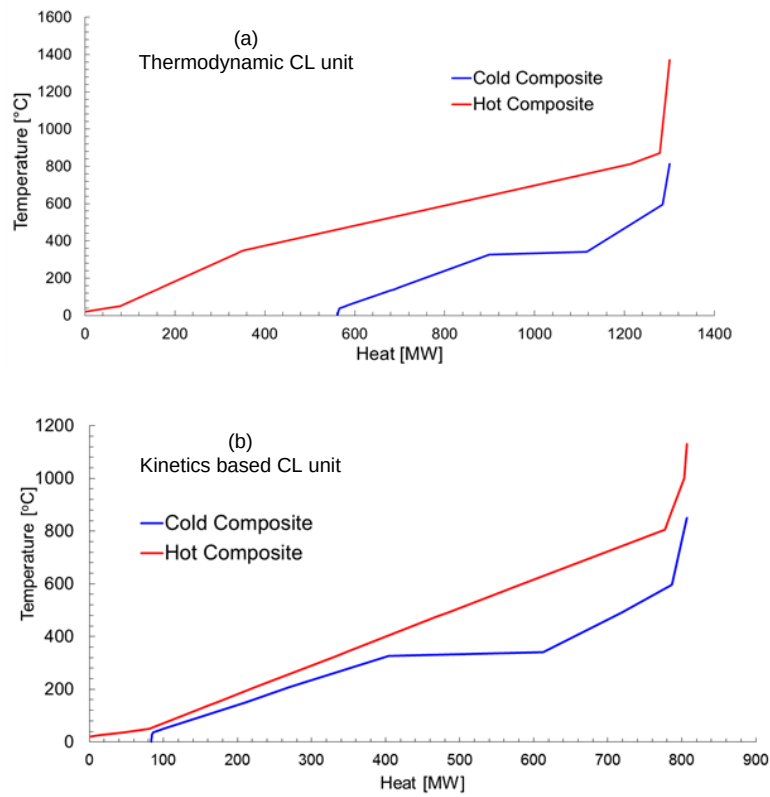
Figure 14 Pinch Analysis of the proposed plant based on (a) thermodynamics model OXY-CC-CL unit and (b) kinetics-based moving bed CL unit (OXY-CC-CL-K)
