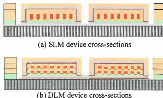
Figure 1 Schematic of SLM & DLM device cross-sections
