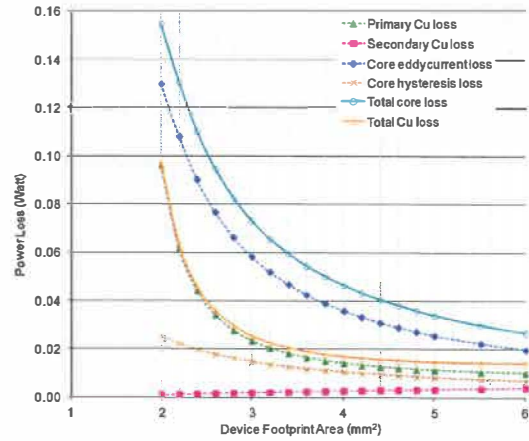
Figure 3. Loss breakdown of SLM designs using 30μm conductors
