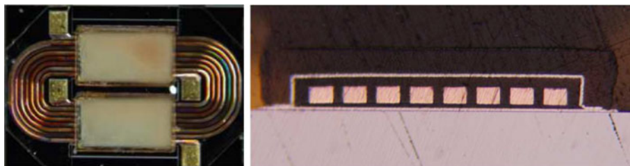
Fig. 5. Plan view and cross-section of single-layer metal (SLM) micro-magnetic process – overall device footprint 3 \times 2 \text{ mm} .
