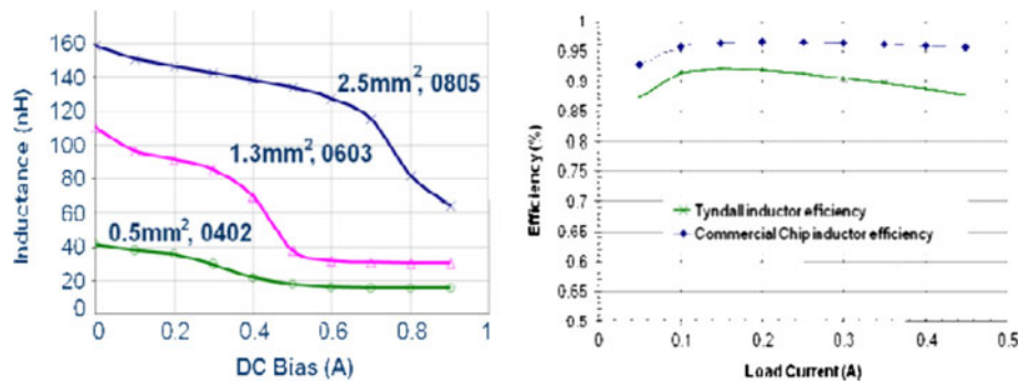
Fig. 9. Micro-inductors – measured inductance versus bias current and extracted inductor efficiency for 8 MHz buck converter circuit. Comparison with commercial wire-wound chip inductor.
