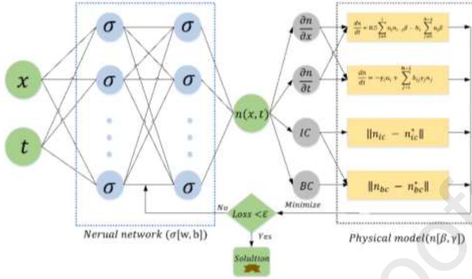
Figure 1. Diagram of a population balance neural network (PBNN) model for solving the forward and inverse problems of particle aggregation and breakage systems.
