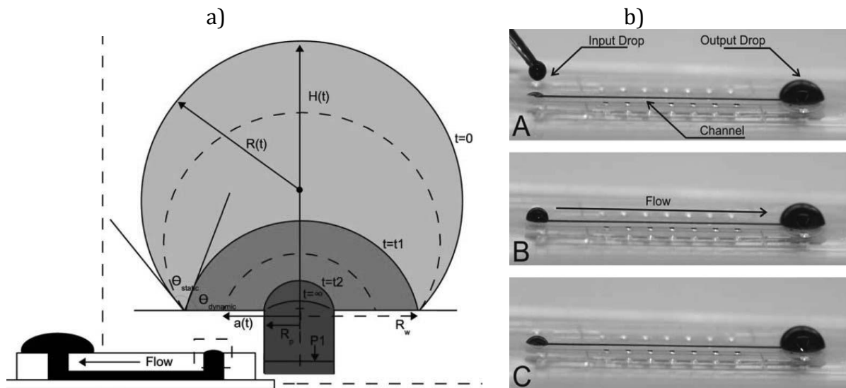
Figure 1.14: a) A schematic of a drop of liquid placed onto a fluidic inlet. b) A practical example of surface tension driven flow. The flow occurs from the small volume drop into the bigger volume drop (Berthier and Beebe, 2007).
