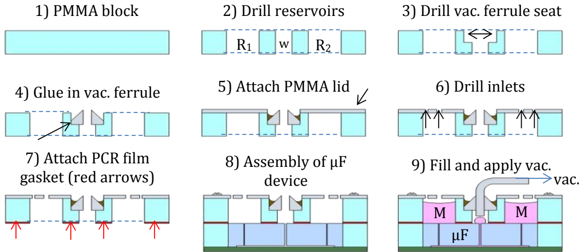
Figure 5.3: Schematic representing fabrication of \mu F reservoir plate and its integration with PDMS \mu F device. 1) A 5mm thick PMMA block is cut to size. 2) The media reservoirs (R1 and R2) and waste outlet (w) drilled out. 3) The waste outlet is widened and 4) the vacuum coupler is glued in using epoxy. 5) A 1mm thick PMMA cover is attached to the reservoir plate using transfer tape. 6) Small inlets are drilled in PMMA cover (2 per reservoir). 7) PCR film is attached to the bottom of the reservoir plate to serve as a gasket (red arrows). 8) The reservoir plate is attached to the PMMA ring on the substrate surface housing the PDMS \mu F device. Screws are used to hold the assembly together. 9) The reservoirs are then filled with cell culture media (M), the waste outlet is connected to a vacuum source (peristaltic or syringe pump) and the media is drawn from the reservoirs into the \mu F device and out to waste outlet.
