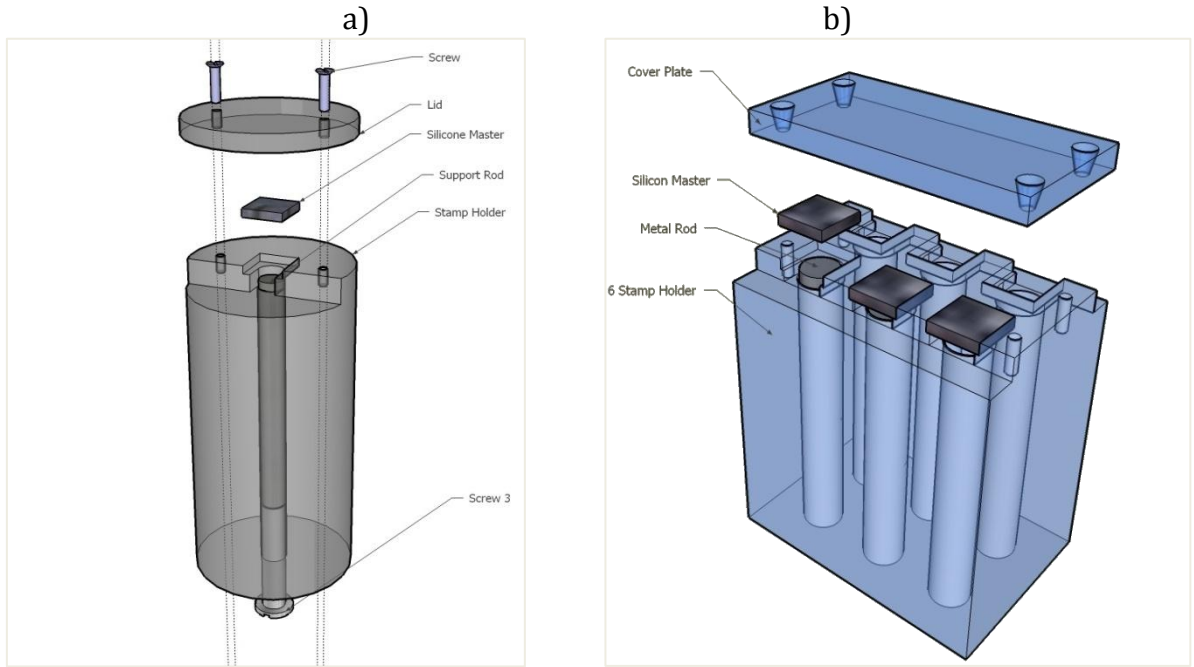
Figure 2.6: The parts used to cast the PDMS against the master to produce a micro-stamp. a) The old, single stamp casting holder as described in (Lauer et al., 2001). b) The newer 6 stamp casting holder. This machined device significantly reduced the amount of time required for making multiple micro-stamps. (Note: Silicon masters are 5 mm 2 x 1 mm).
