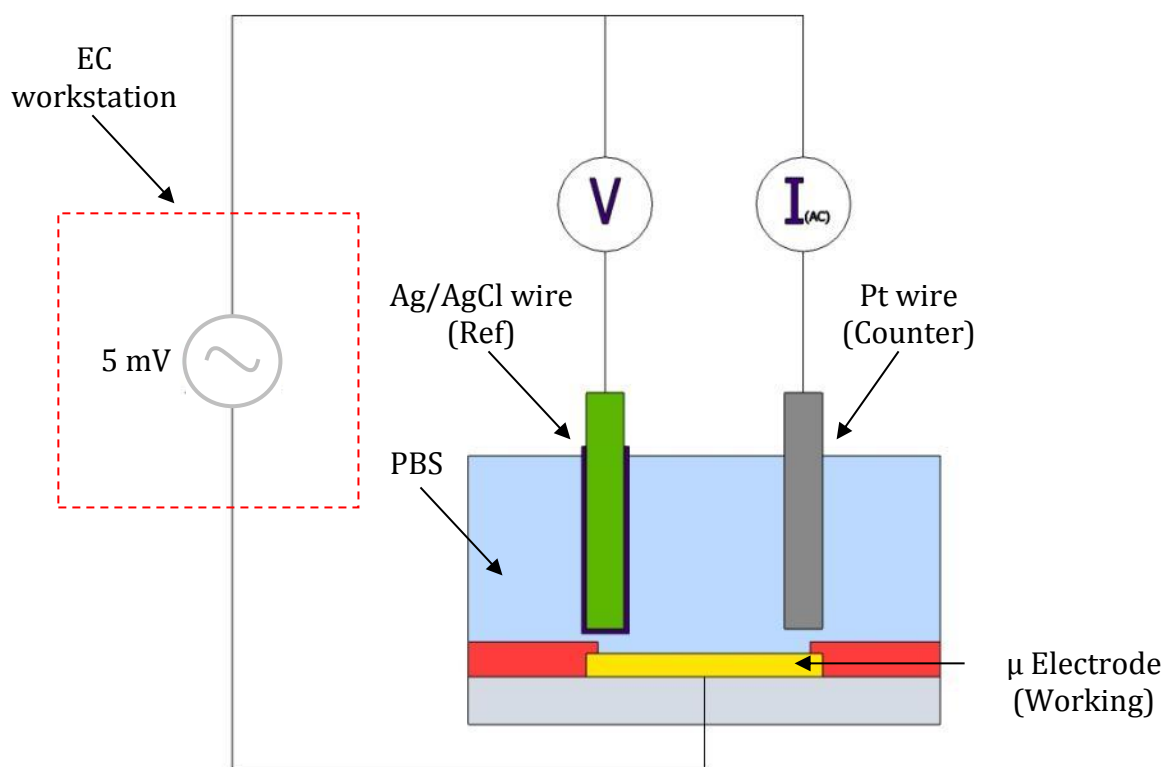
Figure 4.2: A schematic summarizing the EIS setup. The current is supplied to the system using an electrochemical work station. The counter electrode was a platinum wire, while the reference electrode was Ag/AgCl. The working electrode was the microelectrode of interest on the surface of MEA.
