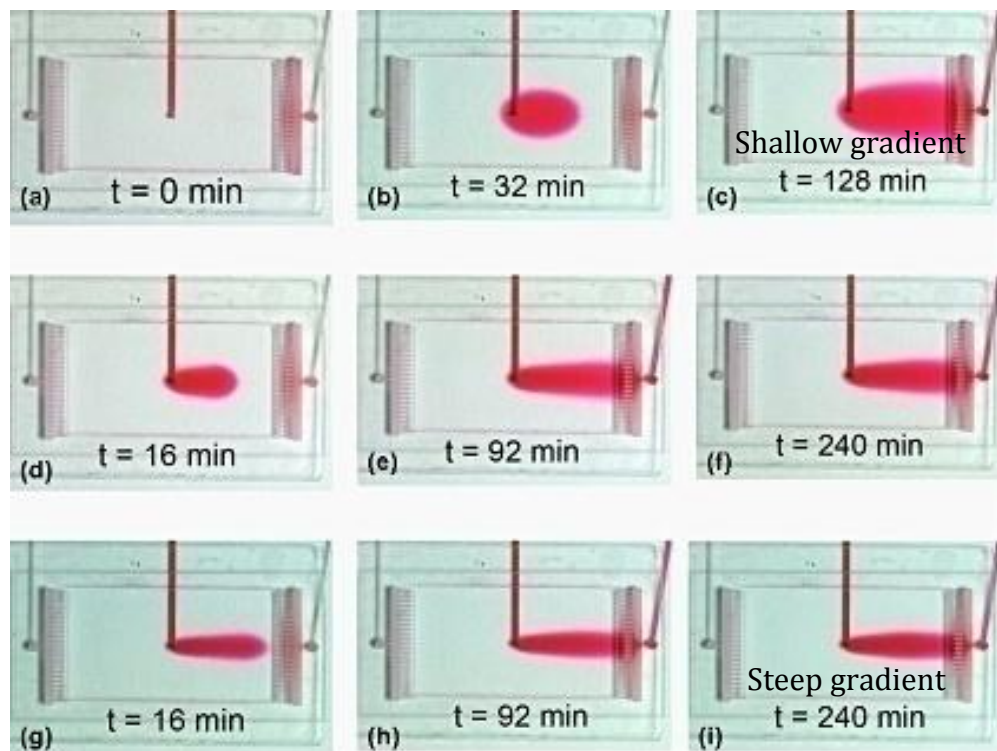
Figure 1.12: Generation of microfluidic gradients of varying slope using variation on flow velocity. (a-c): Bulk media flow at 10\mu\text{L/h} , dye supply through the effusion inlet is also at 10\mu\text{L/h} . (d-f): Bulk media flow at 30\mu\text{L/h} . (g-i): Bulk media flow at 50\mu\text{L/h} (Cheng et al., 2008).
