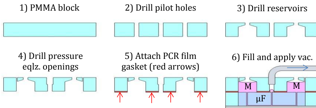
Figure 5.4: Schematic representing simplified fabrication of \mu F reservoir plate and its integration with PDMS \mu F device. This method of fabrication greatly reduces the number of steps and components required.
