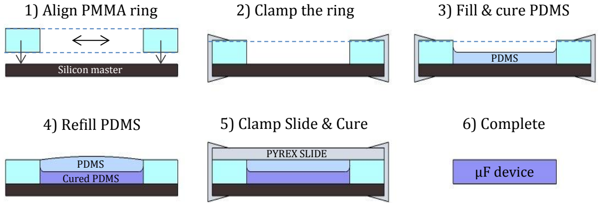
Figure 2.9: The schematic representing the basic steps involved in fabrication of flat \mu F devices. The fabrication involves two stages. Stage #1 is represented by steps 1-3. Stage #2 is represented by steps 4-6.
