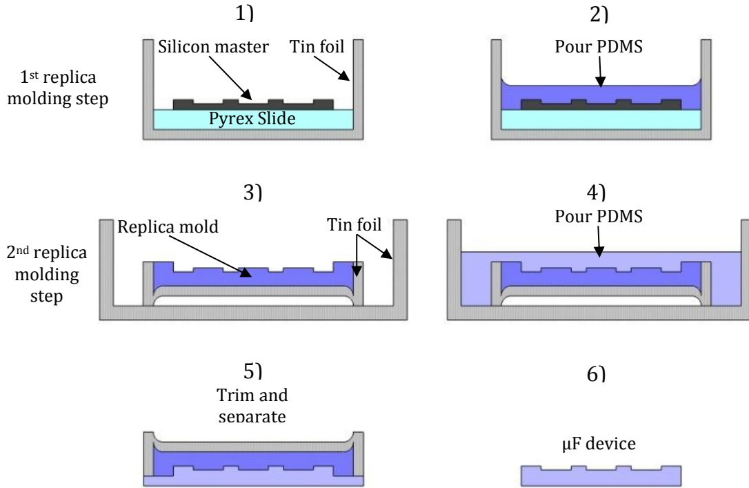
Figure 2.10: Basic schematic of fabrication of the \mu F devices using PDMS masters. 1) A silicon master was placed onto a Pyrex slide partially wrapped with tin foil. 2) 1 st replica molding step. 3) A cured replica mold wrapped in tin foil. 4) The second replica molding step. 5) After PDMS is cured, the excess is trimmed using a razor blade and the mold is separated. 6) The fabricated \mu F device, a direct copy of silicon master.
