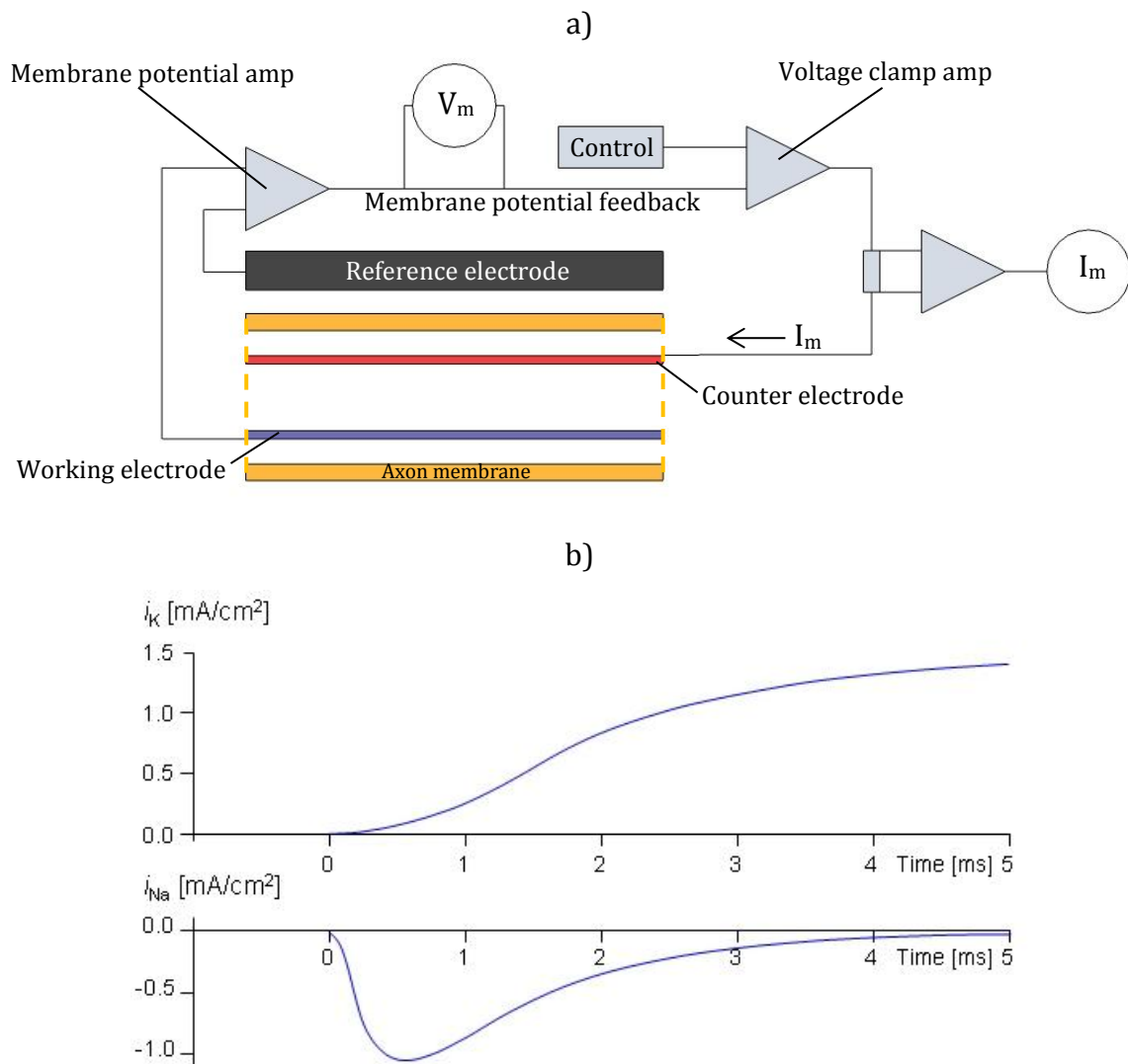
Figure 1.5: a) Schematic representation of voltage clamp experiment. b) Idealised voltage clamp recordings of sodium and potassium ion movement (Malmivuo and Plonsey, 1995).
