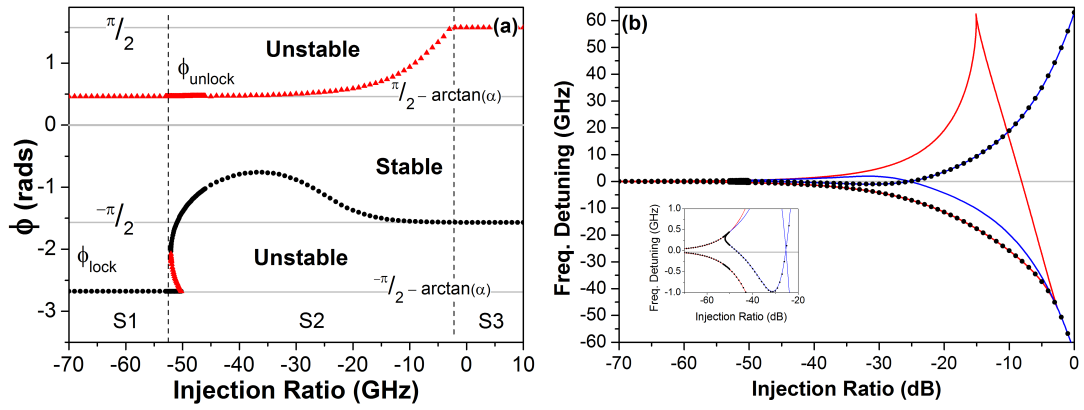
Figure 3.11: (a) Phase limits and (b) frequency limits for the stable locking region when \alpha = 2 .
