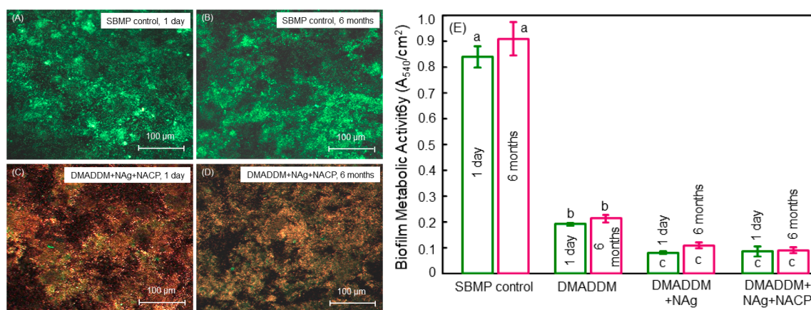
Figure 4. Anti-biofilm bonding resin after water-aging for 6 months. (A,B) Typical confocal laser scanning microscopy live/dead images for SBMP control; (C,D) DMADD + Nag + NACP, at one day and six months, respectively. DMADD and DMADD + NACP groups had features similar to (C,D) (not shown). The novel bioactive bonding agent had primarily compromised bacteria. SBMP control had mostly live bacteria. (E) Metabolic activity (mean \pm SD; n = 6 ). The potent antibacterial function remained after water-aging for six months. Adapted from Ref. [56], with permission from © 2013 Elsevier.
