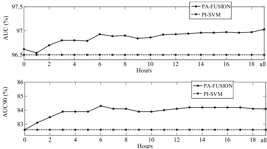
FIGURE 5. Performance of the baseline SVM and adaptive fusion system measured as AUC (top) and AUC90 (bottom) as a function of time.
