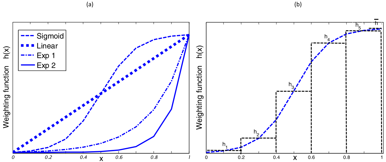
FIGURE 3. (a) Four different weight functions; here x = PSVM for providing weights for updates to seizure class GMM, x = (1-\text{PSVM}) for updating non-seizure class GMM. (b) An example of a sampled sigmoid weighting using 5 clusters.
