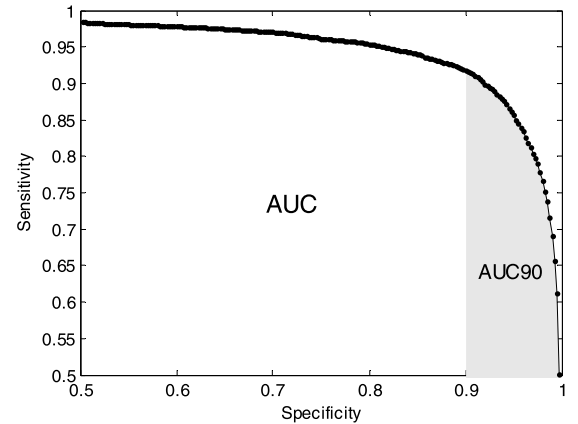
FIGURE 4. Performance of a SDA - measured as the area under the ROC curve.
