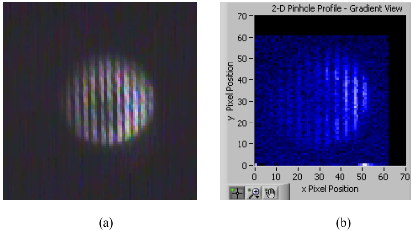
Figure 13. Optical irradiance 2-D mapping of a non-uniform irradiance distribution using the Fig.11 sensor. The pattern is a 1-D grating produced using spatial modulation of a laser beam. (a) The irradiance pattern seen by a CCD. (b) The irradiance pattern mapped by the proposed Fig.11 sensor.
