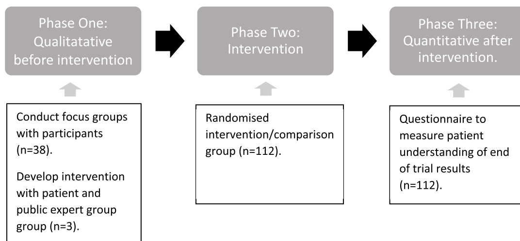
Fig. 1. Study Design.
