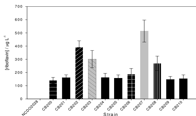
Figure 1 Riboflavin produced by roseoflavin-resistant Lc. mesenteroides NCDO2028 mutants. The riboflavin concentration was determined in the cell free supernatant as the cells entered stationary phase. The various patterns indicate different mutations.
