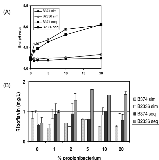
Figure 8 (A) Final pH of yoghurt with various inoculum levels of P. freudenreichii B374 or B2336 either added 24 hours before-hand or simultaneously with the yoghurt starter culture. (B) Final riboflavin levels in yoghurt with various inoculum levels of P. freudenreichii B374 or B2336 either added sequentially or simultaneously with the yoghurt starter culture.
