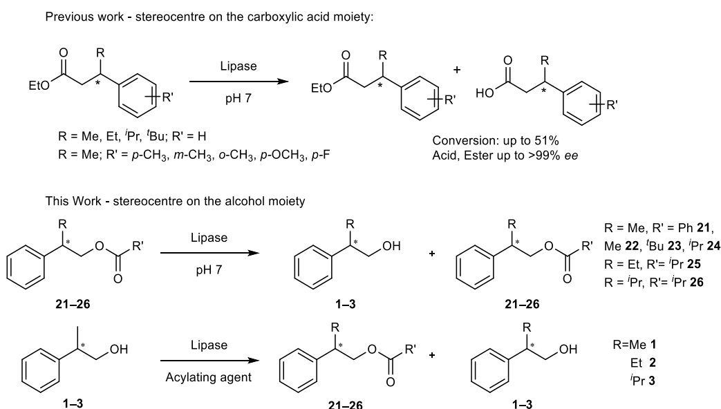
Scheme 2.8 Hydrolysis and transesterification of chiral primary alcohols and esters
