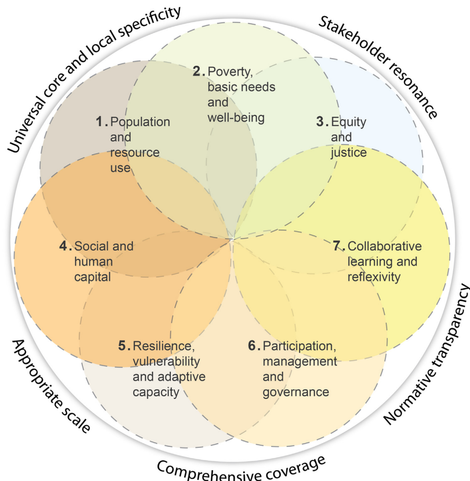
Fig. 3. Social-ecological dynamics of coastal ecosystems: a conceptual framework.
