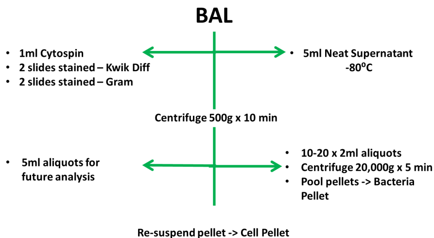
Figure 3. Patient BAL processing schematic BAL processing began in the laboratory on the day of bronchoscopy.
