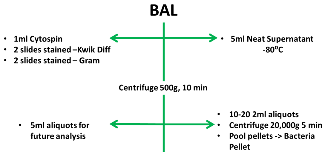
Figure 1 Patient BAL processing. Schematic depicting the processing undertaken with the patient BAL once received in the laboratory on the day of bronchoscopy.
