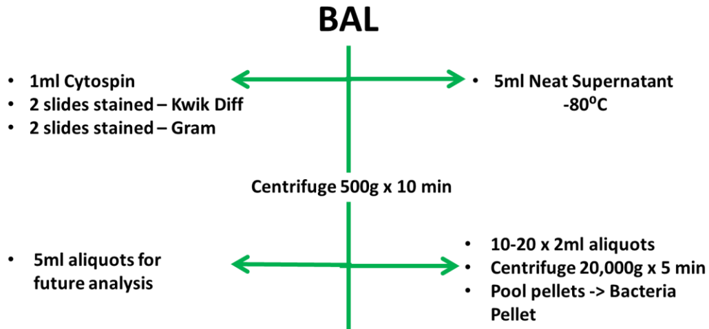
Figure 1. Patient BAL processing schematic. Chart depicting the process the patient BAL underwent once processing began in the laboratory on the day of bronchoscopy.
