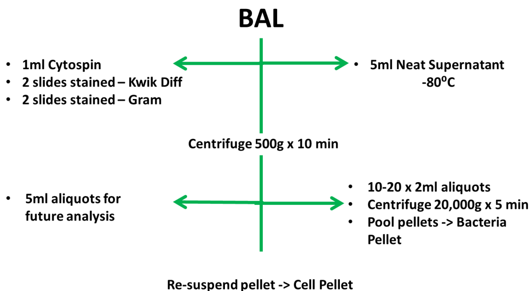
Figure 2. BAL sampling schematic. The processing steps undertaken with the patient BAL once received in the laboratory on day of bronchoscopy.
