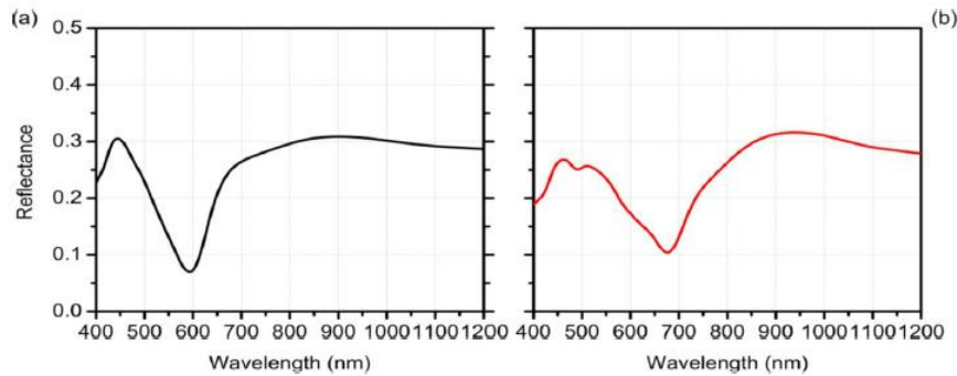
Figure S4. Simulated specular reflectance results for a 40 degree TE polarized incident light. Simulated specular reflectance of: (a) non-tapered GaAs-AlGaAs C-S NWs with the same core radius and half of the radius of the shell of sample B1, and (b) tapered GaAs-AlGaAs C-S NWs with the same core radius and half of the radius of the shell of sample B2.
