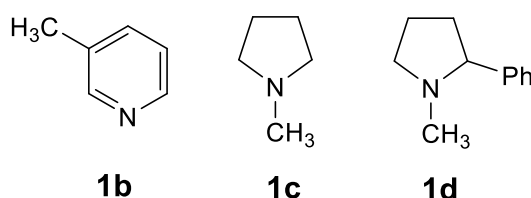
Scheme 2. Structural analogues of nicotine.
