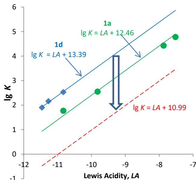
Figure 3. Moving the correlation line for 1d down by 2.4 \lg K units gives a good estimate for the Lewis basicity of the pyrrolidinyl nitrogen of 1a . The estimated correlation line is indicated by the dashed red line.
