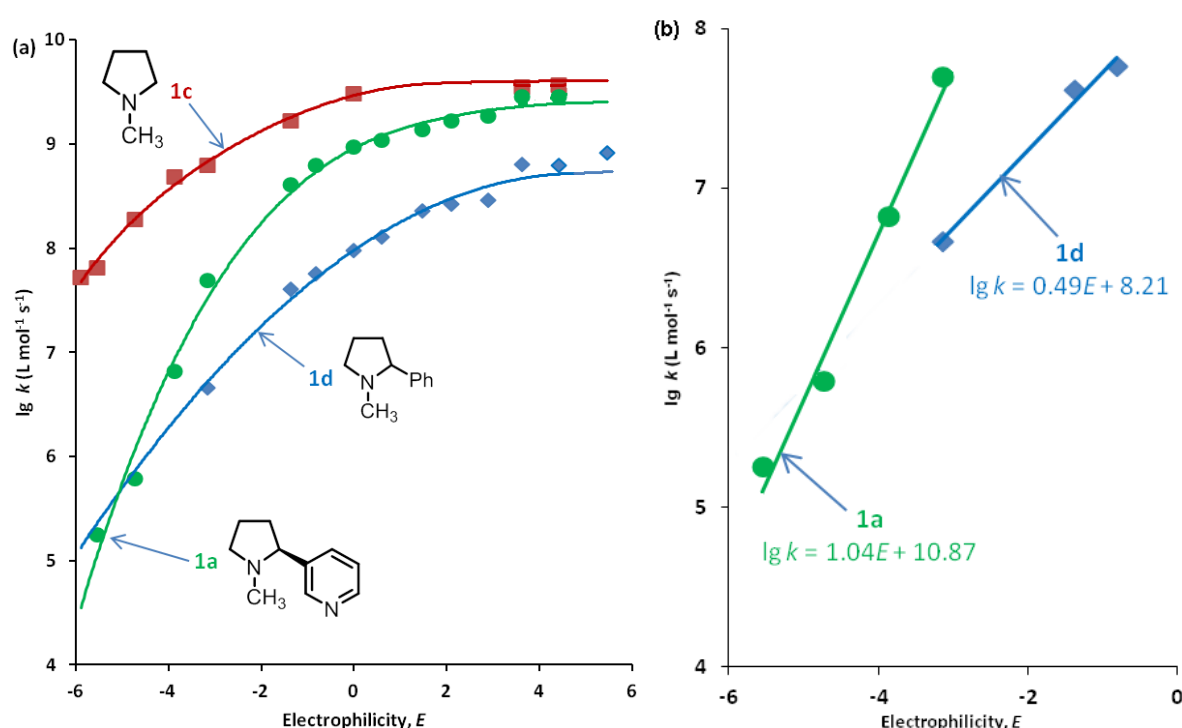
Figure 1. (a) Plot of \lg k (second-order rate constants; \text{L mol}^{-1} \text{s}^{-1} ) for the reactions of nicotine ( 1a ) and structurally related compounds 1(c,d) with benzhydrylium ions 2 versus the electrophilicity parameters E ( \text{CH}_2\text{Cl}_2 , 20 °C) of 2 ; (b) Close-up on the linear parts of Figure 1a, which were used to determine approximate values of N and s N for 1a & 1d (see Table 2). 15 The plot for 1b is almost coincident with that of 1a , and is omitted for clarity.
