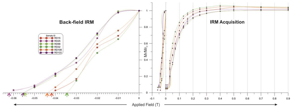
Fig. 8.16 Results of IRM acquisition and back-field IRM demagnetisation. All samples show a narrow spectrum of responses and most are essentially saturated in fields below 0.3T. RD25 and RD122 are significantly H_{CR} & M_s values
