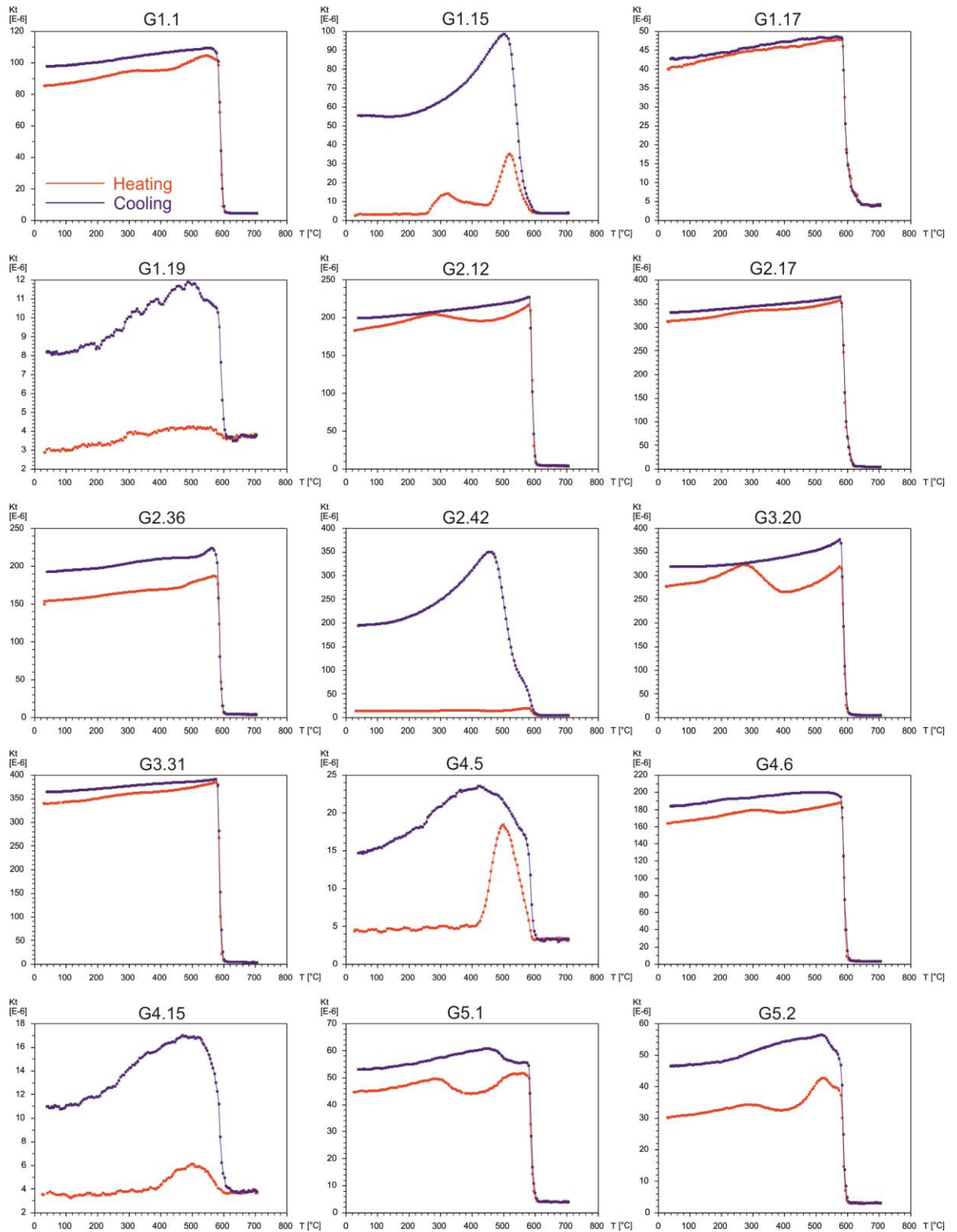
Fig. 9.9 Graphed data from high temperature low field susceptibility experiments, blue = cooling, red = heating. Note several samples exhibit distinct "bumps" at 300°C which are not present on the corresponding cooling curves.
