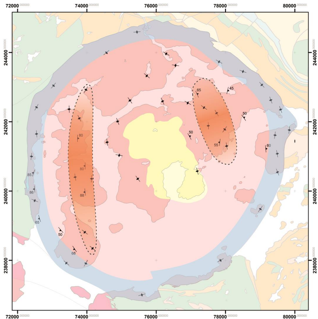
Fig. 8.10 Summary map of the distribution and orientation of fabrics observed in the field. The degree of fabric anisotropy increase towards the pluton contact, an overall concentric ballooning foliation is observed (blue). Fabric intensity decreases toward the centre of the pluton, fabrics are extremely rare in the core and north and south of the intrusion. Two zones of anomalous foliations are observed in the east and west of the pluton 3km from the pluton margin (red).
