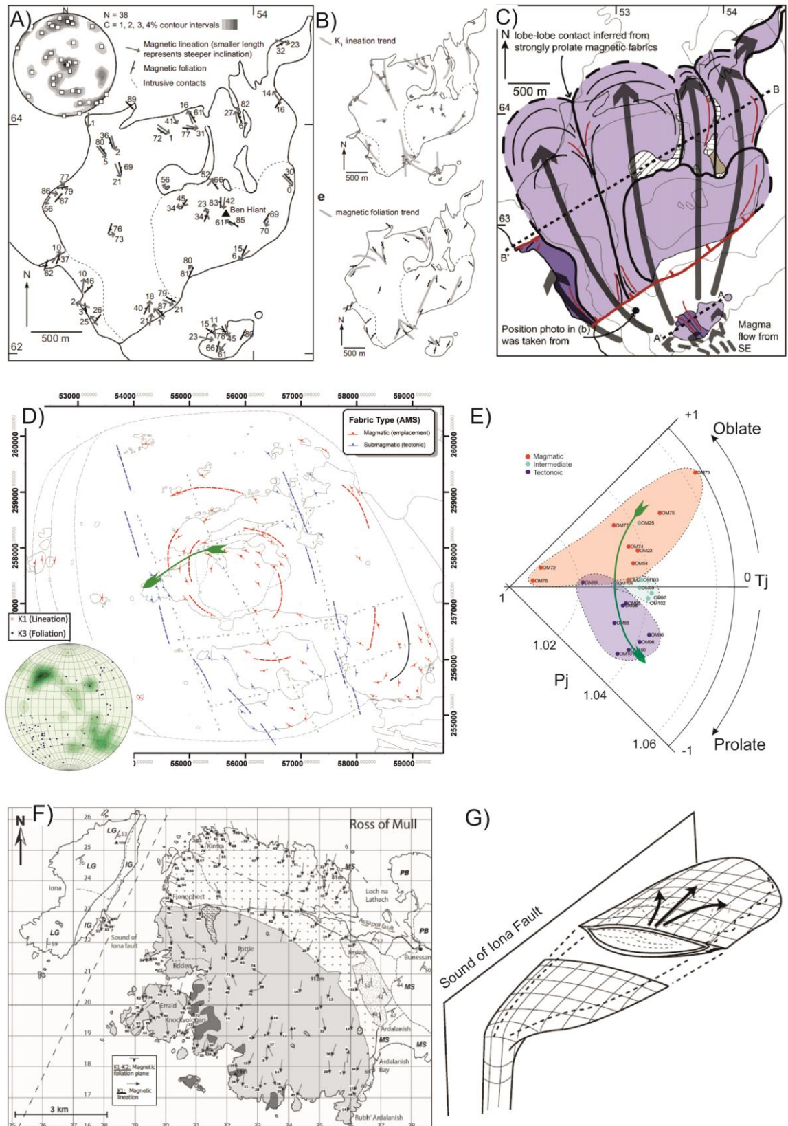
Fig. 10.8 Magee et al. (2012) interpreted AMS tensors from the Ben Hiant Dolerite as magmatic flow indicators (A-C) however the results of the current work show that extremely similar data (note similarities in stereographic projections) actually reflects both pluton inflation and tectonic shearing along NNW-SSE trans-plutonic faults in the Omev Pluton (D-E). Petronis et al. (2012) considered the AMS tensor to be a product of both tectonic and magmatic processes.
