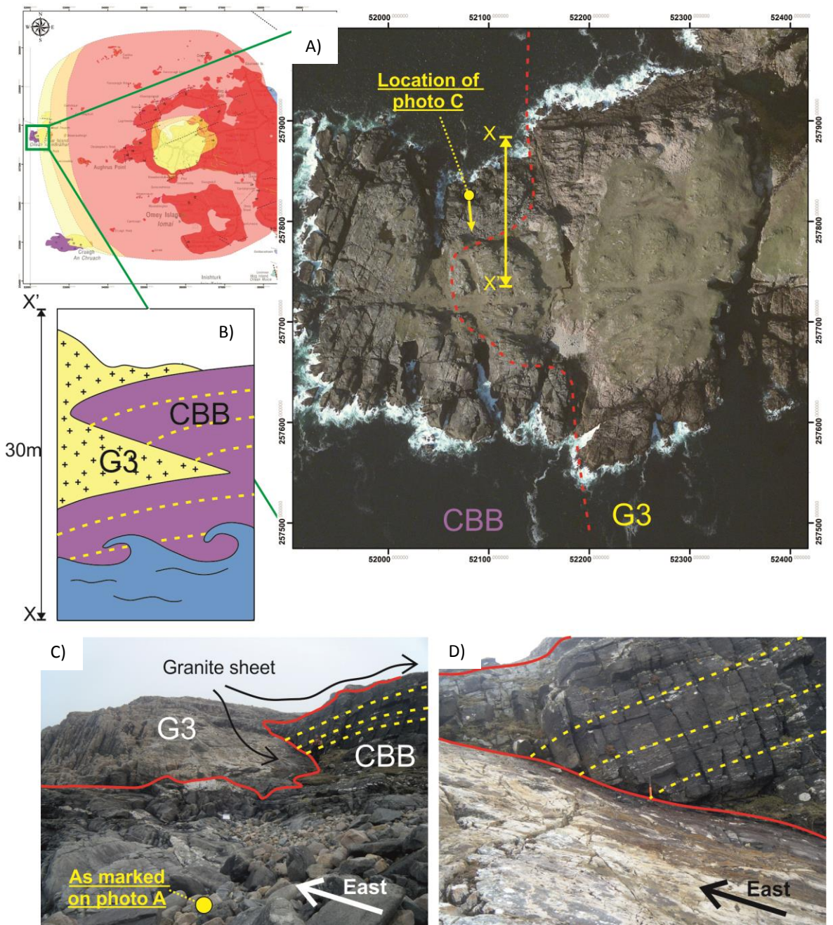
Fig. 7.9 Pluton contact relationships on Friar Isl. A) The eastern and central part of the island is dominantly composed of G3 that sheets into and over the gently dipping ( 10^{\circ} - 20^{\circ} E) bedded strata of the Cleggan Boulder Bed Fm. in the west. B) A schematic section, (looking south) from sea level (X) to the topographic high point on the island (X'), shows that the granite intruded concordant to bedding but also cross cuts bedding along joint planes. This relationship is illustrated in (C) and (D) where the granite has cross cut bedding along a large joint but also sheets parallel to bedding on the cliff top.
