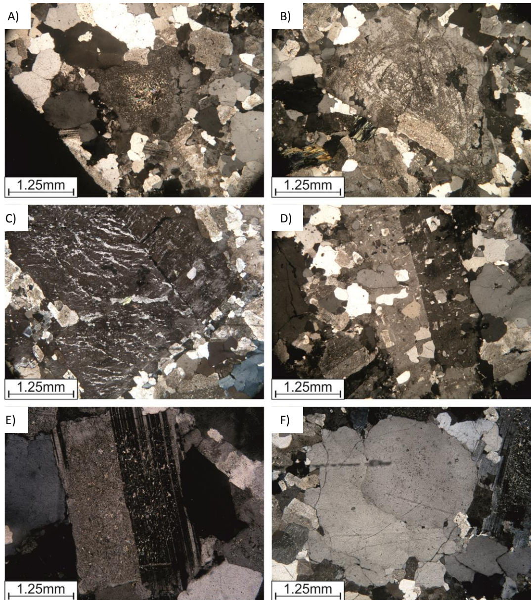
Fig. 7.4 Characteristic petrographic features of G3. Sericitization of plagioclase and orthoclase is concentrated along calcic rich cores or spiked concentric rims (A, B). Porphyritic texture defined by \leq 15\text{mm} tabular plagioclase and orthoclase (A-E) and \leq 12\text{mm} studs of anhedral or rounded quartz (F).
