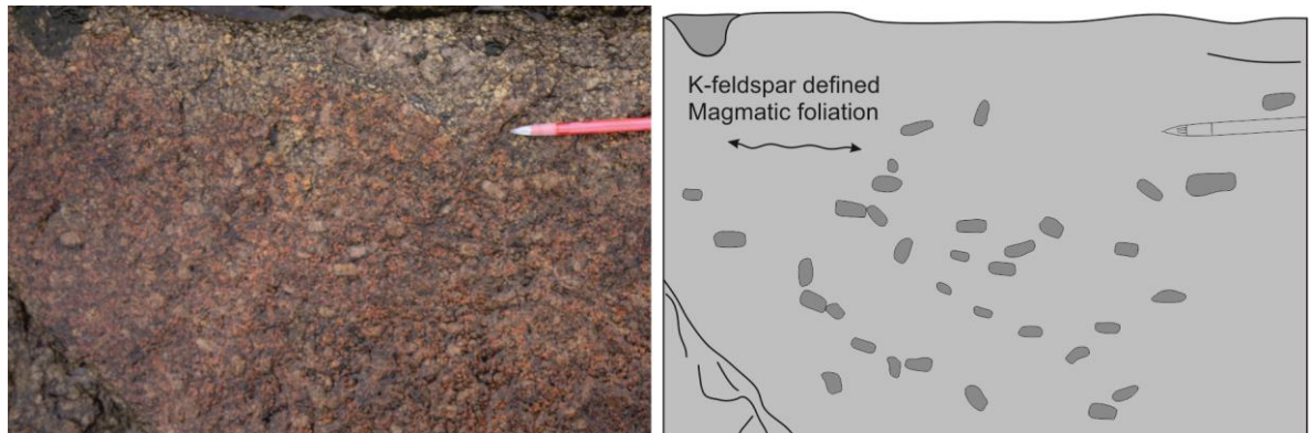
Fig. 9.3 Concentric foliation formed in the magmatic state defined by aligned tabular K-feldspar (North of Gorteen).
