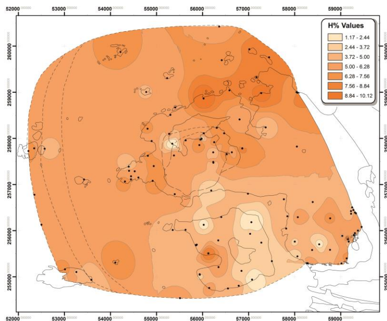
Fig. 7.26 A contour map of determined H values. No definite pattern is observed which can be correlated with facies distribution.
