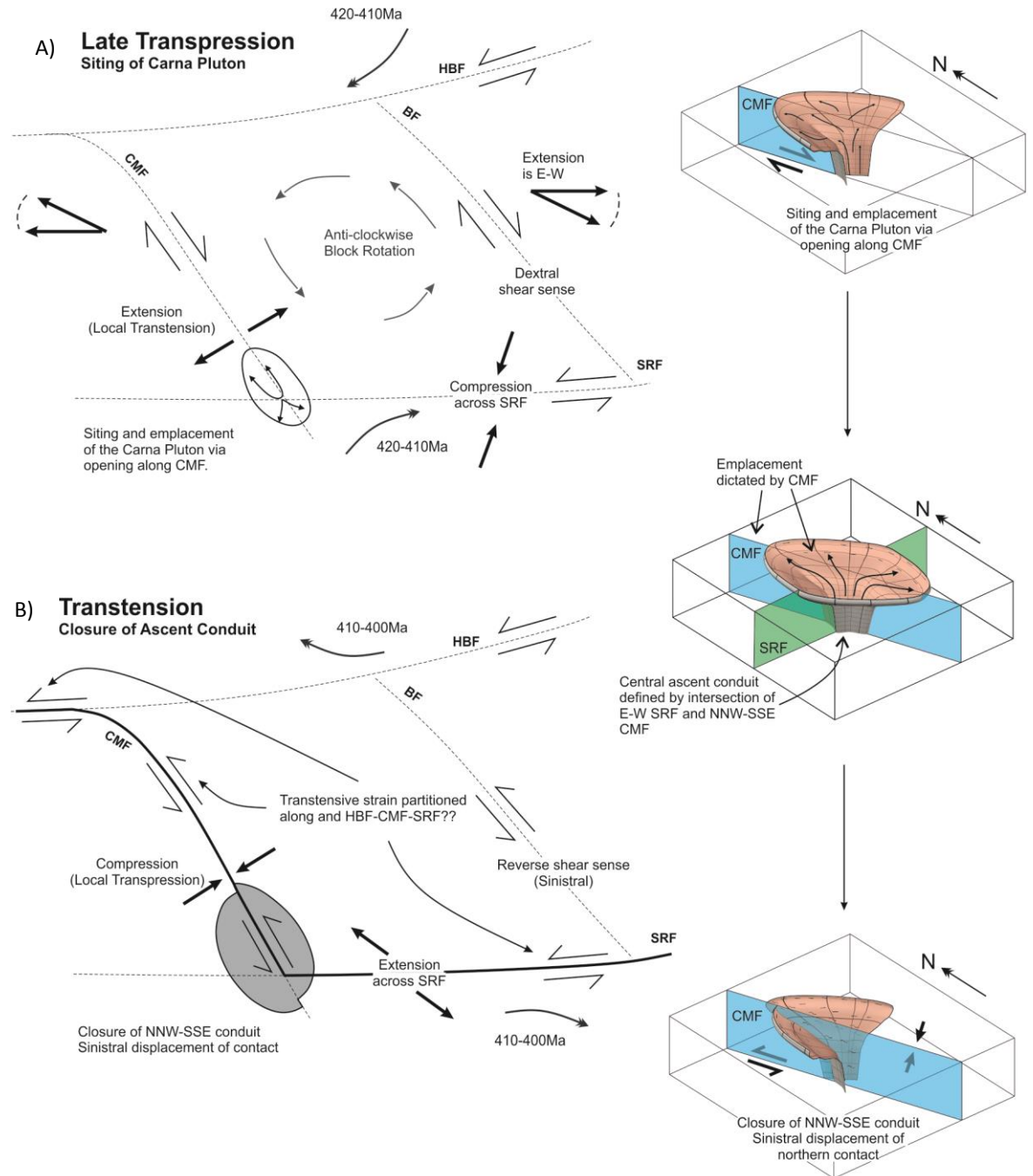
Fig. 9.22 Proposed relationship between regional stress, local structure and the construction of the Carna Pluton. A) Regional sinistral transpression promotes net E-W extension across the CMF and N-S compression across the SRF. A vertical ascent conduit forms over the intersection of these structures and magma preferentially migrates along the CMF at the site of emplacement where inflation commences. B) The transpression-transtension transition occurs between 412-409Ma as regional transtension causes net compression across the CMF and extension across the SRF. This terminates magma ascent along the CMF as the SRF provides a new path of least resistance for over-pressured magma leading to the emplacement of the Kilkieeran Pluton.
