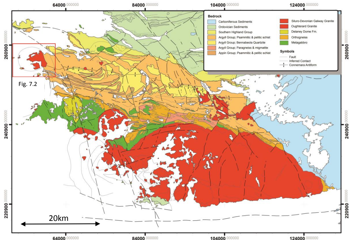
Fig. 7.1 Summarised geology of Connemara. D4 Connemara Antiform axis trends ESE-WNW across the region and is cross cut by the Omev Pluton in the west. Several northwest-southeast and southwest-northeast D5 faults cross cut the Connemara Metamorphic Complex and some members of the Galway Granite Complex.
