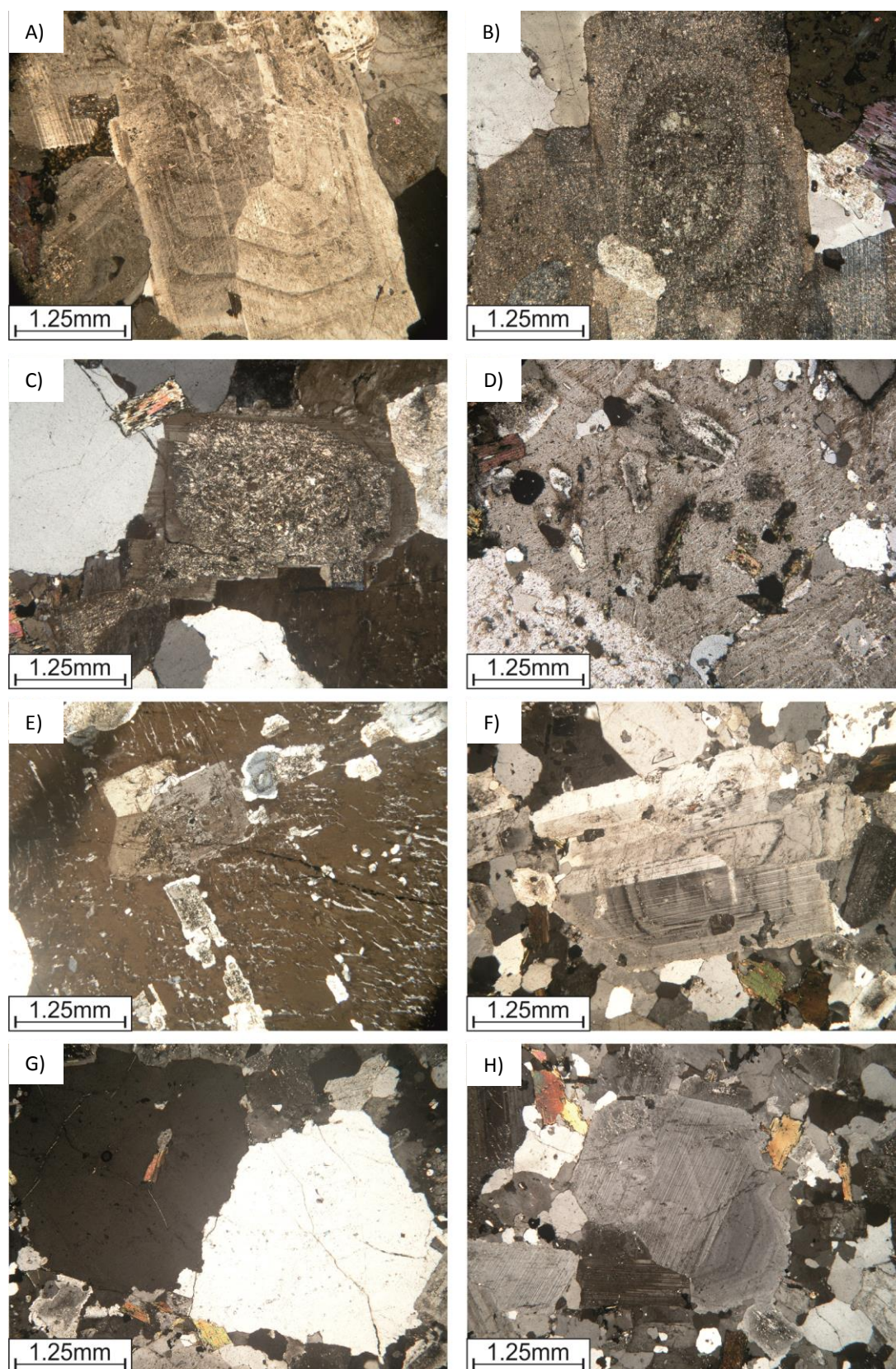
Fig. 7.3 Characteristic petrographic features of facies G1 and G2. Calcic spikes are extensively sericitized (A, B). Feldspars are partially altered and commonly extensively replaced by sericite (B, C). Poikilitic K-feldspars exhibit 0.5-2mm quartz, euhedral feldspar and oxides that accreted to or nucleated on the once outer margins of the phenocrysts crystal lattice (D, E). Micropertthite texture with thin exsolution lamellae of albite flames in K-feldspar (E). G2 is distinguished from G1 by the presence of larger K-feldspars (E) and rounded quartz (G, H).
