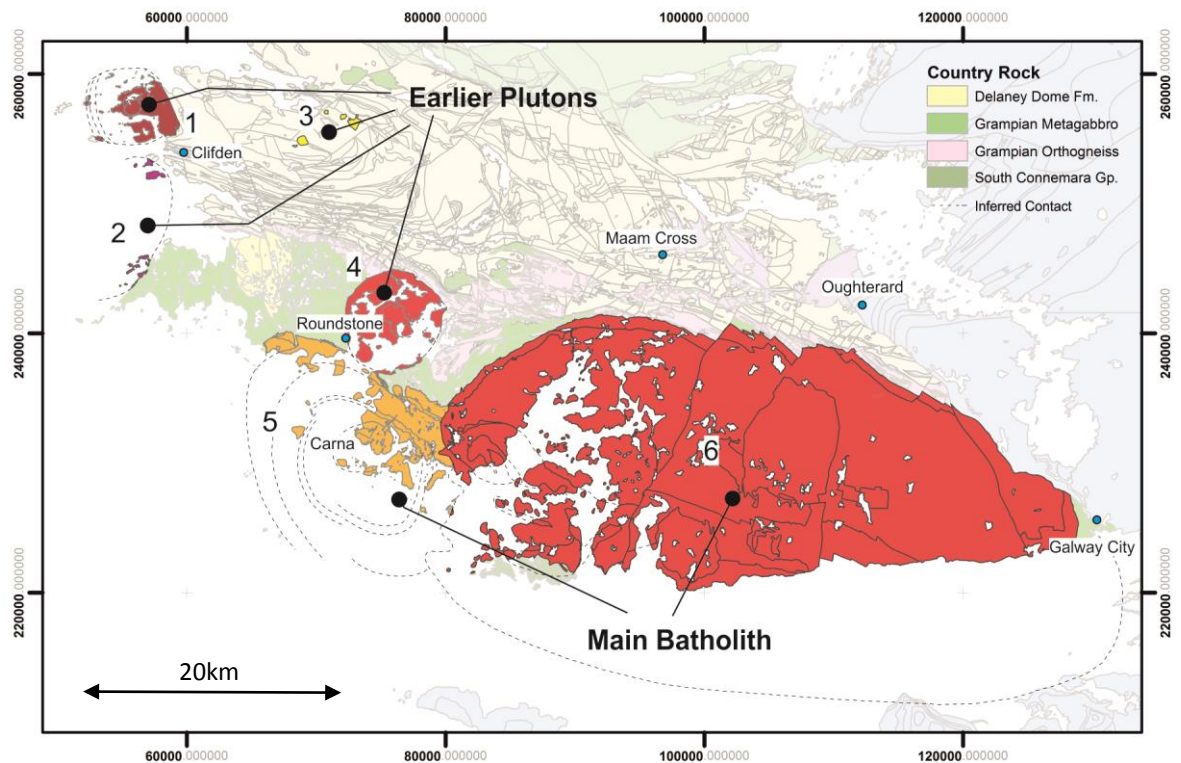
Fig. 5.1 The Siluro-Devonian Galway Granite Complex is comprised of the Earlier Plutons and the Main Batholith both of which comprise of several temporally, structurally and petrographically distinct plutons. Pluton names; 1 = Omev, 2 = Innis, 3 = Letterfrack, 4 = Roundstone, 5 = Carna, 6 = Kilkieran.
