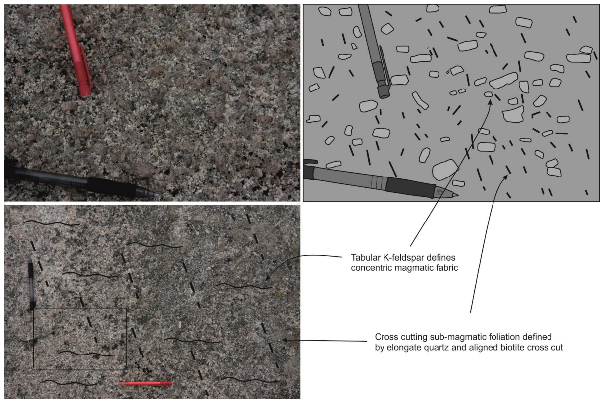
Fig. 9.6 Concentric K-feldspar defined inflation fabric cross-cut by NNW-SSE tectonic foliation associated with submagmatic shearing along the Clifden - Mace Fault (North of Gorteen Bay).
