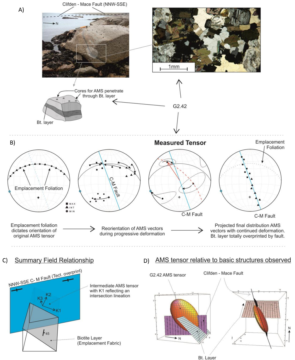
Fig. 9.21 A) Sample collected from biotite layer with no obvious tectonic deformation (Dogs Bay). B) The AMS tensor reflects a composite of an concentric emplacement and a NNW-SSE tectonic foliation. C) Simplified field relationship at sample site with fault cross cutting inclined biotite layer. D) Data shows K1 axis of AMS tensor is close to parallel to the intersection lineation defined by magmatic and tectonic foliations. Shearing must have occurred in the pre-solid state as this sample shows no evidence of brittle or low temperature deformation (A).
