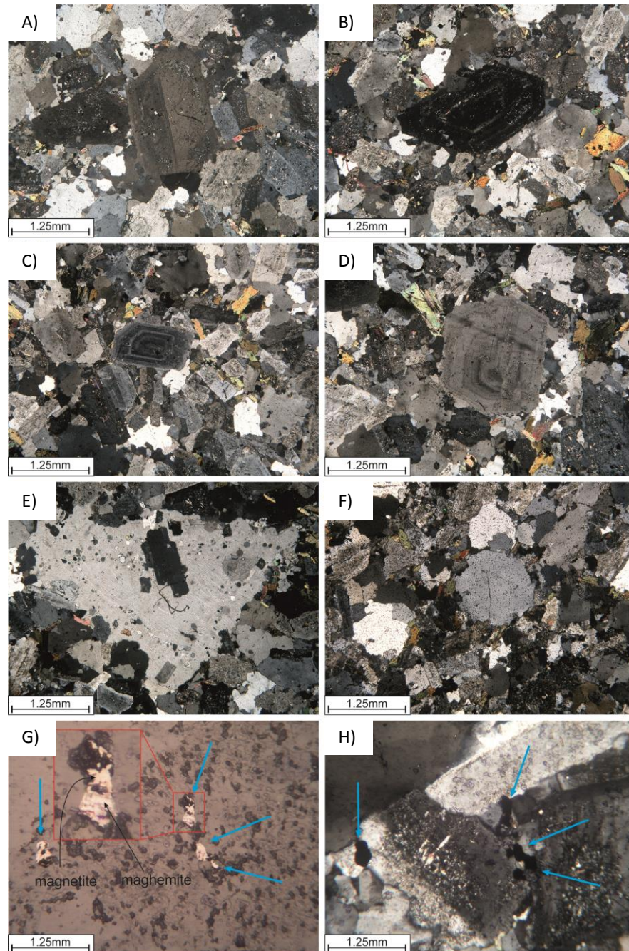
Fig. 8.7 Characteristic petrography of G2. G2 exhibits a finer grained ground mass, strongly complexly zoned euhedral xenocrysts of plagioclase with distinctive calcic spikes (A-D) and rounded quartz (F). Some K-feldspar phenocrysts contain relic crystal margins with agglutinated matrix mineral inclusions (E). Coarse magnetite is typically interstitial and partially oxidised to maghemite along grain boundaries (G & H).
