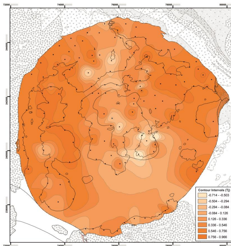
Fig. 8.20 Contour map of Tj values determined from AMS analysis. Again an anomaly is observed along the central NNW-SSE axis where prolate ( \leq 0 \geq -1 ) tensors are detected. The highest shape anisotropies are oblate and are located in the east and west but peak values are associated with the inner strain zone and not the pluton's marginal fabric.
