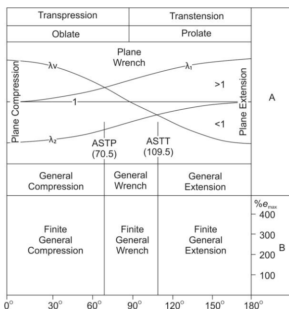
Fig. 10.3 Graphical solutions of McCoss (1986) for determining the characteristics of the infinitesimal strain ellipsoid (A) and the finite strain ellipsoid (A & B) progressively through compressive to transcurent to extensional stress fields. In any system the transition between transtension and transpression will occur progressive through the classic "wrench tectonics" field, and in most systems some element of compression or extension is expected. Axially symmetric transpression and transtension are denoted by ASTP and ASTT respectively, \lambda_v is the vertical principal quadratic elongation, \lambda_1 and \lambda_2 are the horizontal principal strains. e_{max} is the maximum finite extension.
