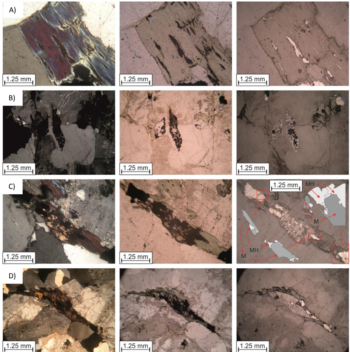
Fig. 7.5 Left to right, XPL, PPL and RL images of representative samples that show the relationship between iron oxide phases and silicate minerals. A; Elongate aggregates of magnetite along cleavage planes within biotite. B; Alteration of titanite with product magnetite pseudomorphing the original mineral. C; RL image shows three blow-ups of magnetite crystals (dark gray) that have been undergone maghemitization along fracture and crystal margins (light gray). D; . Altered biotite pseudomorphed by secondary magnetite.
