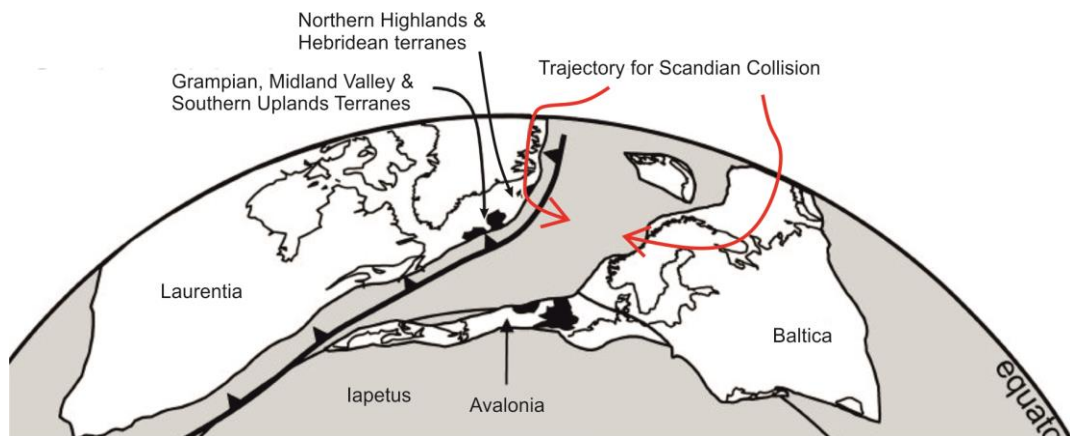
Fig. 2.7 Pre-Scandian (~ 450Ma) distribution of Laurentia, Baltica and Avalonia.
