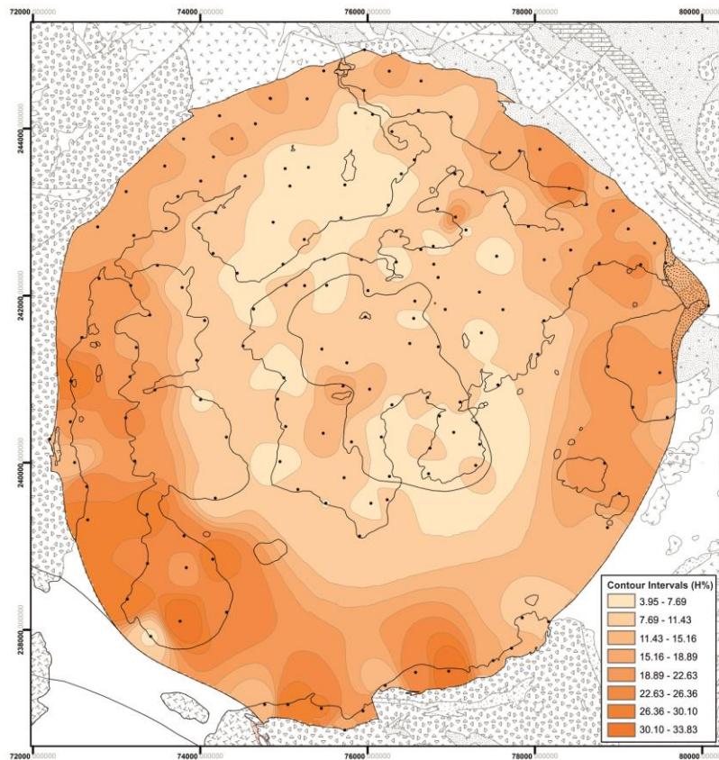
Fig. 8.19 Contour map of H values determined from AMS analysis. A low degree of anisotropy is associated with the core and NNW-SSE axis of the intrusion. The highest H values are in the west and east. Note that peak values are not always associated with the margins of the intrusion and are concentrated in the ENE and WSW, this is inconsistent with a straightforward ballooning scenario.
