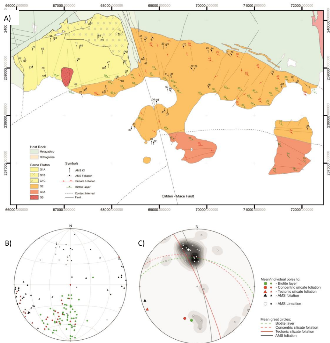
Fig. 9.20 A) Blow up map of the Dogs Bay area and summarised fabric data. B) stereonet of all data plotted in (A), (C) is the same data summarised with K1 axes of AMS contoured. Note that the mean K1 axis defined by all data lies along the intersection of the concentric ballooning fabric and the tectonic overprint.
