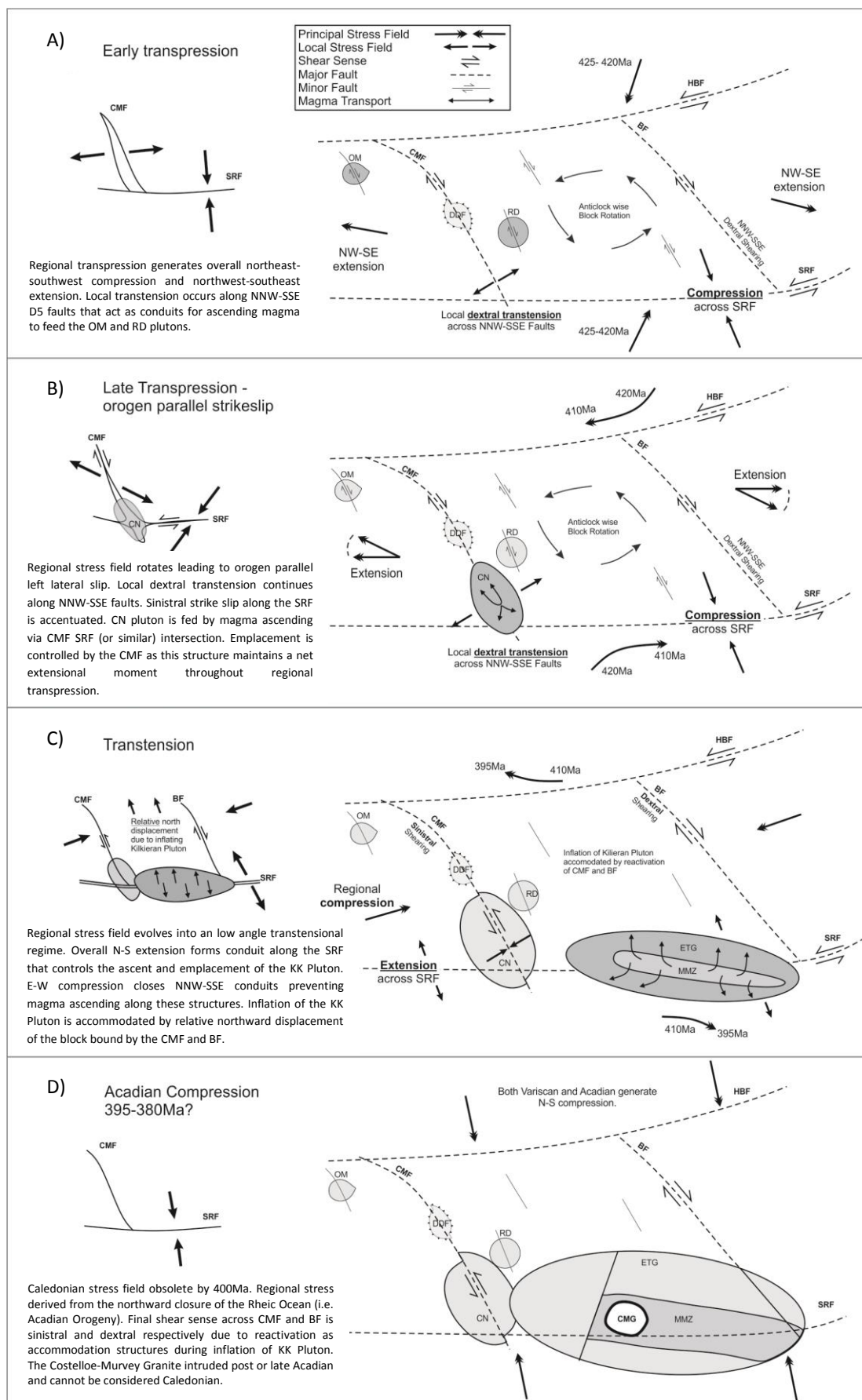
Fig. 10.6 Proposed model for the interaction of local structure, igneous intrusions and the evolution of the regional stress field from the late Silurian to mid-Devonian.
