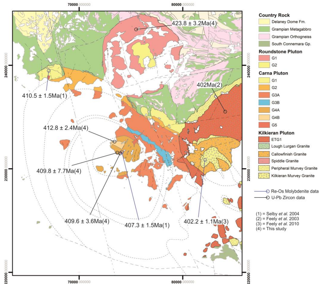
Fig. 9.8 Compilation of old and new chronological data for the Carna and Roundstone plutons (Leggo et al. (1966) and Pidgeon (1969) omitted).
