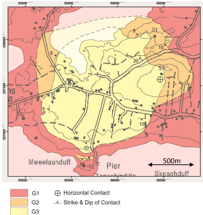
Fig. 7.10 A map of the central portion of the Omev pluton. Contacts between G1, G2 and G3 are almost exclusively gradational and thus the orientation cannot be directly measured. Mapped contacts east of Aughrus Hill and north of Mweelaunduff are approximately contour parallel and therefore likely to be subhorizontal. A very gently inclined sharp G1-G3 contact is observed in the west. Contours mapped in the north east and southern part of the map cross cut topographic contours and thus must be inclined.
