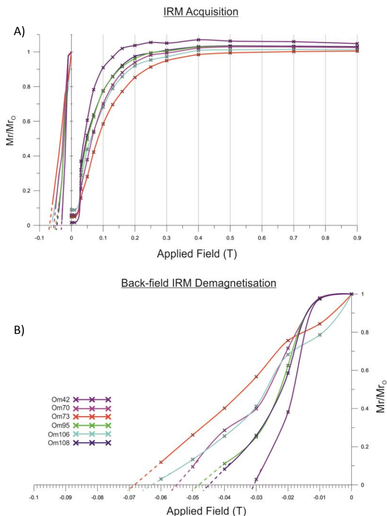
Fig. 7.23 A) results of SIRM acquisition experiments. B) Results of BIRM demagnetisation experiments. All samples exhibit exponential demagnetisation curves and are saturated in less than 0.3T (exception of OM73). Those samples which the highest coercivity values (OM73 & OM106) also required higher AF - demagnetising fields in the Lowrie - Fuller test.
