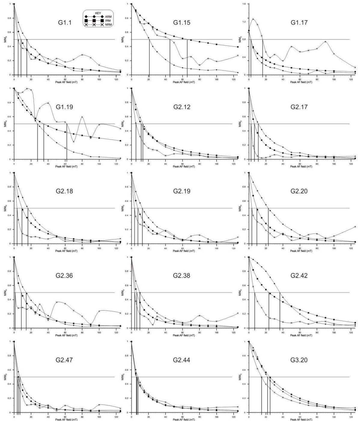
Fig. 9.13 Graphed results of Lowrie-Fuller test (continued below).
