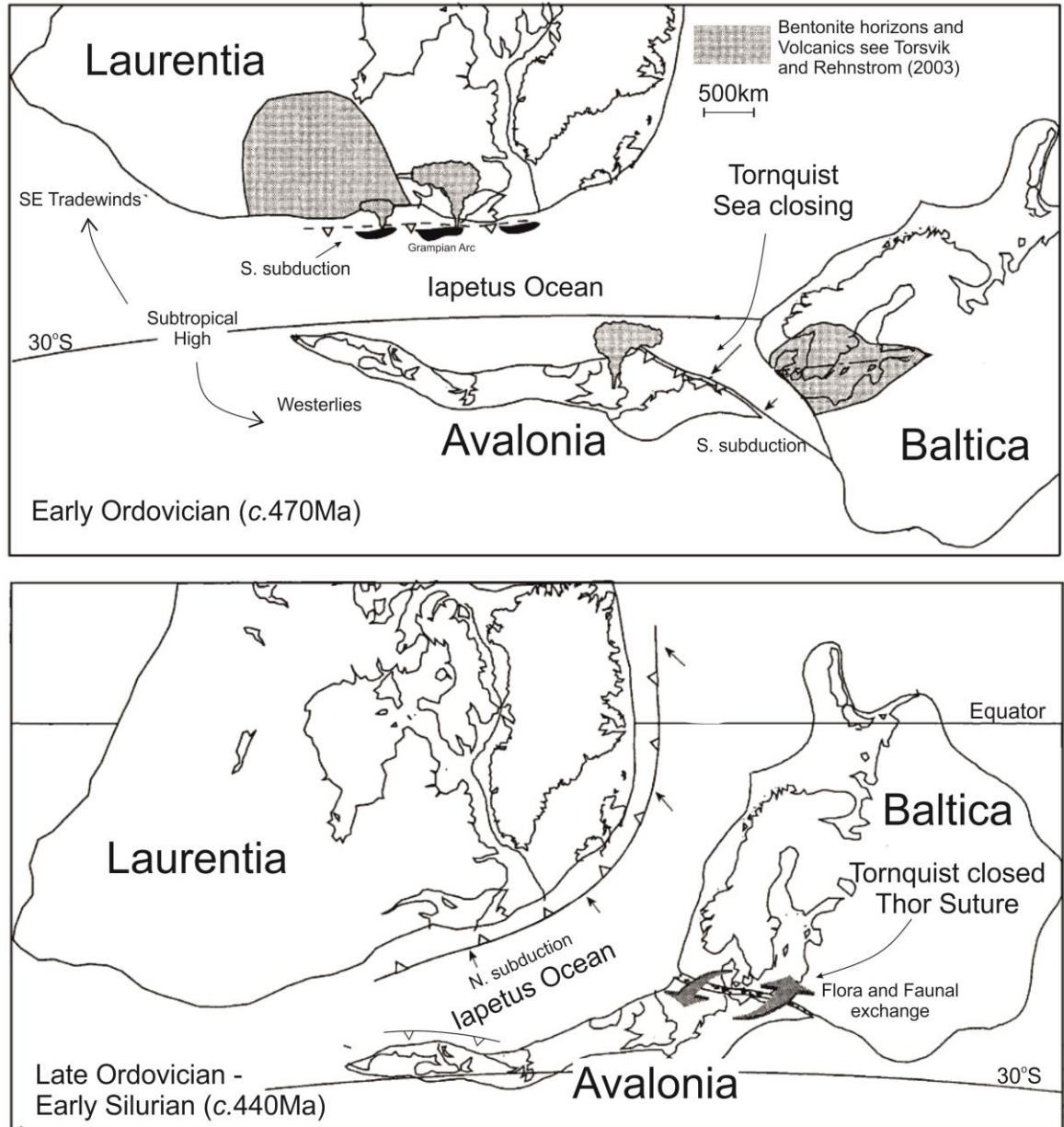
Fig. 2.6 Distribution and relative movements of continents boarding the Iapetus between ~ 470-440Ma during the closure of the Tornquist Sea (adapted from Torsvik and Rehnström (2003)). Volcanism on the Avalonian continent was driven by southward subduction of oceanic crust as Baltica converged on Avalonia and the Tornquist sea closed. Isotopic evidence from this process as well as floral and faunal evidence, places temporal constraints on the timing of this closure. Note Grampian subduction flip on southern Laurentian coast. Note the timing contrast between this model and that in Fig. 2.10.
