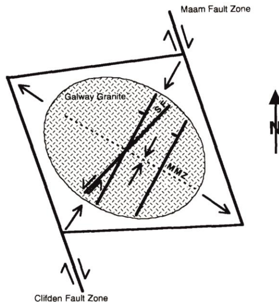
Fig. 5.5 Schematic model for the emplacement of the Main Batholith (Kilkieran Pluton and Carna Pluton) as proposed by El-Desouky et al. (1996). In this model, space for magma ingress was created by dextral shearing along the Clifden Fault and Maam Fault which acted as bounding translation faults to a crustal pull apart. El-Desouky et al. (1996) suggested that the MMZ intruded parallel to the compressive axis of the batholith and the Shannawona Fault (SF) cross cut the core of the pluton as a left lateral dip slip release structure.
