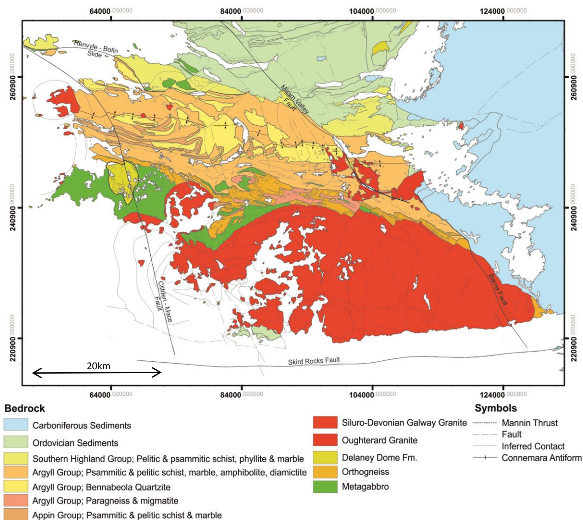
Fig. 3.2 Bedrock geology of Connemara and major structures. The CMC was thrust south along the Mannin Thrust and over the Delaney Dome Fm.. The Oughterard Granite intruded soon after and the Siluro-Devonian granites were emplaced at the end of the Caledonian Orogeny.
