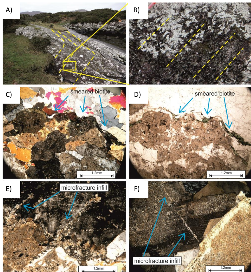
Fig. 8.11 A & B; Typical examples of low temperature marginal fabrics at outcrop scale (blue in Fig. 8.10). C & D; Smearing of biotite (C & D) and fracturing of feldspars infilled with quartz and feldspars indicate deformation occurred under low temperature conditions
