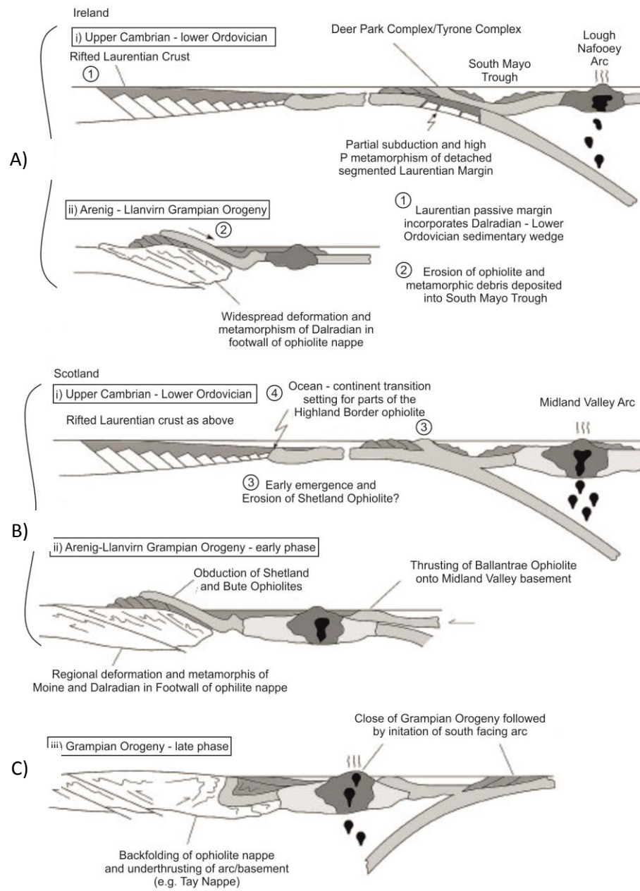
Fig. 2.5 The Grampian orogenic phase of the Caledonian Orogeny (schematic diagram from Woodcock and Strachan (2012) after Ryan and Dewey (1991). (A) and (B) are equivalent examples of Grampian events based on evidence from Ireland and Scotland respectively. In both cases initial southward subduction of ocean crust (i) drives arc magmatism and the formation of the a forearc basin and convergence of the island arc with Laurentia (ii) causes obduction of oceanic crust onto the Laurentian margin. (C/iii) Continued closure of Iapetus causes a new forearc basin to form to the south of the accreted island arc and Laurentia and northward subduction of Iapetan oceanic crust.
