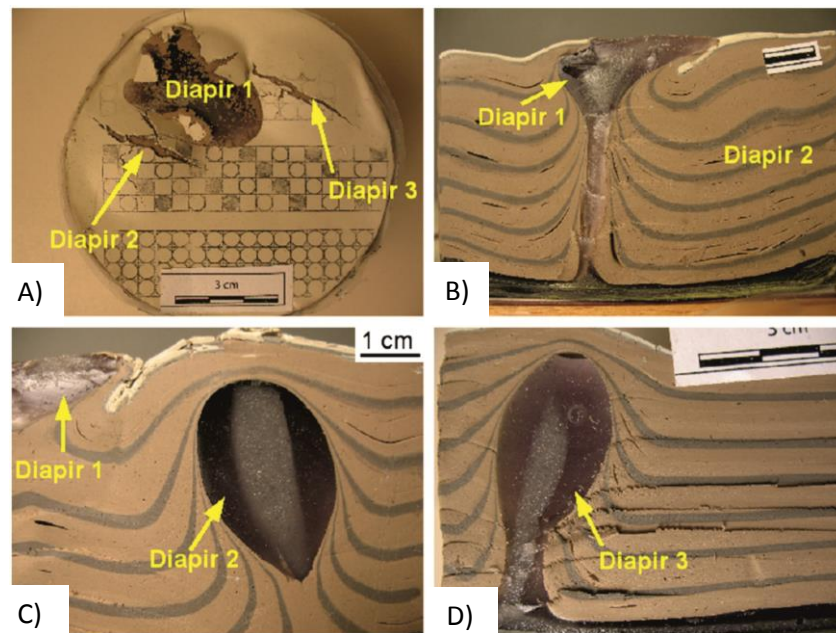
Fig. 1.3 Results of centrifuge analogue experiments using plasticine-silicone materials of differing density (Dietl and Koyi (2011)). Many of the structures recognised are comparable to real field observations (isoclinal folds, doming and fracturing of overburden, concentric internal architecture of diapir, rim synclines). In this model “magma” ascent is achieved due to a buoyancy contrast between the plasticine and silicone. However, in reality a buoyancy contrast between host and magma is not always present, or magma may be denser than the host. As such, this model cannot account for the ascent and emplacement of all intrusive bodies.
