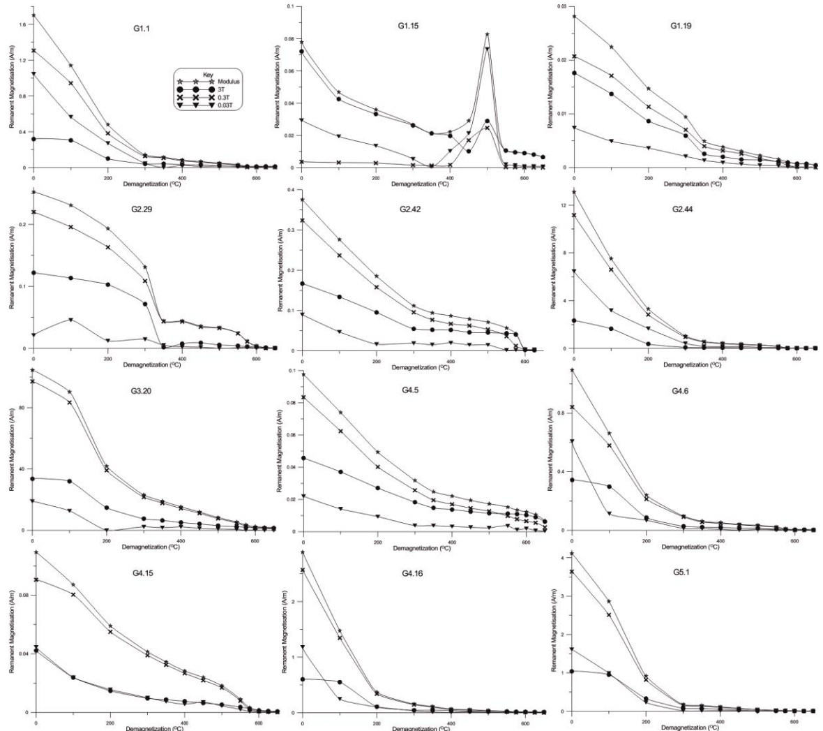
Fig. 9.15 Graphed results of 3 component demagnetisation. The majority of samples are dominated by moderate coercivity minerals (0.3T). G1 samples are atypical and exhibit a large high coercivity fraction.
