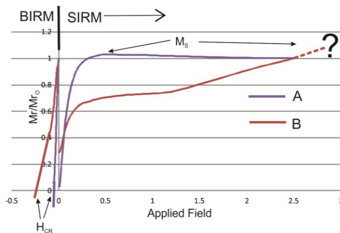
Fig. 6.12 SIRM and BIRM acquisition and demagnetisation curves for samples "A" and "B" (same as those used in Fig. 6.11) Rapid acquisition of remanence and demagnetisation of "A" shows low coercivity minerals dominate. Sample "B" never reaches saturation and carries much higher H_{CR} value. This is consistent with the presence of higher coercivity minerals in B relative to A and is consistent with the data shown in Fig. 6.11.
