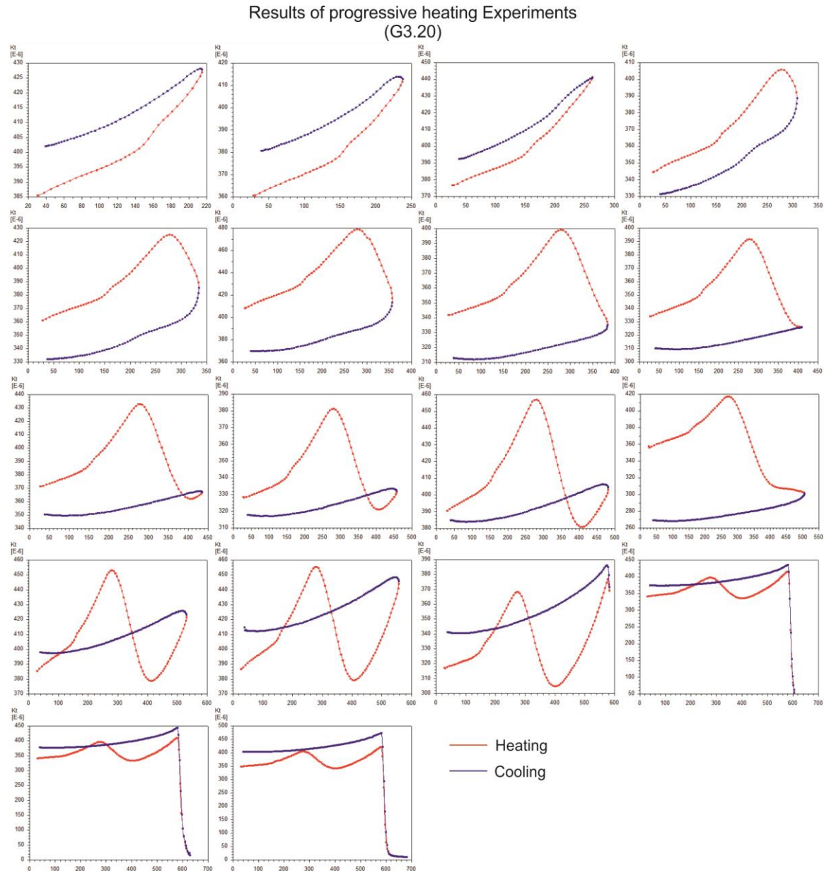
Fig. 9.12 Progressive stepwise heating of G3.20 shows defined "bump" between 250-350°C. No net change in susceptibility occurs prior to 250°C. Between 250-450°C a net decrease in susceptibility is noted on the cooling curve and the "bump" is erased. From 450-520°C an abrupt increase on the heating curve is accompanied by a net increase on the cooling curve. This sharply contrasts the results of G1.15 as susceptibility on the cooling curve initially decreases at lower temperatures and then increases at a much more abrupt rate over 450°C.
