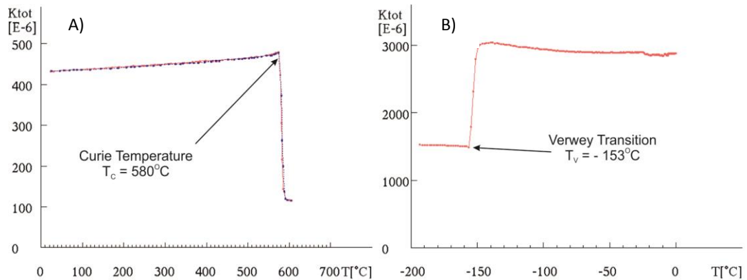
Fig. 6.10 Schematic graph of the variation of susceptibility in pure magnetite with temperature. A) The susceptibility of magnetite increases with temperature up to the Curie Temperature where the mineral undergoes a transition from a ferrimagnetic to paramagnetic state, this is associated with a major decrease in susceptibility. B) At low temperature magnetite undergoes a transition from cubic to orthorhombic symmetry, this is indicated by an abrupt decrease in susceptibility and is termed the Verwey Transition.
