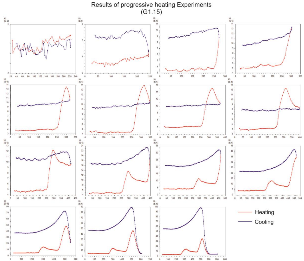
Fig. 9.11 Progressive stepwise heating of G1.15 shows no net change in susceptibility occurs prior to 250°C, over this temperature a net increase is observed on the cooling curve which stabilises up to 400°C. From 400-600°C a second increase in susceptibility is recorded, over this temperature range the relative magnitude on the cooling curve progressively increases as the sample is exposed to higher temperatures over longer time intervals. The heating curve "bump" is fully erased from the cooling curve by 325°C.
