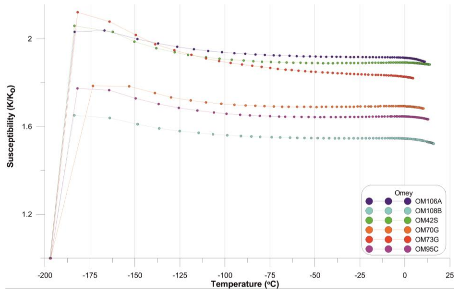
Fig. 7.21 Results of cryogenic experiments show little variation among the sample population. All exhibit a rapid increase in susceptibility between -198°C and -170°C (at T_v ) followed by a gradual decline up to room temperature.
