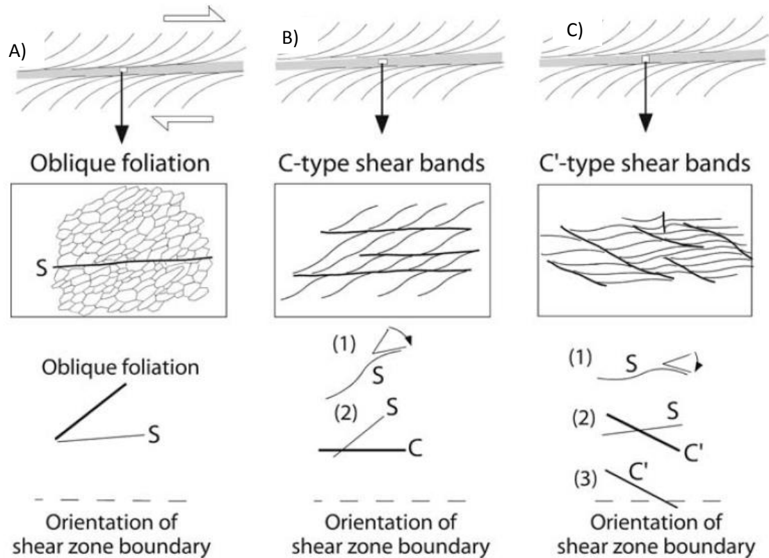
Fig. 6.6 Development of S,C and C' fabrics within shear zones (from Passchier and Trouw (2005)). A) A S-type fabric. B) C-type S-C fabric due to compression, the C-plane is parallel to the shear zone boundary and laterally continuous. C) C' type S-C fabric due to extension, the C-plane is oblique to the shear zone boundary and is laterally discontinuous.
