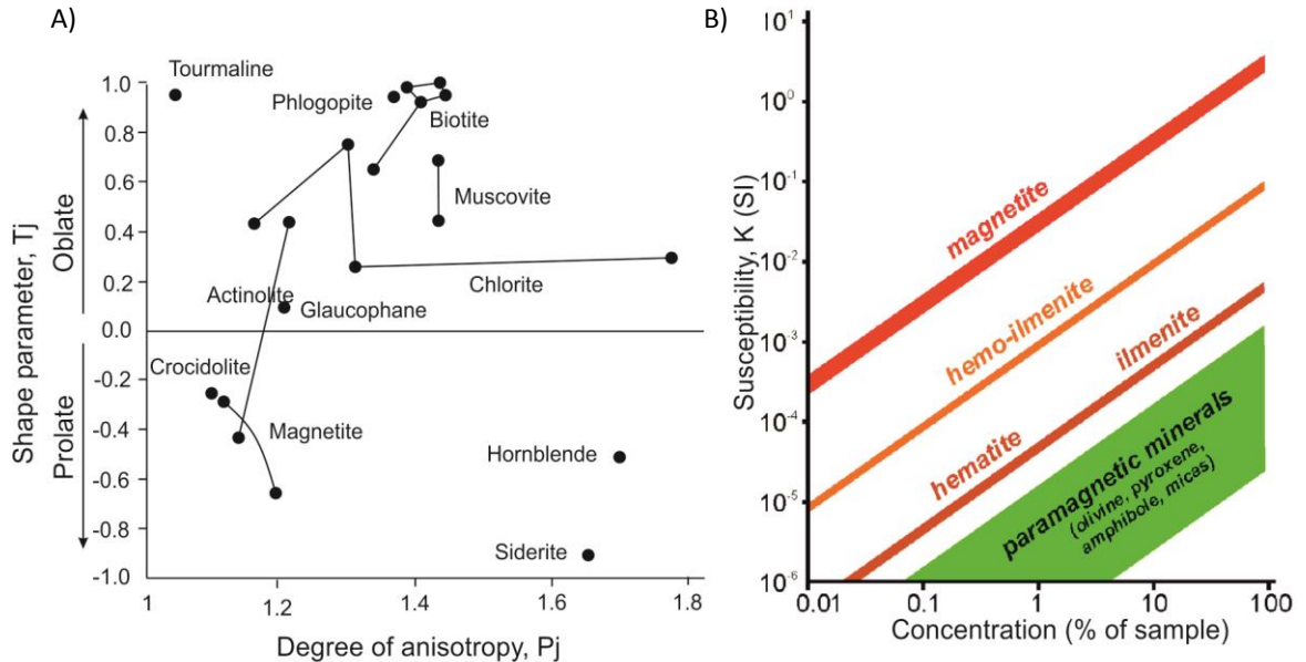
Fig. 6.9 A) Low field magnetic susceptibility shape anisotropy and degree an anisotropy parameters of some minerals (from (Tarling and Hrouda 1993)). Shape anisotropy values in many paramagnetic minerals are much higher and more consistent that those associated with magnetite. B) The contribution of different mineral phases to the bulk magnetic susceptibility of a rock depends on the minerals intrinsic susceptibility and concentration (after Hrouda and Kahan (1991)). For example, <0.5% modal abundance of magnetite will generate a higher susceptibility than a >50% modal abundance of biotite.
