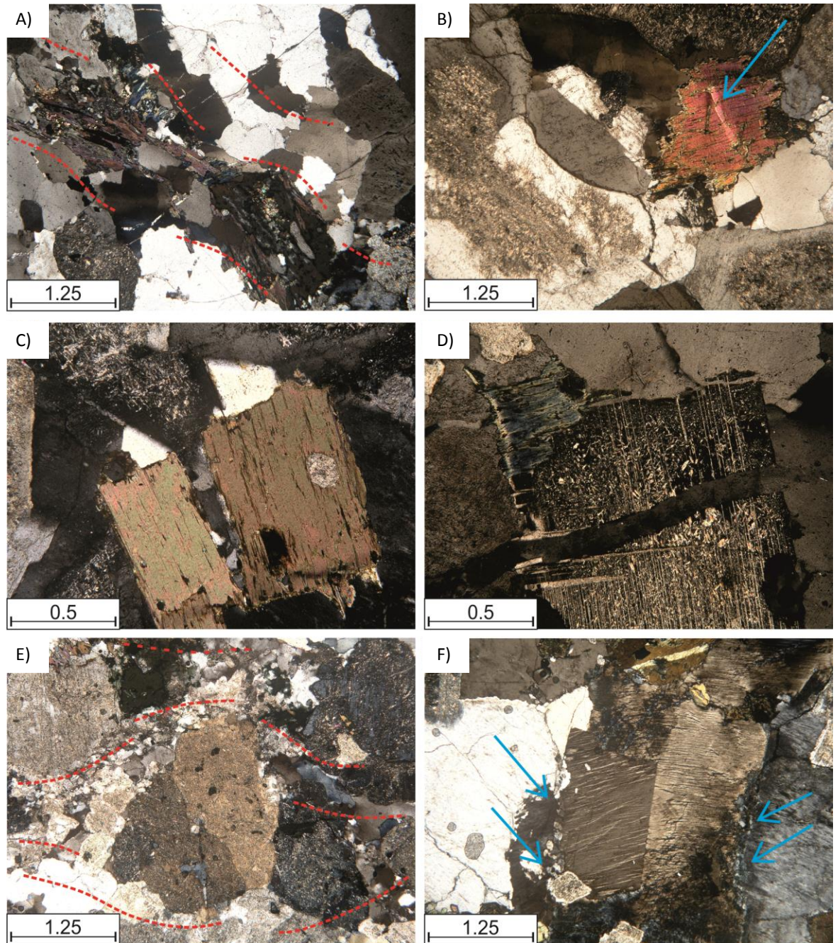
Fig. 7.19 XPL images of microstructural observed within a NNW-SSE shear zone on Aughrus Point. A) Quartz ribbons and smeared biotite. B) Minor kink in biotite, undulose extinction in quartz. C) Fracture along biotite cleavage plane and (D) fracture through plagioclase both with primary magmatic quartz infill shows submagmatic deformation occurred. E & F) Marginal dynamic recrystallisation of plagioclase into the foliation plane.
