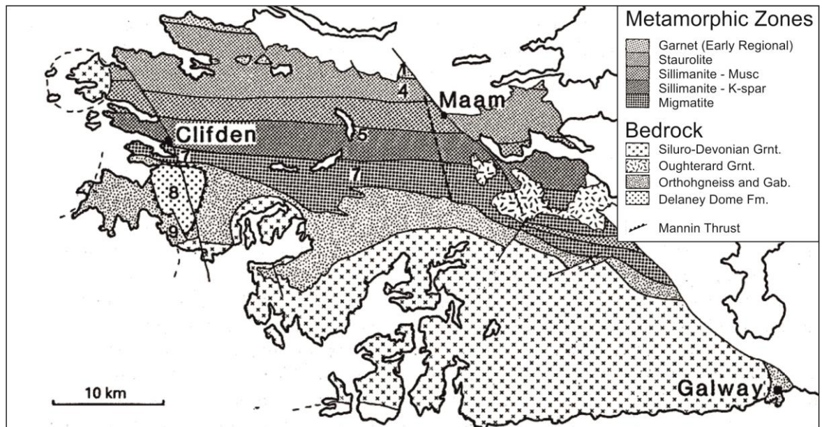
Fig. 3.8 Regional metamorphic zones defined across Connemara (from Yardley (1980)). Early Regional high pressure low temperature garnet bearing M1 is largely overprinted by M2 which show a progression in grade from north to south. Rocks in direct contact with the Gabbro and Orthogneiss Complex are migmatised.
