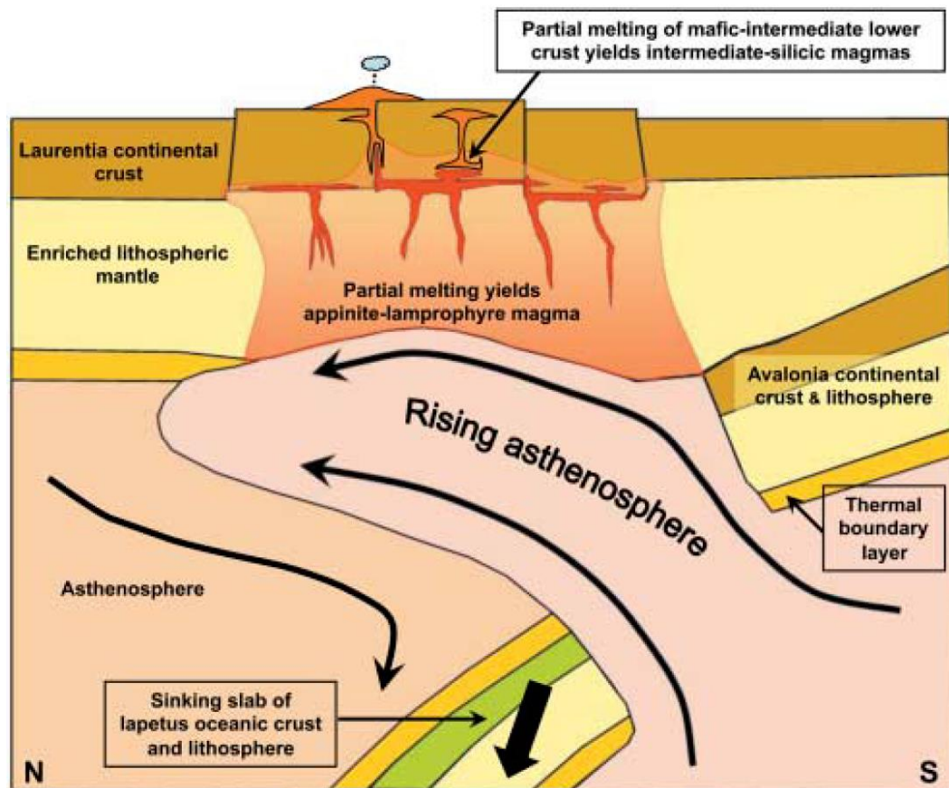
Fig. 4.2 Cartoon diagram of the leading petrogenetic model for the Northern Granites (from Neilson et al. (2009)). Based off the slab break off model of Atherton and Ghani (2002), this model shows partial melting of enriched lithospheric mantle, new crust generation by intrusion of appinite-lamprophyre sheets and crustal recycling of the lower crust to generate associated plutons and volcanoes.
