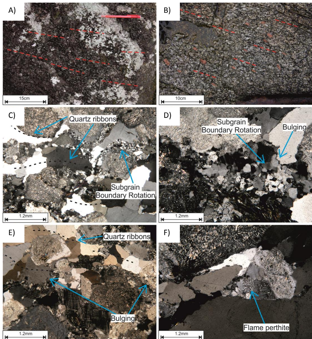
Fig. 8.12 Microstructures associated with the inner foliation zone (red in Fig. 8.19). A; Fabric observed at outcrop scale. B; Observed aligned tabular K-feldspars indicating the fabric formed in the submagmatic state. C, D & E; microstructural analysis shows deformation was achieved through bulging and subgrain boundary rotation indicating deformation occurred in the submagmatic state. F; Flame perthite is rare but
