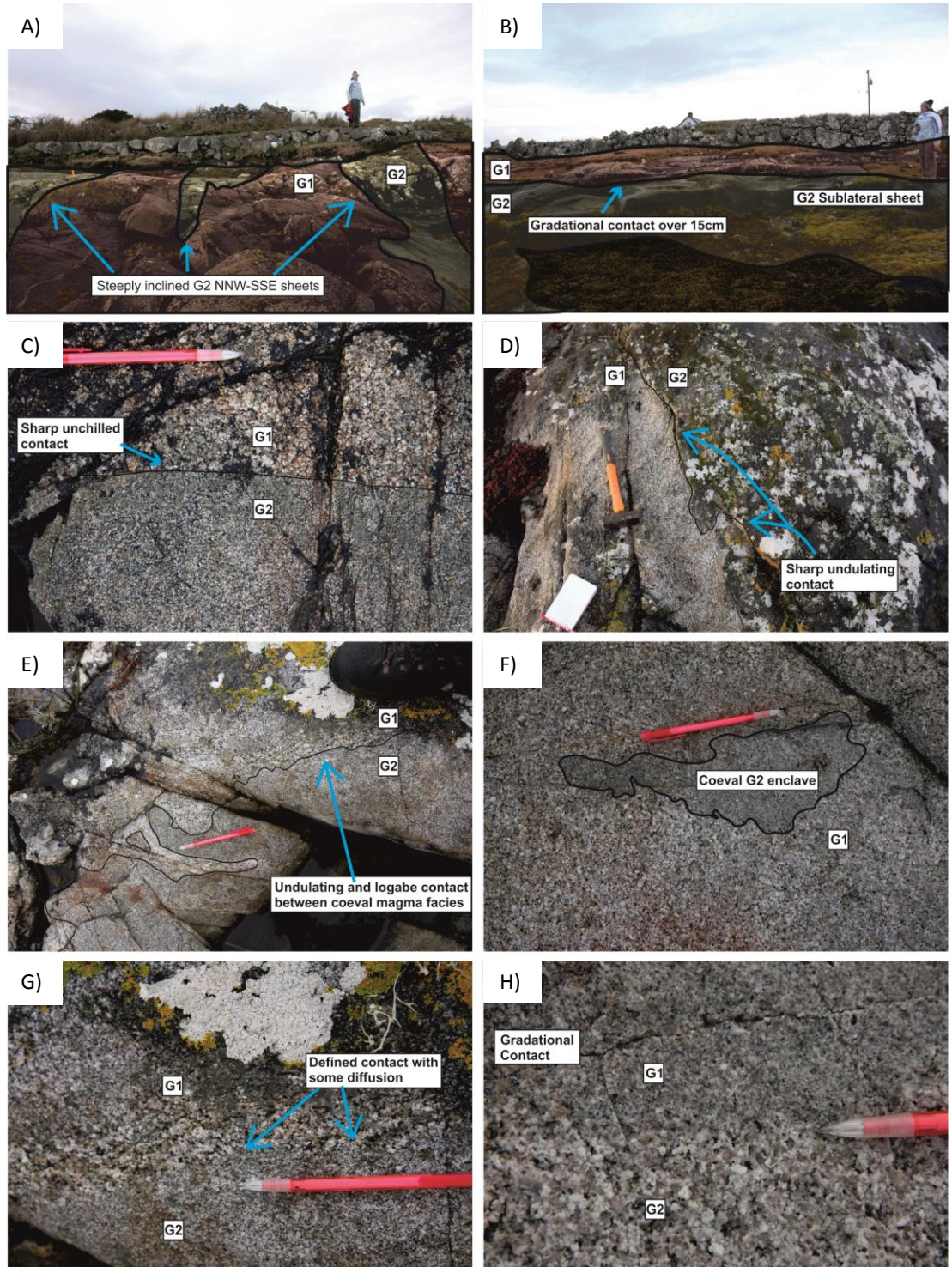
Fig. 8.8 A variety of gradational, highly lobate and sharp G1-G2 contacts show G1 was cooling as G2 continued to intrude (A-H). Enclave of G2 with lobate contacts hosted in G1 (F).
