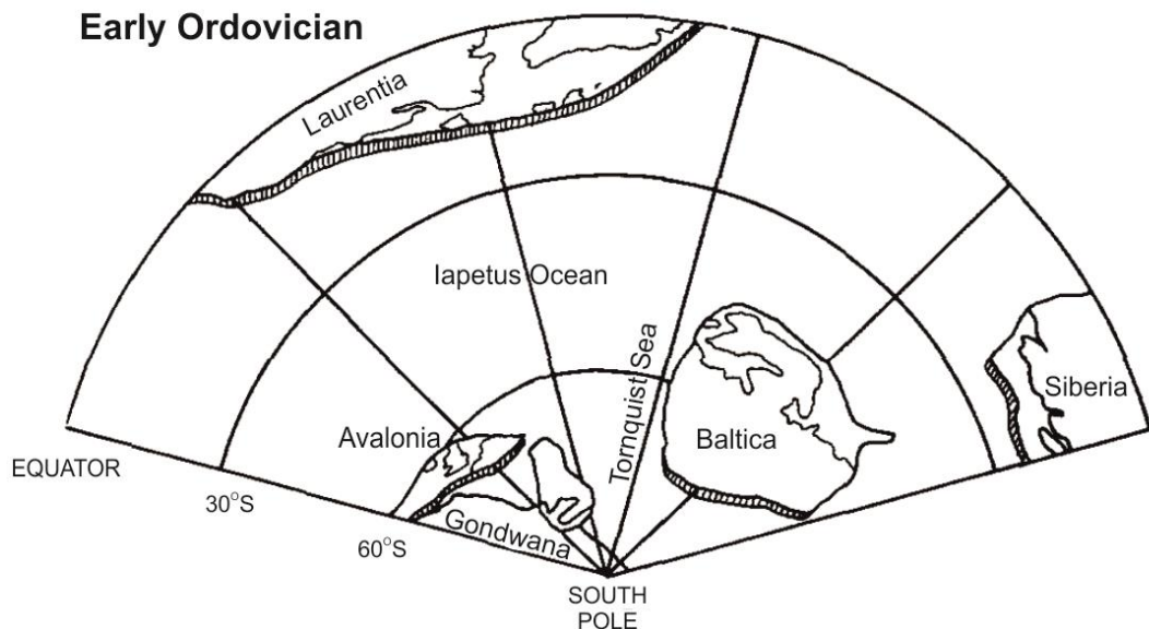
Fig. 2.2 Basic distribution of the continents bordering the Iapetus Ocean in the early Ordovician. Adapted from Trench and Torsvik (1992).
