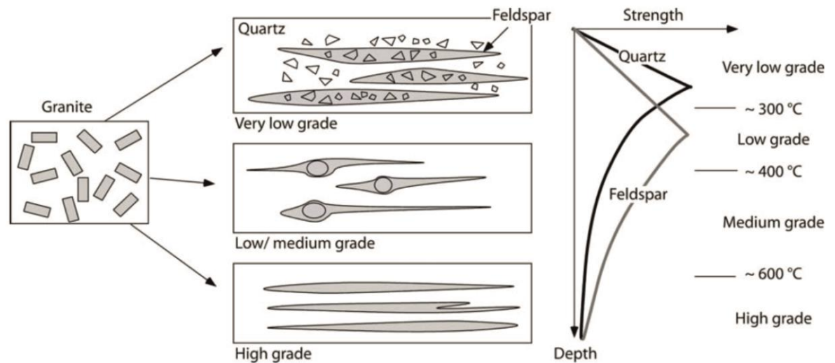
Fig. 6.3 Contrasting deformation behaviour of quartz and feldspar (from Passchier and Trouw (2005)). At low temperature quartz is more competent. Quartz begins to deform in a ductile fashion at lower temperature than feldspar and becomes less competent under moderate temperature conditions. At higher temperatures both minerals have similar strength properties.
