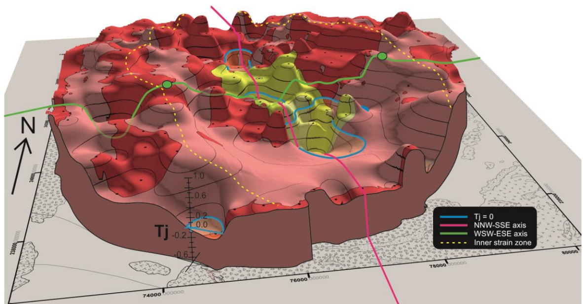
Fig. 8.23 Digital elevation model using T_j as the z-axis parameter draped with basic facies map of the pluton. Note that the highest T_j values (highly oblate) occur along two arcs marked in dashed yellow which define an oval elongate along a NNW-SSE axis. Green dots mark the localities with the highest T_j values, these define a line orthogonal to that defined by the lowest T_j and H values.
