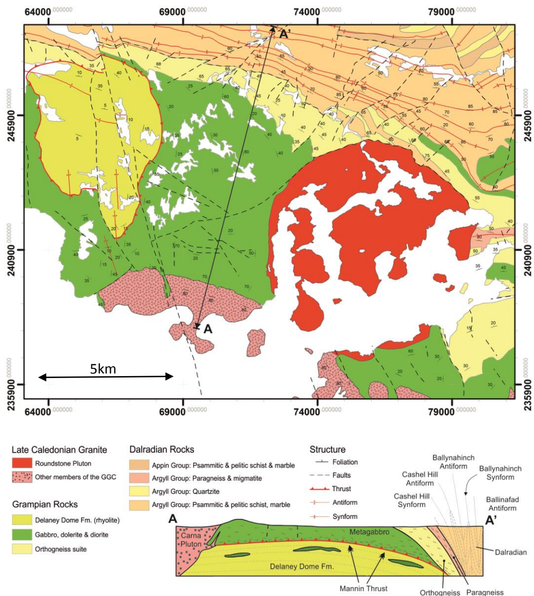
Fig. 8.1 Summary geological map of the study area (modified after Leake and Tanner (1994)) and cross section (modified after Leake (1986)). The Connemara Metamorphic Complex is intruded by the Roundstone Pluton at the current exposure level. The CMC is a hanging wall to the Mannin Thrust which is exposed \approx 5\text{km} to the west of the pluton. The Roundstone Pluton cross cuts the host rocks WNW-ESE foliation and is cross cut by reactivated D5 faults.
