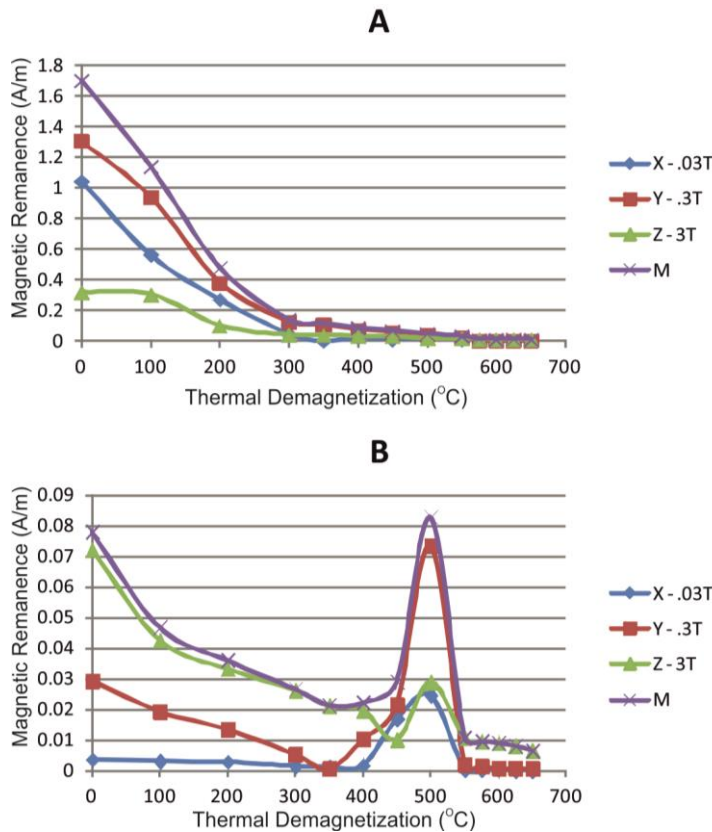
Fig. 6.13 Thermomagnetic Analysis of three-component IRM data from samples A & B (same samples as used above). Sample "A" has a large proportion of the modulus magnetic vector (M) dominated by low (X - 0.03T) and moderate (Y - 0.3T) coercivity minerals, high coercivity minerals are not abundant (Z - 3T). The modulus vector of sample "B" is dominated by high coercivity minerals (Z - 3T) and low coercivity minerals are negligible. These data are consistent with the results shown above and indicate that sample "B" has a magnetic assemblage distinct from sample "A". This contrast in mineral modal abundance means that the AMS of each sample is not directly comparable as it is controlled by entirely different magnetic parameters that are inherent to each mineral assemblage.
