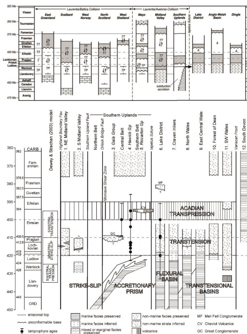
Fig. 10.1 A) Dewey and Strachan (2003) suggest transtension did not initiate until 410Ma. B) Soper and Woodcock (2003) suggest that extension between Laurentia and Avalonian started at 420Ma.
