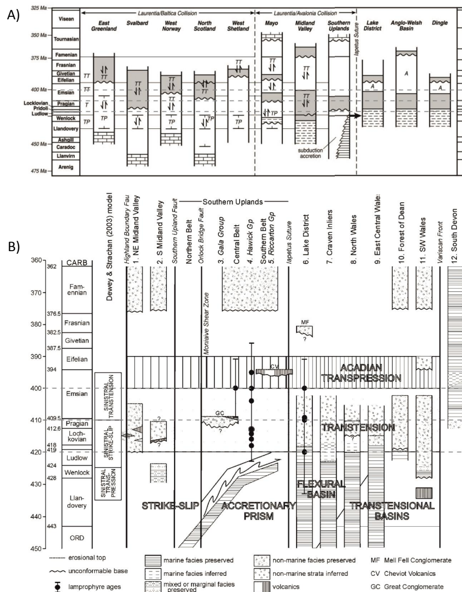
Fig. 2.12 Contrasting tectonostratigraphic columns of Dewey and Strachan (2003) (A) and Soper and Woodcock (2003) (B). (A) TP, transpression; TT, transtension; A, Acadian, shows transtension did not instigate until 410 Ma. (B) Shows more uniform relationship across the studied terranes and transtension initiation at 420 Ma.
