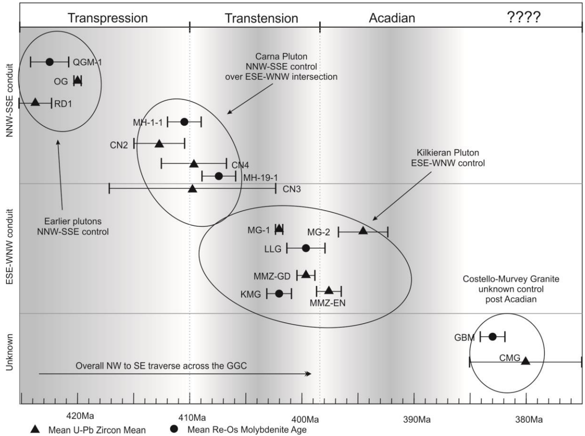
Fig. 10.5 Regional stress field evolution relative to the timing and structural controls over pluton construction. Samples projected correspond to those presented in Table 10.1 and Fig. 10.4.
