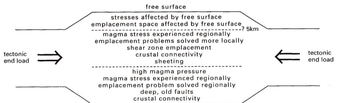
Fig. 1.7 Simplified diagram illustrating the contrast in emplacement styles expected at different crustal depths (Hutton 1996).
