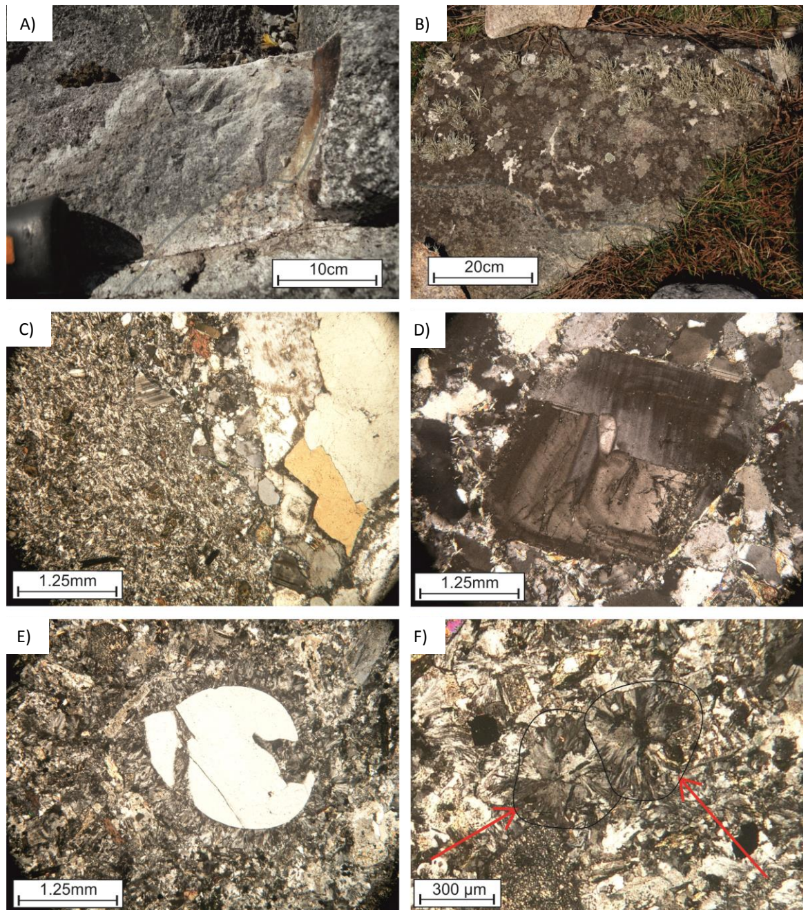
Fig. 7.11 Late porphyritic dykes exhibit narrow gradational (A) or sharp lobate contacts (B) with only minor chilled margins (C) (if present). D) Part of a tabular plagioclase with dramatic zoneation and pericline twins. E) Rounded quartz with peripheral spherulitic quartz. F) Spherulitic quartz aggregates.
