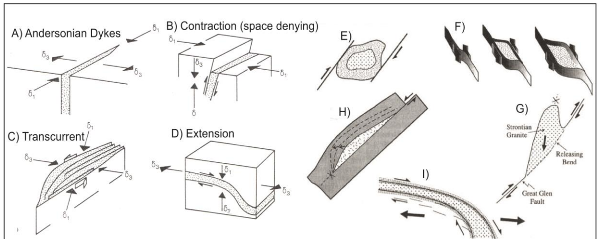
Fig. 1.9 Emplacement can be achieved in contractional, transcurrent and extensional structures highly oblique to the regional stress field (A-D), therefore \sigma_1 must differ from \sigma_L . Contrasting styles of emplacement (Hutton 1996); E) The Rehanna Granite, Morocco intruded into a transtensional pull apart along a wrench fault (Lagarde et al. 1990); F) The Galway Granite, Ireland, intruded into a dilatational jog (Leake 2006); G) the Strontian Granite, Scotland intruded the active Great Glen Fault (Hutton 1988a); H) the Main Donegal Granite, Ireland, intruded at a shear zone termination and I) the Quernetoq Pluton intruded into an active tensional setting (Hutton et al. 1990).
