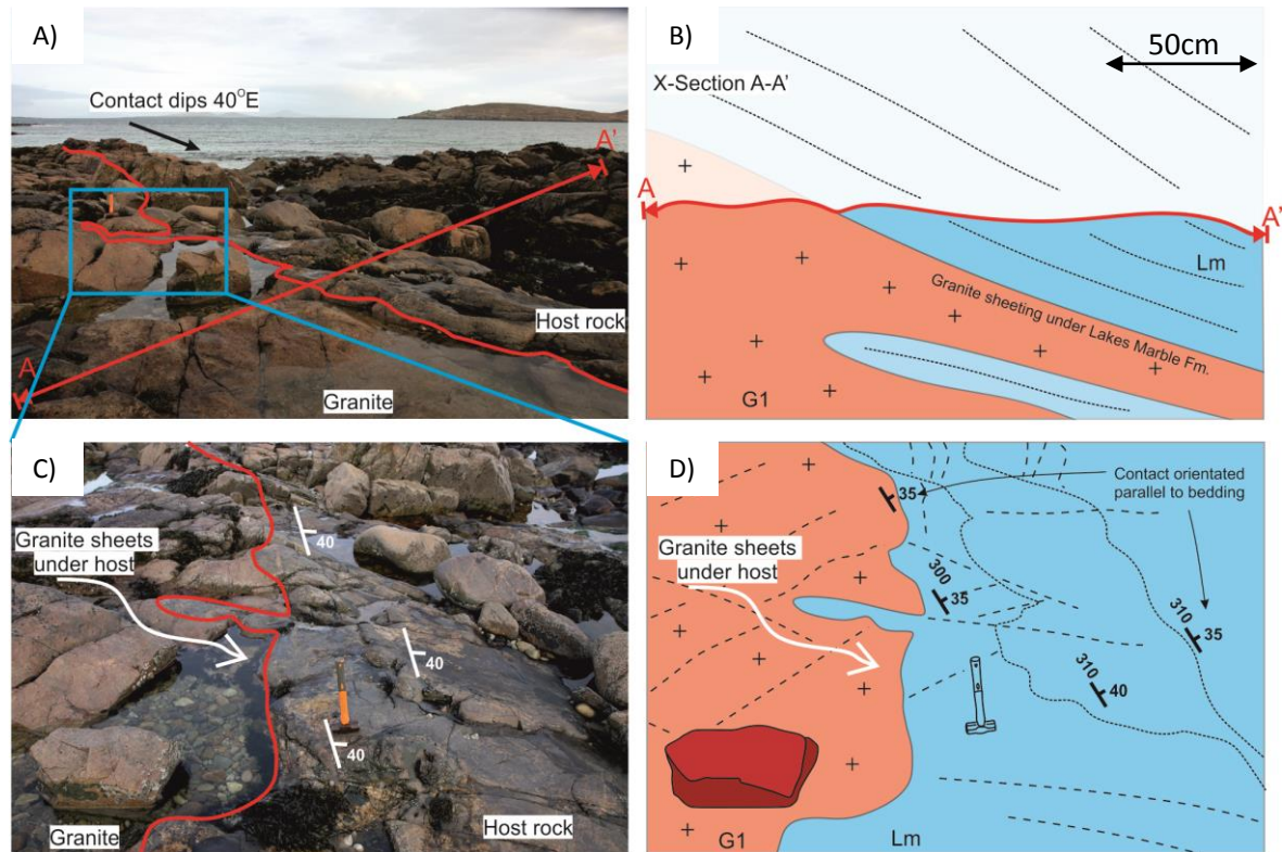
Fig. 7.7 A) The northern contact on Rossadillask beach (looking north), the granite contact dips to the east concordant to host rock bedding (Lakes Marble Fm., Lm). B) Cross section along A-A' of the sheeted contact. C) Blow-up area highlighted in blue in (A). D) A sketch of the Blown-up area in (C). Granite has emplaced into the Lakes Marble Fm. concordantly with the northward dipping limb of the Connemara Antiform.
