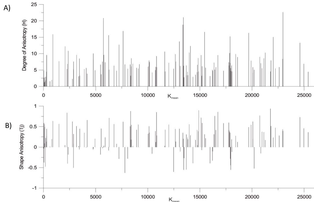
Fig. 9.16 A bar chart of the degree of anisotropy vs. K_{\text{mean}} (A) and shape anisotropy vs. K_{\text{mean}} (B) shows that even though a broad spectrum of susceptibility values are detected in different facies there is no systematic relationship between H or Tj and K_{\text{mean}} .
