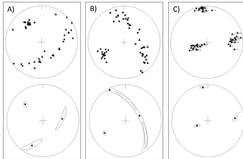
Fig. 7.29 Examples of different AMS tensor shapes depicted on southern hemisphere stereonet projections (individual sub-specimen susceptibility axes plotted above, mean susceptibility axes with 95% confidence ellipses below; square = K1, circle = K3, triangle = K2). A) A prolate fabric is defined when K1 is well constrained and K2 and K3 define a girdle. B) An oblate fabric is defined when K3 is well constrained and K2 and K1 define a girdle. C) Both a foliation and lineation may be determined when all axes are well constrained.
