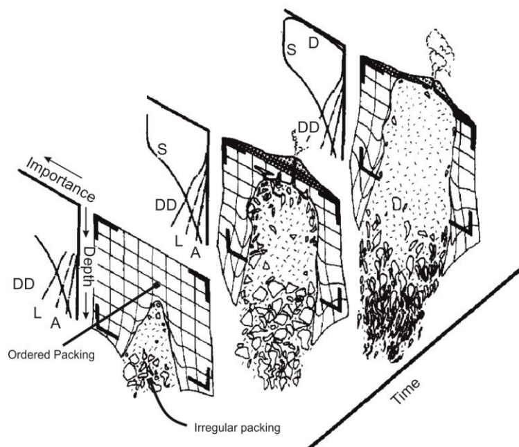
Fig. 1.12 Schematic diagram of a pluton ascending that heavily relies on the stoping mechanism (modified from Paterson and Fowler (1993)). The material transfer process at work varies from assimilation (A), rigid translation of wall-rock (L) and ductile shortening (DD) dominated at depth to stoping (S) and vertical displacement of overburden (D) in the brittle crust. Note that stoping re-deposits material in an inefficient fashion at the base of the diapir, this would ultimately cause arrest of magma ascent.
