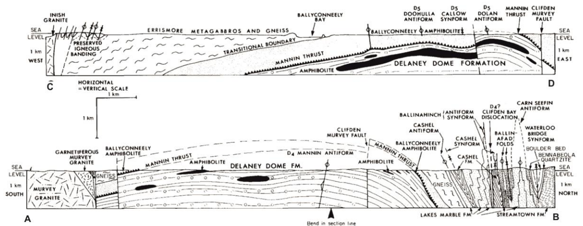
Fig. 3.11 Two cross sections across the Mannin Thrust (from Leake (1986)). Lines of section illustrated in Fig 3.10. X-sections show the Delaney Dome Fm. to be a footwall over which the CMC and been thrust via the Mannin Thrust.
