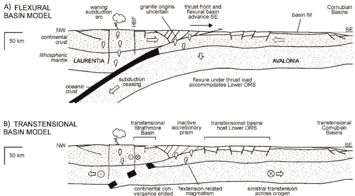
Fig. 2.9 Two contrasting models for the final stages of the soft docking of Laurentia and Avalonia (after Soper and Woodcock (2003)). (A) the classic flexural model proposed that convergence, i.e. transpression, continued after Iapetus closed until 410Ma. (B) Suggests regional transension (orogenic collapse) initiated by 420Ma soon after closure of Iapetus.
