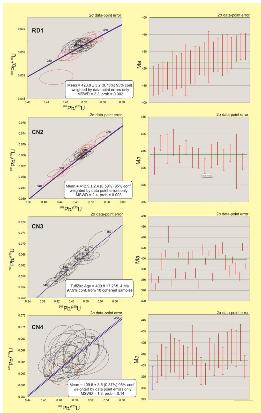
Fig. 9.7 Graphed Zircon U-Pb data. Red circles on isochron plots indicate rejected data points. All red points on bar charts were counted in calculated determined age.
