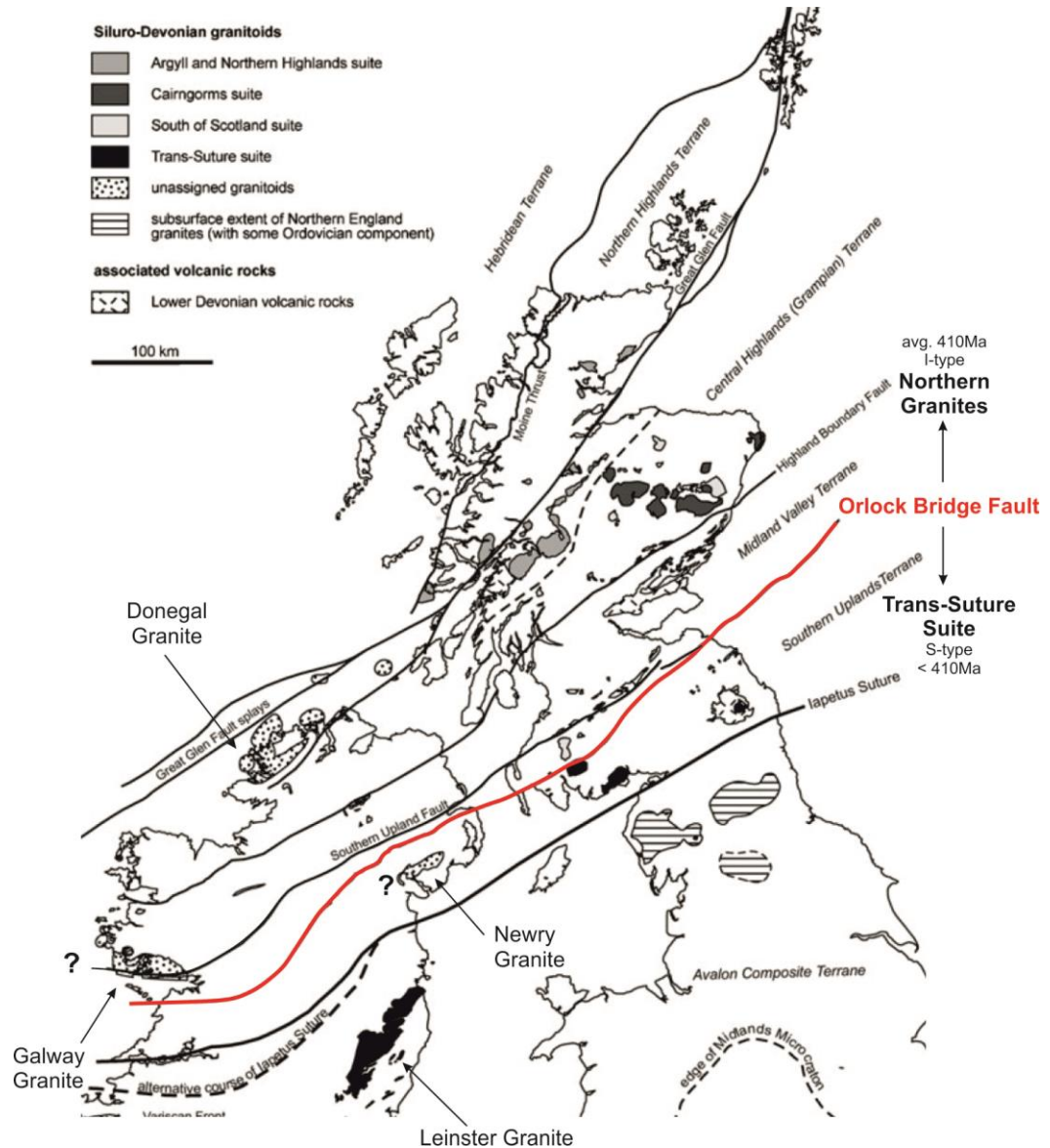
Fig. 4.1 Sub-classifications of the Newer Caledonian Granites and associated volcanics in Britain and Ireland (modified from Brown et al. (2008)). Note the position of the I-type Newry Granite south of the OBF and the Galway Granite north of the OBF.
