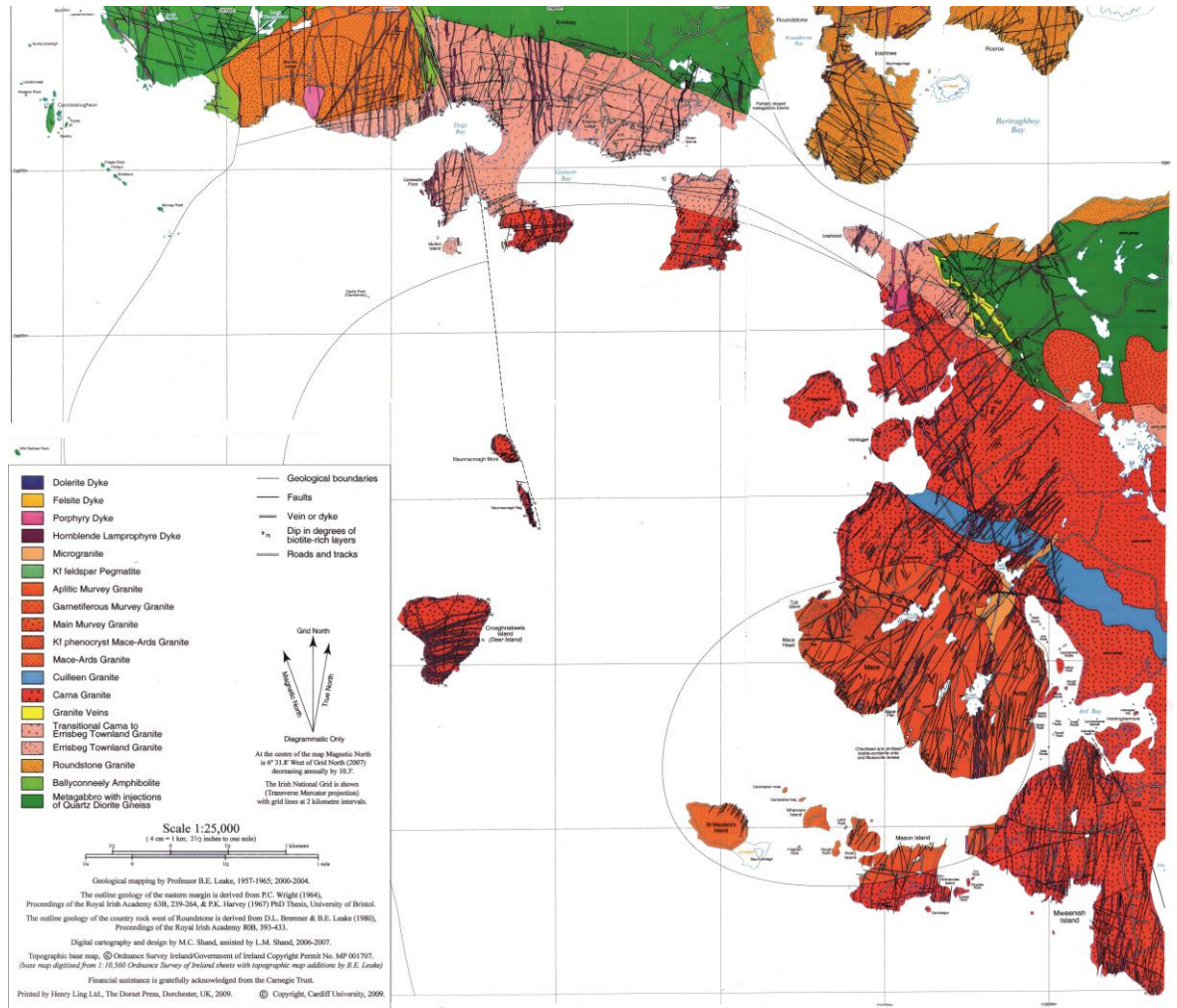
Fig. 5.3 Geological Map of the Carna Pluton (from Leake (2011)). This intrusion is interpreted by Leake (2011) as a central ring complex emplaced via stoping and without the influence of tectonic processes.
