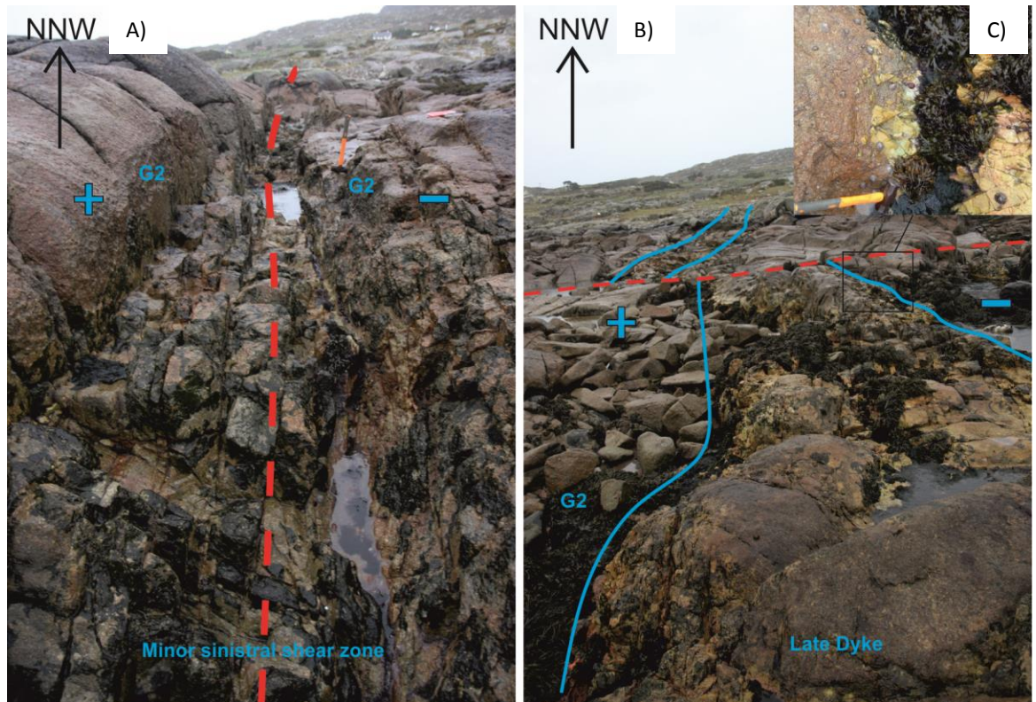
Fig. 9.4 A & B) Examples of NNW-SSE brittle shear zones which strike parallel to the Clifden - Mace Fault . In both cases late stage quartz/feldspar-phyric dykes have been emplaced into these faults. B) These dykes are cross cut by minor WNW-WSW faults after full crystallisation. C) Faulted margins are brecciated and angular fragments of the intruding rhyolitic dykes are included within the granite host.
