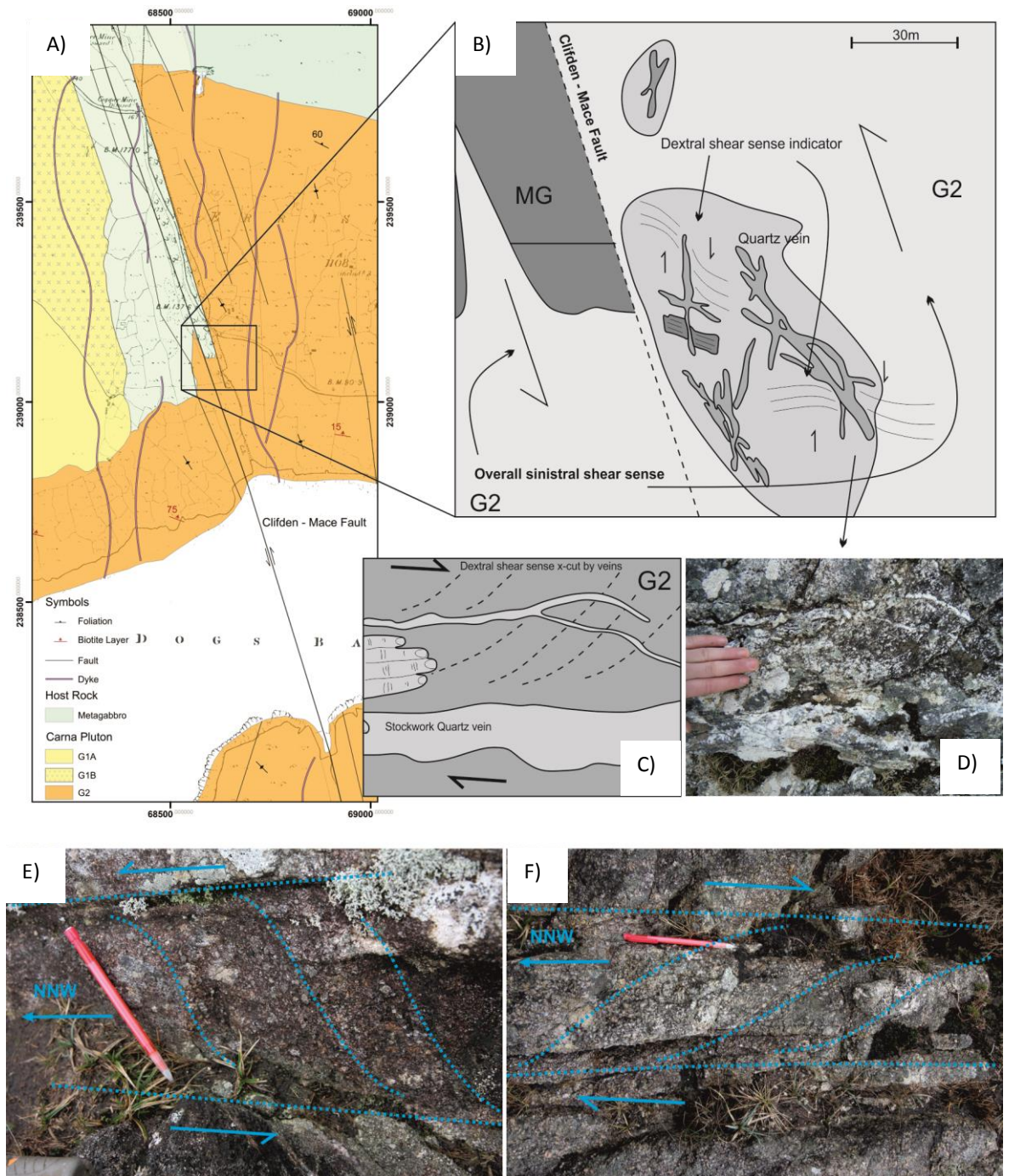
Fig. 9.5 Shear sense indicators along NNW-SSE faults in the Dogs Bay area. A) Overall 700m sinistral shear sense across the Clifden - Mace Fault. B) Sketch of outcrop adjacent to Clifden-Mace Fault, extensive stockwork quartz veins and brecciation is associated with faulting, several examples of dextral shear sense is noted within this zone (C & D). Further to the northeast on the southern side of Errisbeg several ductile NNW-SSE shear zones are noted, both dextral and sinistral shear sense indicators are present, lack of brittle deformation and in some cases aligned tabular feldspars indicate shearing was active in the submagmatic state (E & F).
