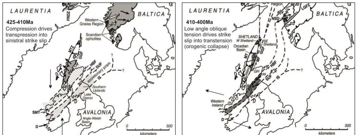
Fig. 2.11 Transition between regional sinistral compression and tension denotes the end of the Caledonian Orogeny (from Dewey and Strachan (2003)).
