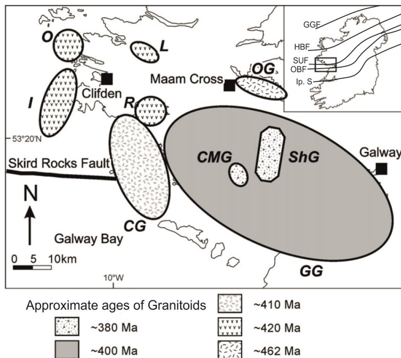
Fig. 4.3 Distribution of Siluro-Devonian plutons in Galway and approximate ages determined (Feely et al. 2010). Note that all intrusions are sited north of the Orlock Bridge Fault but a broad range of isotopic age determinations have been reported which are inconsistent with the petrogenetic models discussed in the text.
