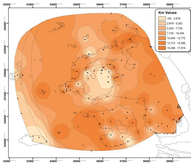
Fig. 7.25 A contour map of K_{\text{mean}} susceptibility values in the Omev Pluton. A low magnetic susceptibility anomaly is centred over the localities where G3 is mapped. Negligible differences are detected between G1 and G2.
