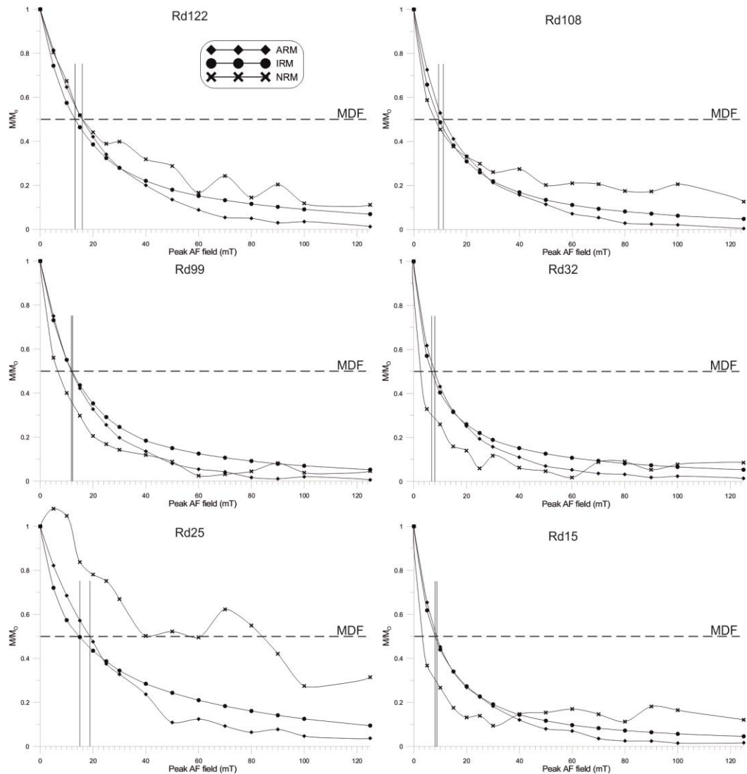
Fig. 8.15 Graphed data from the modified Lowrie-Fuller test. Irregular demagnetisation of NRM in RD25 may reflect TRM or NRM interference due to heat or fluid convection during emplacement of the Carna Pluton.
