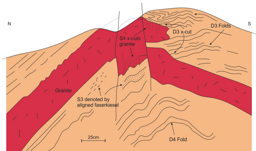
Fig. 3.7 Sketch of the structural relationship between D3 and D4 folding and minor Oughterard Granite sheets (redrawn from Tanner et al. (1997)). Granite cross cuts D3 folds and intrudes concordant to D4 folds but exhibits subtle S4 cleavages which show emplacement and folding was concomitant.
