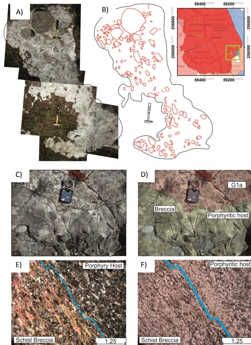
Fig. 7.12 A) Representative images of the Barnahallia Breccia. B) Outline of breccia clasts shows a crude NNW-SSE preferred orientation, breccia clasts are not completely randomly orientated. This breccia is not hosted directly in the G1a but instead is suspended within a porphyritic microgranite which exhibits sharp contact with the surrounding G1a (C & D). E & F) XPL and PPL images of a contact between the fine grained porphyritic microgranite host and a breccia clast (in this case a schist). It can be concluded from this preliminary work that this not an "explosion breccia" hosted within the G1 facies.
