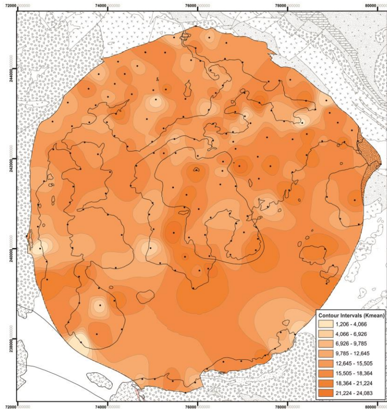
Fig. 8.18 Contour map of K_{\text{mean}} values. No major fluctuation is observed indicating a reasonably homogenous assemblage.
