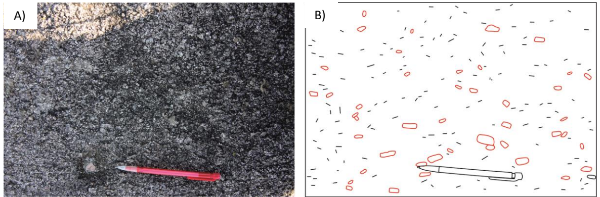
Fig. 7.14 A) An example of a typical magmatic foliation observed in the Fountainhill area. B) A trace of the same image demonstrates the presence of a foliation predominantly defined by K-feldspar and biotite.
