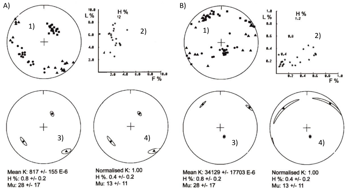
Fig. 6.8 A & B) AMS data from two independent samples (from Owens (2000a)). In both cases (1) shows principal axis directions for all sub-samples. 2) is a Flinn plot of the same data. 3) shows the un-normalised mean principal susceptibility axes for the compiled data with a 95% confidence ellipse. 4) is the normalised mean principal susceptibility axes for the compiled data with a 95% confidence ellipse. Note in sample (A) normalised and un-normalised projections are essentially identical but in (B) they differ. This shows the averaged AMS tensor in (B) is complex and many contain a sub-fabric and that of (A) is relatively straight forward.
