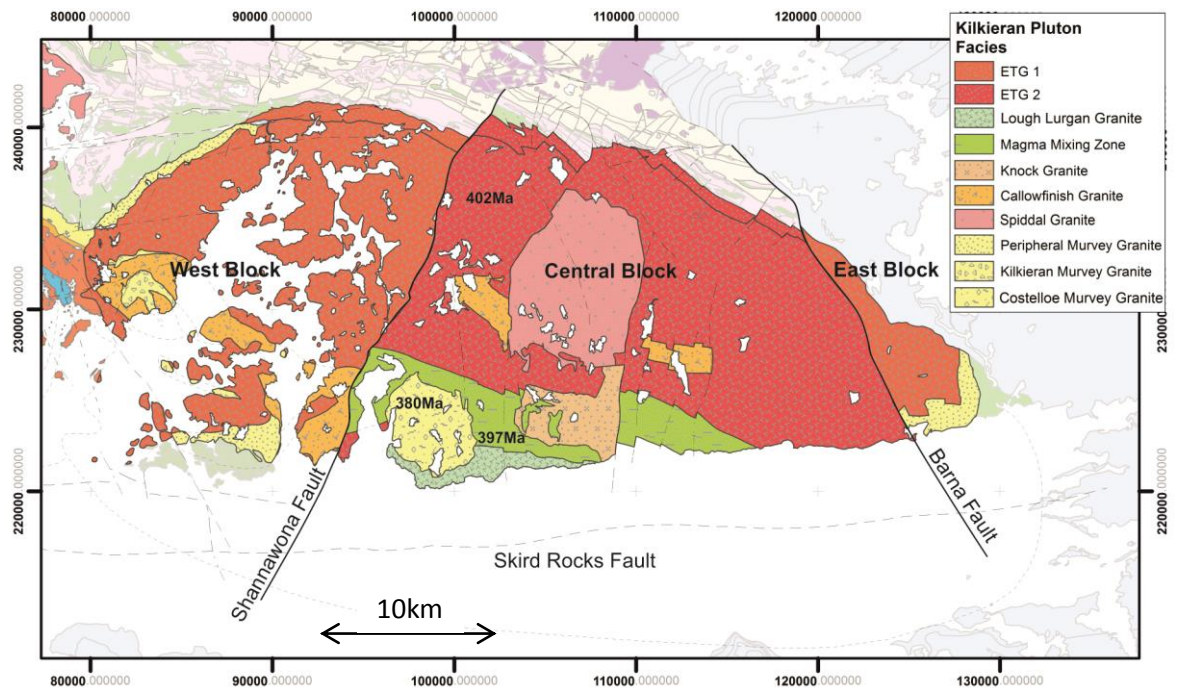
Fig. 5.4 Map of the Kilkieran pluton illustrating the fundamental structure and cross cutting relationships established by the authors referred to in the text. Map redrawn based on Long and McConnell (1995b) and the work referred to in the text. Geochronology shows oldest and youngest constituents of the Kilkieran Pluton as well and the age of the MMZ (from Feely et al. (2003)).
