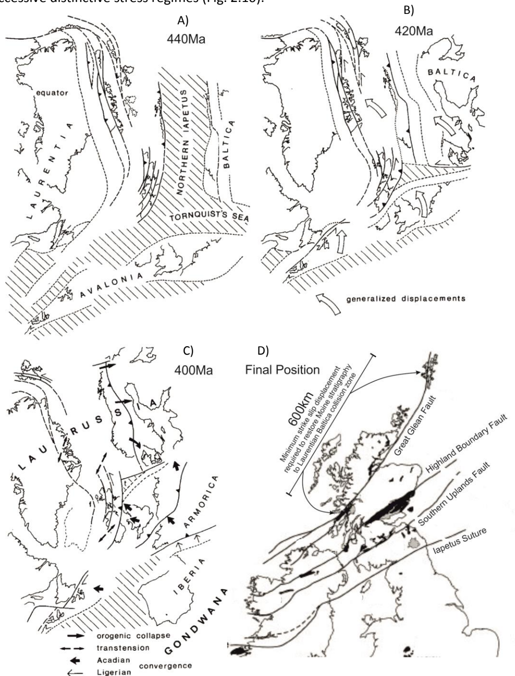
Fig. 2.10 Late Caledonian final closure of Iapetus (after Soper et al. (1992)). In this model the Iapetus Ocean is closed by 420Ma (A & B). Regional sinistral strike slipping along major Caledonian faults persists up to 400Ma (C) to juxtapose contrasting terrane blocks in Britain and Ireland (D). This model shows transpression persists after 420Ma and, in contrast to Fig. 2.6 also shows the Tornquist Sea remain open into the mid Silurian.
