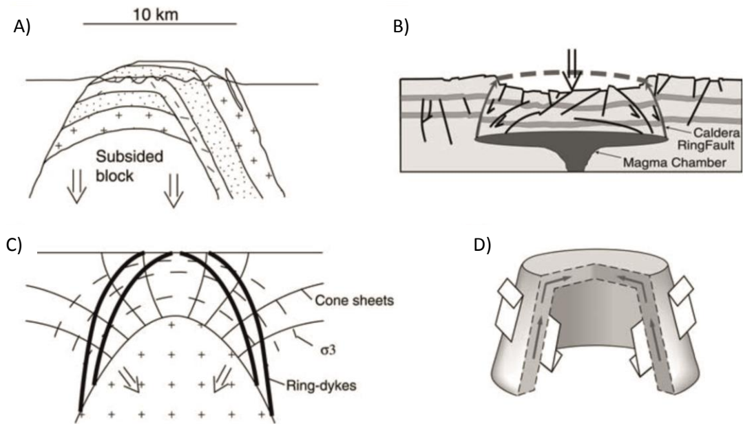
Fig. 1.11 A) The cauldron subsidence model for the Eastern Mourne Granites (Stevenson et al. 2008b). B) The emplacement of ring dykes (O'Driscoll et al. 2006). C) Cone sheets (Bailey et al. 1924). D) Shear sense and magma flow direction within ring dykes (O'Driscoll et al. 2006).
