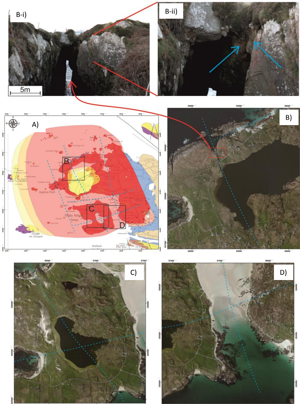
Fig. 7.17 Abrupt topographic lows cross cut the Omev pluton (A). These lows are associated with scarps (B), caves (B-i), lakes (C) and bays (D). In some cases minor brecciation is observed (B-ii).
