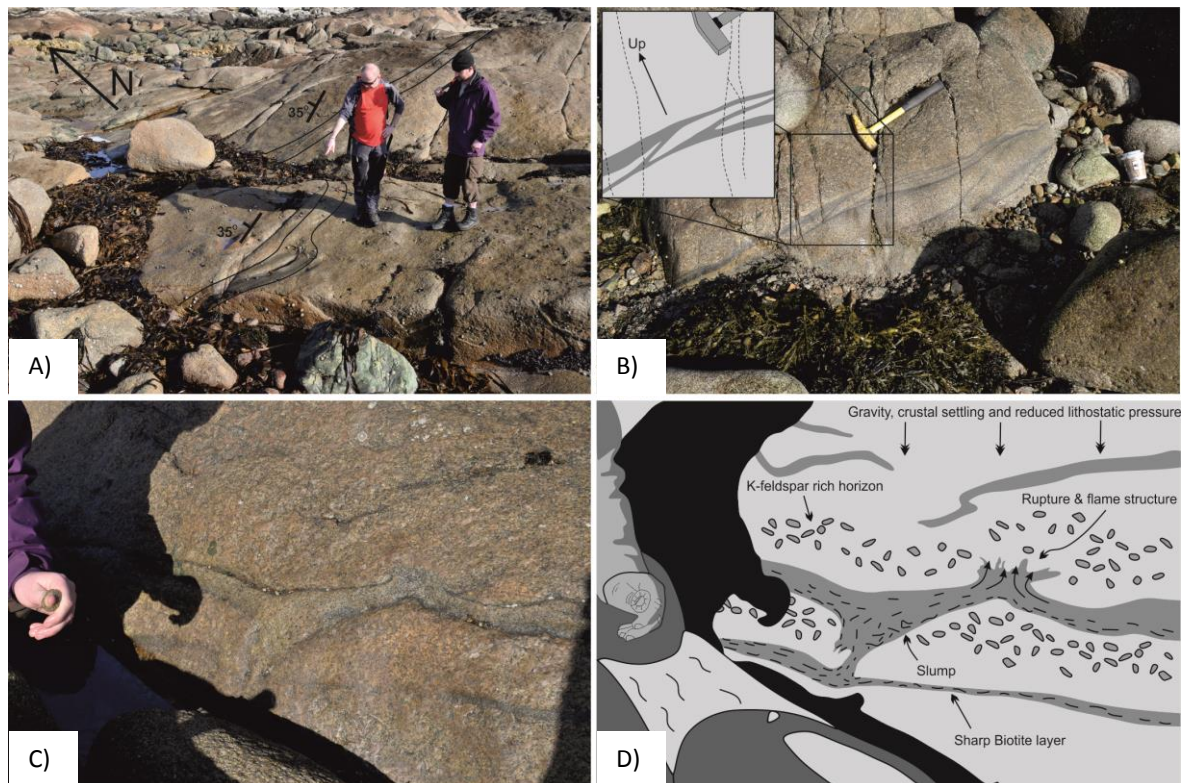
Fig. 9.2 A) Northward dipping biotite layers at Dogs Bay. B) Cross bedding identified in fractionated biotite layers. C & D) Biotite and K-feldspar modal layering disrupted by slumping and flame structures.
