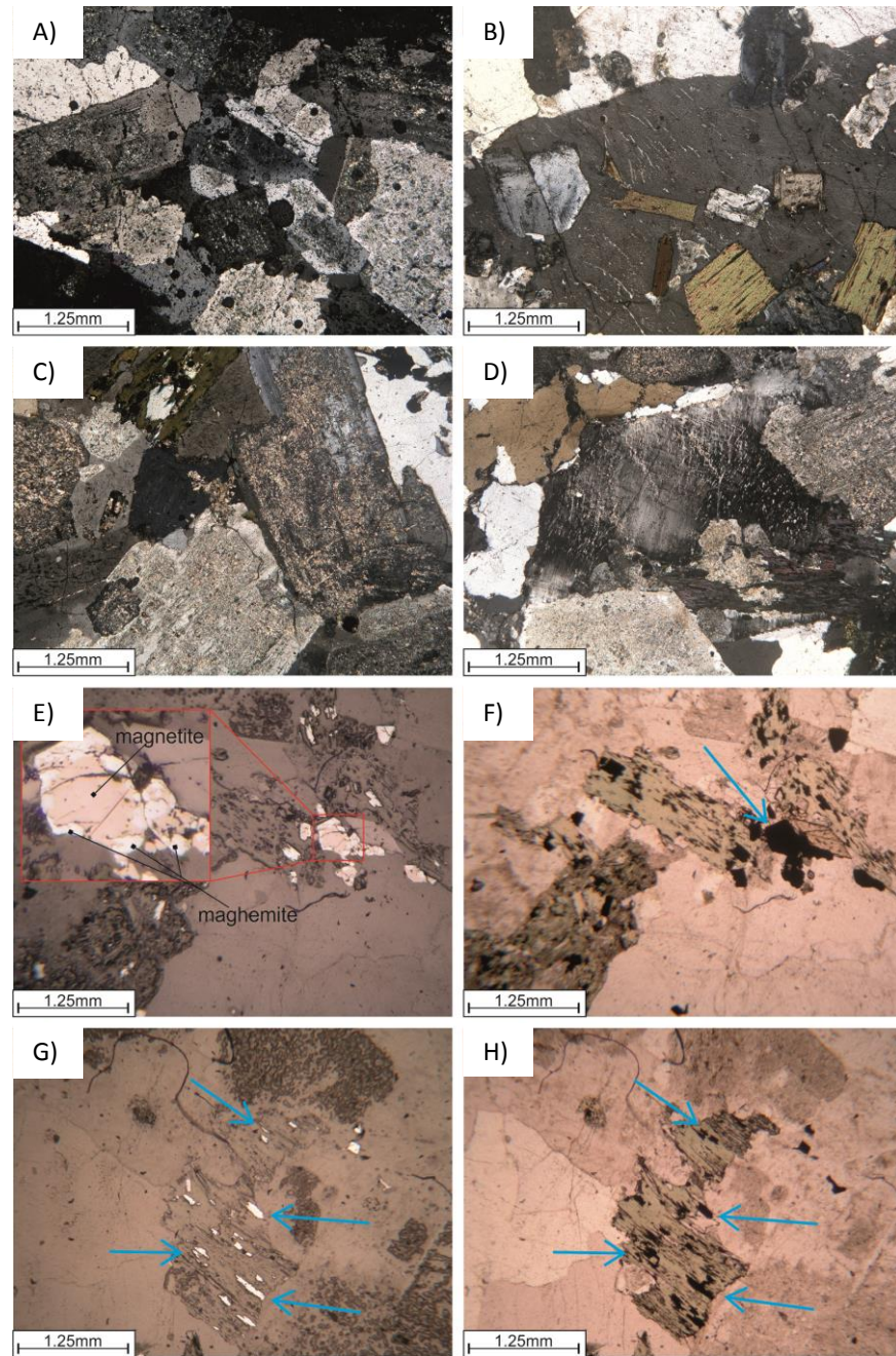
Fig. 8.6 Typical petrography of G1. Medium grained granodiorite, occasional perthitic K-feldspar with included feldspar and biotite (A & B), euhedral weakly normally zoned feldspars with calcic cores and anhedral quartz (C & D). Reflected light and PPL views (E-H) of biotite that hosts a disproportionate amount of magnetite. This can be associated with incorporation of magnetite into the biotite cleavage during crystallisation and deuteric alteration of biotite Dunlop and Ozdemir (1997). E) Periphery of maghemite oxidised to magnetite.
