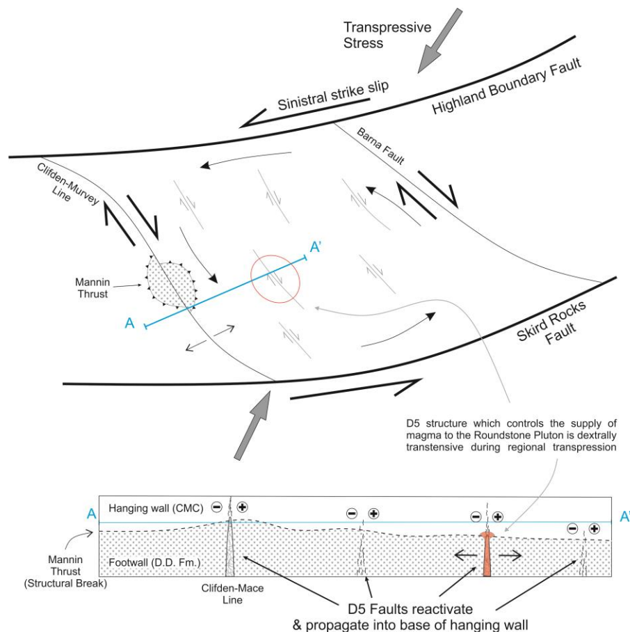
Fig. 8.25 Schematic model of the relationship between regional stress, local structure and magma transport. The terrane bound by the Skird Rocks Fault and Highland Boundary Fault acted as a large scale deformation zone. Anticlockwise rotation of blocks bound by NNW-SSE faults generated localised dextral transtension long these shear zones. These faults provided vertical ascent conduits for ascending magma which was capped by the Mannin Thrust stress barrier at the site of emplacement.
