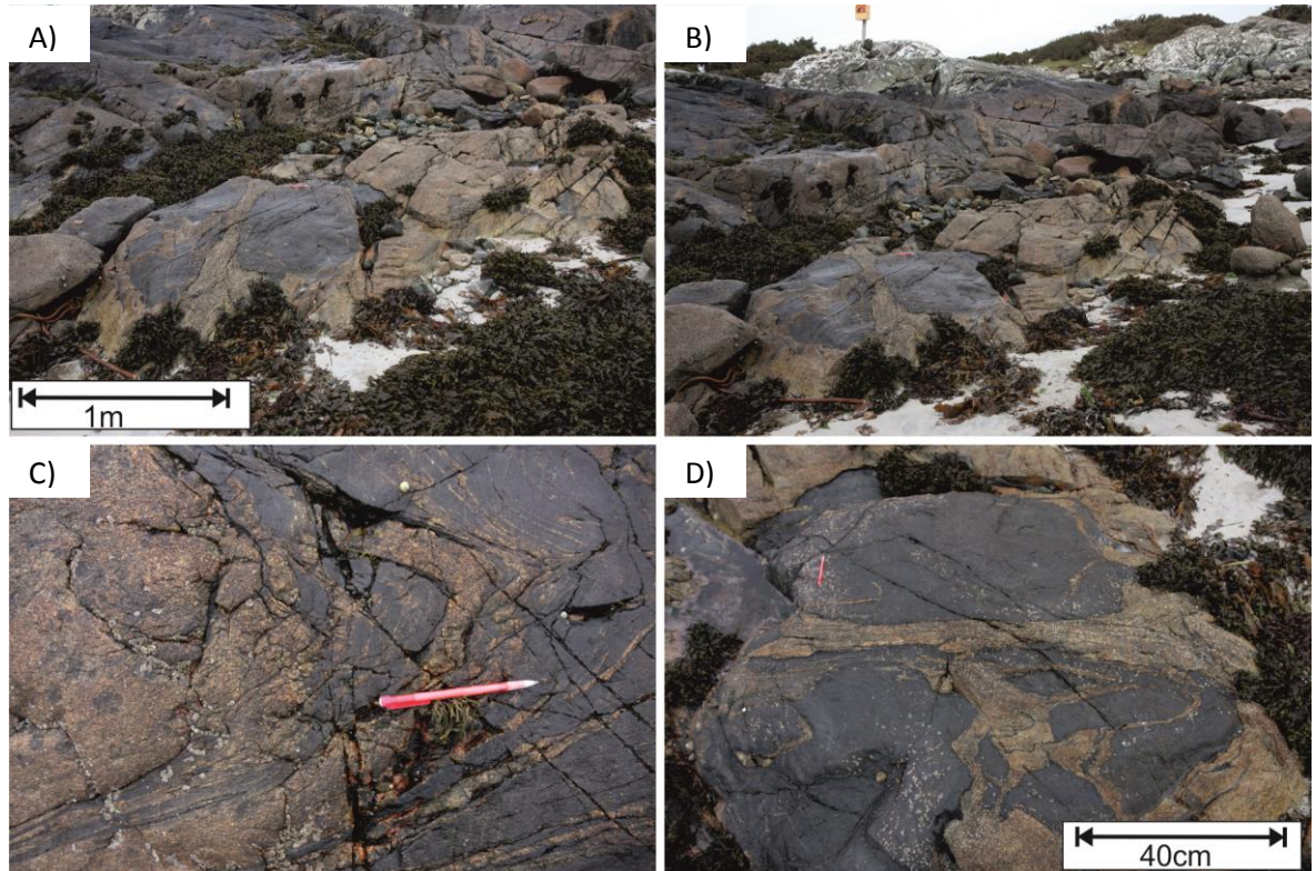
Fig. 8.4 Examples of stoped blocks and the relationship shared between country rock structure and the intruding granodiorite. Overall, the pluton is discordant relative to host rock structure (A & B) but locally intrudes along the tectonic fabric associated with D3 folding in the CMC (C & D).
