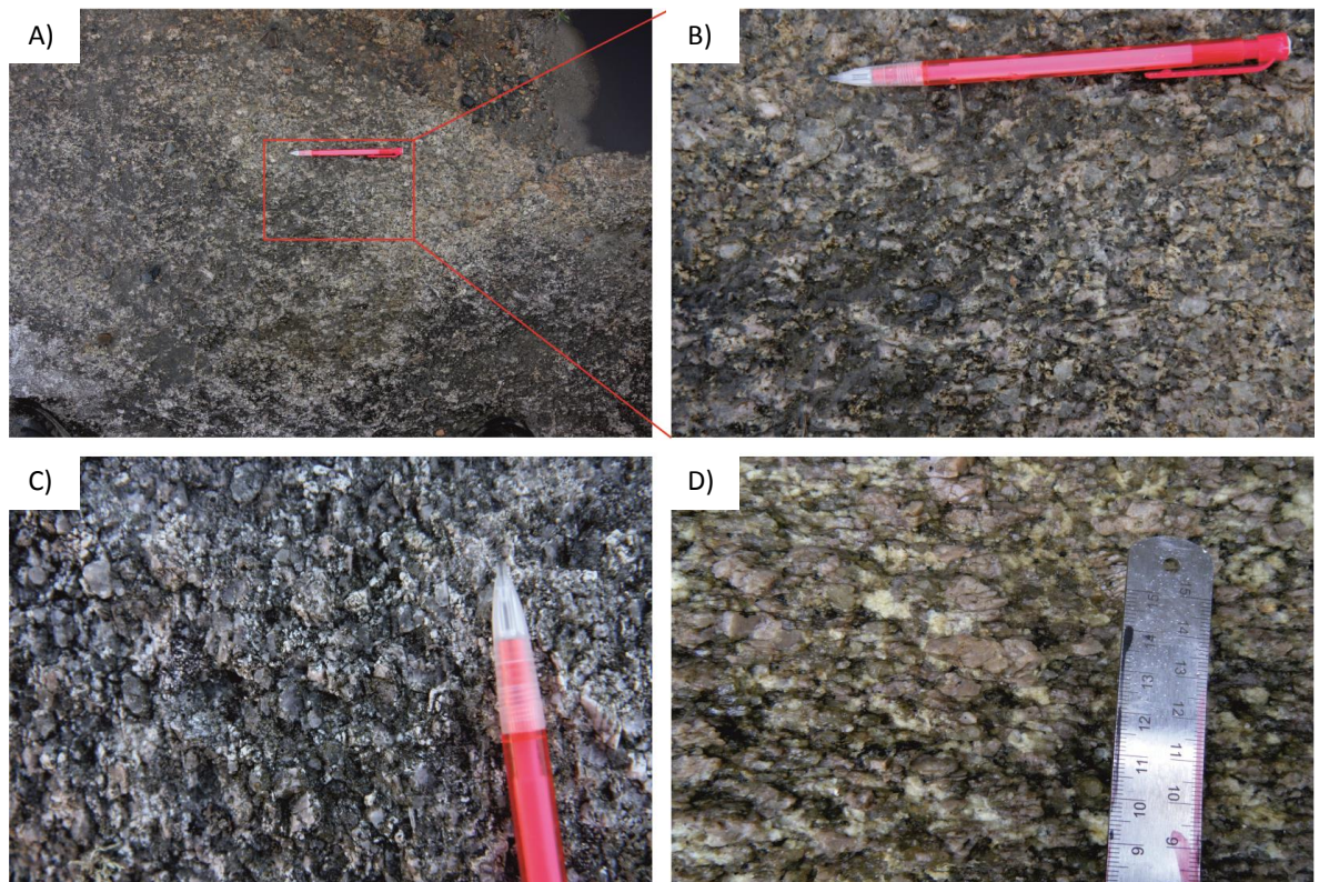
Fig. 7.18 Fabric development within a NNW-SSE shear zones mapped at Aughrus Point. A & B) On the periphery of the shear zone a definite petrographic fabric is observed, this is defined by elongate quartz and smeared biotite. An apparently strong foliation is observed within the shear zone (C). Close inspection reveals a moderate petrographic foliation that parallels fine scale micro fracturing which give rise to a strong textural anisotropy (D).
