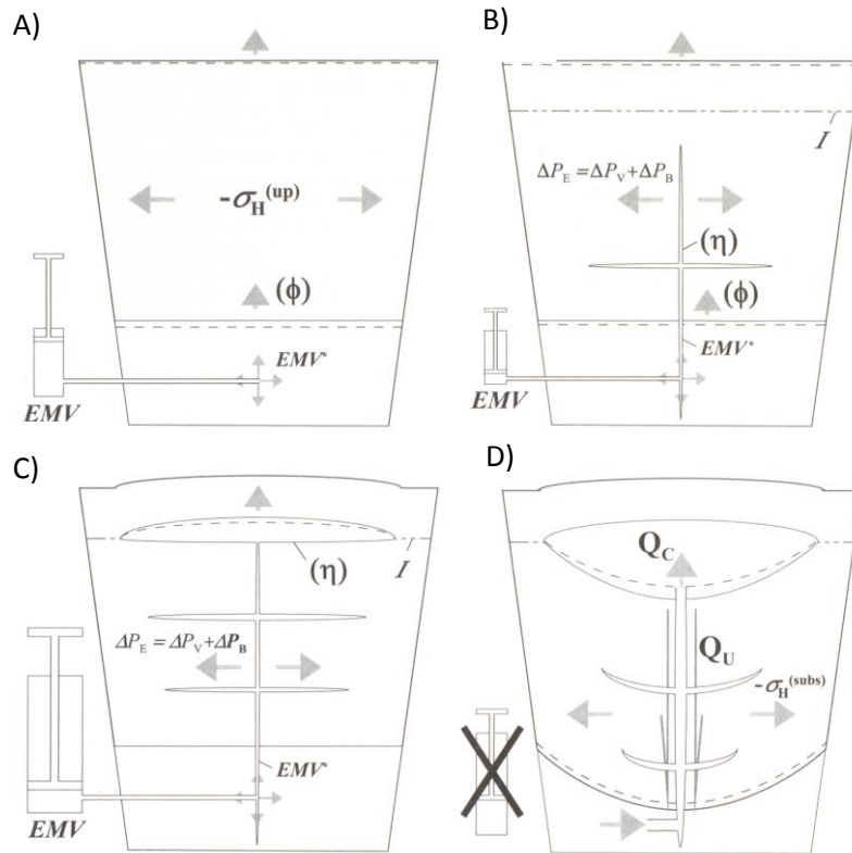
Fig. 1.4 Fracture-mediated intrusion model driven by Excess Magma Pressure as proposed by Ablay et al. (2008). A) Pre-rupture stresses. B, C & D) Low and high EMV (excess magma volume) and buoyancy pumping regime generate distinct conduit morphologies i.e. sills and dykes, Christmas-tree laccolith and a lopolith respectively. Q_C ; conduit flux, Q_U ; under-burden flux, -\sigma_H ; horizontal (confining) stress, \phi ; Coefficient of EMV relaxation by inelastic deformation, \eta ; Coefficient of EMV relaxation by crack growth.
