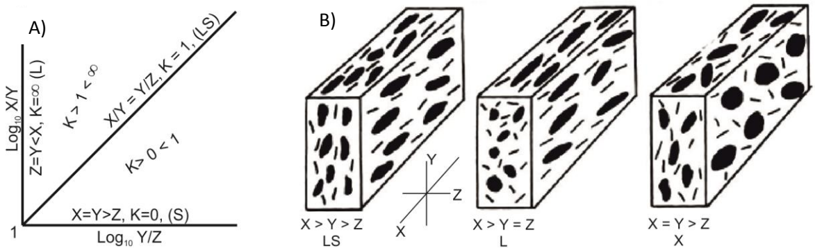
Fig. 6.4 Graphical representation of the possible symmetry of the strain ellipsoid based on the Flinn diagram (A) and associated rock fabrics (B) (from Hutton (1988a)). X, Y and Z are the max, intermediate and minimum strain axes of a strain marker, L= prolate fabric, S = oblate fabric, LS = triaxial ellipsoid or fabric with both lineation and foliation. A higher H value (Ramsay and Huber 1983) is equivalent to greater distance from the origin (1) on the Flinn plot.
