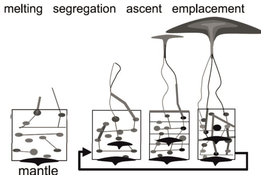
Fig. 1.1 The four fundamental processes, melting, segregation, ascent and emplacement, involved in granite generation (from Vigneresse (2005)). The four stages are discrete and may occur episodically or continuously during a protracted tectonic event. In this paradigm the mantle represents a fifth factor, that of a heat source and chemical reservoir.
