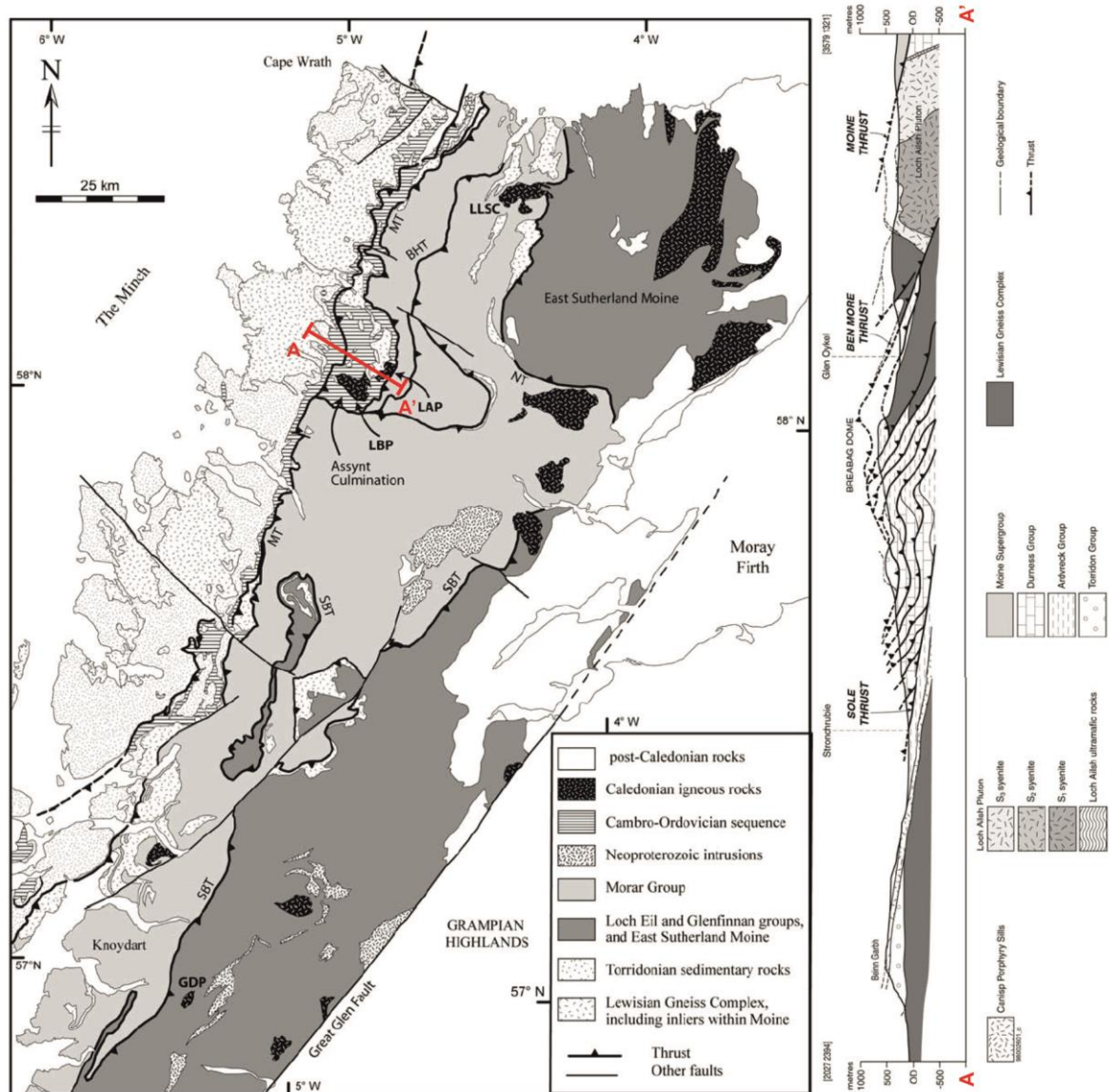
Fig. 2.8 Geological map of the Scottish highlands and more detailed x-section of the classic Assynt area (from Goodenough et al. (2011), after BGS (2007)). The Lewisian Gneiss Complex, Torridonian and Cambro-Ordovician strata unconformably overlie each other in that order west to east. The Moine Thrust Zone (MT) overlies and has thrust the early Neoproterozoic Moine Supergroup westward. Several stacked thrusts define the MT, these are uniquely exposed in the Assynt area (x-section). Correlation of thrust sheets with foreland sequences (Lapworth 1883) reveals a piggy-back thrust sequence which propagates toward the foreland (Coward 1985). Thus the structurally highest unit is actually the oldest. BHT, Benn Hope Thrust; NT, Naver Thrust; SBT, Sgurr Beag Thrust; GDP, Glen Dessarry Pluton; LBP, Loch Borralan Pluton; Lap, Loch Ailsh Pluton; LLSC, Loch Loyal Syenite Complex.
