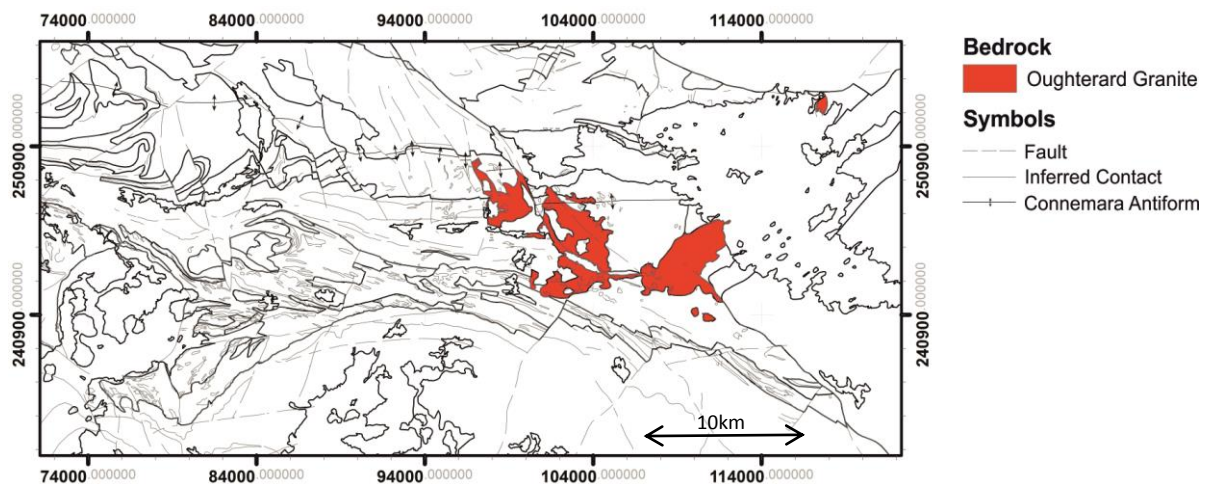
Fig. 3.6 Location of the three main bodies of Oughterard Granite in Connemara.
