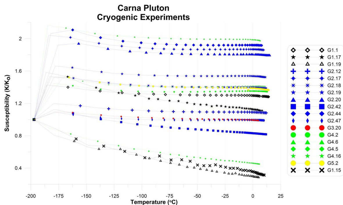
Fig. 9.10 Graphed results of cryogenic low field susceptibility experiments. Only three samples do not show a defined Verwey Transition (G1.15, G1.19 and G4.5) which indicate the paramagnetic fraction may heavily influence the AMS tensor.
