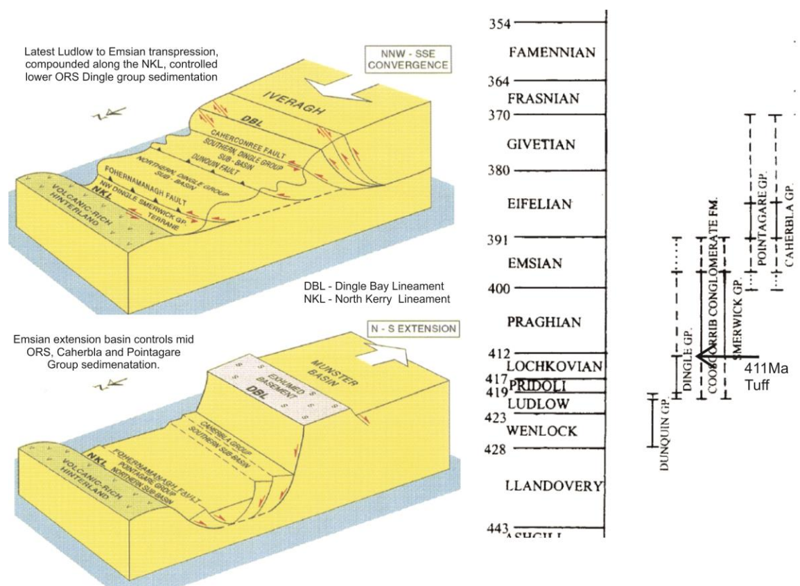
Fig. 2.14 Late Silurian - mid Devonian evolution of the Dingle Basin (from Richmond and Williams (2000)). This work shows regional transpression continued into the early Praghian and this stress field is associated with ORS basin development in this area.
