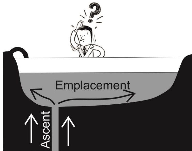
Fig. 1.2 Fundamental distinction between Ascent and Emplacement
