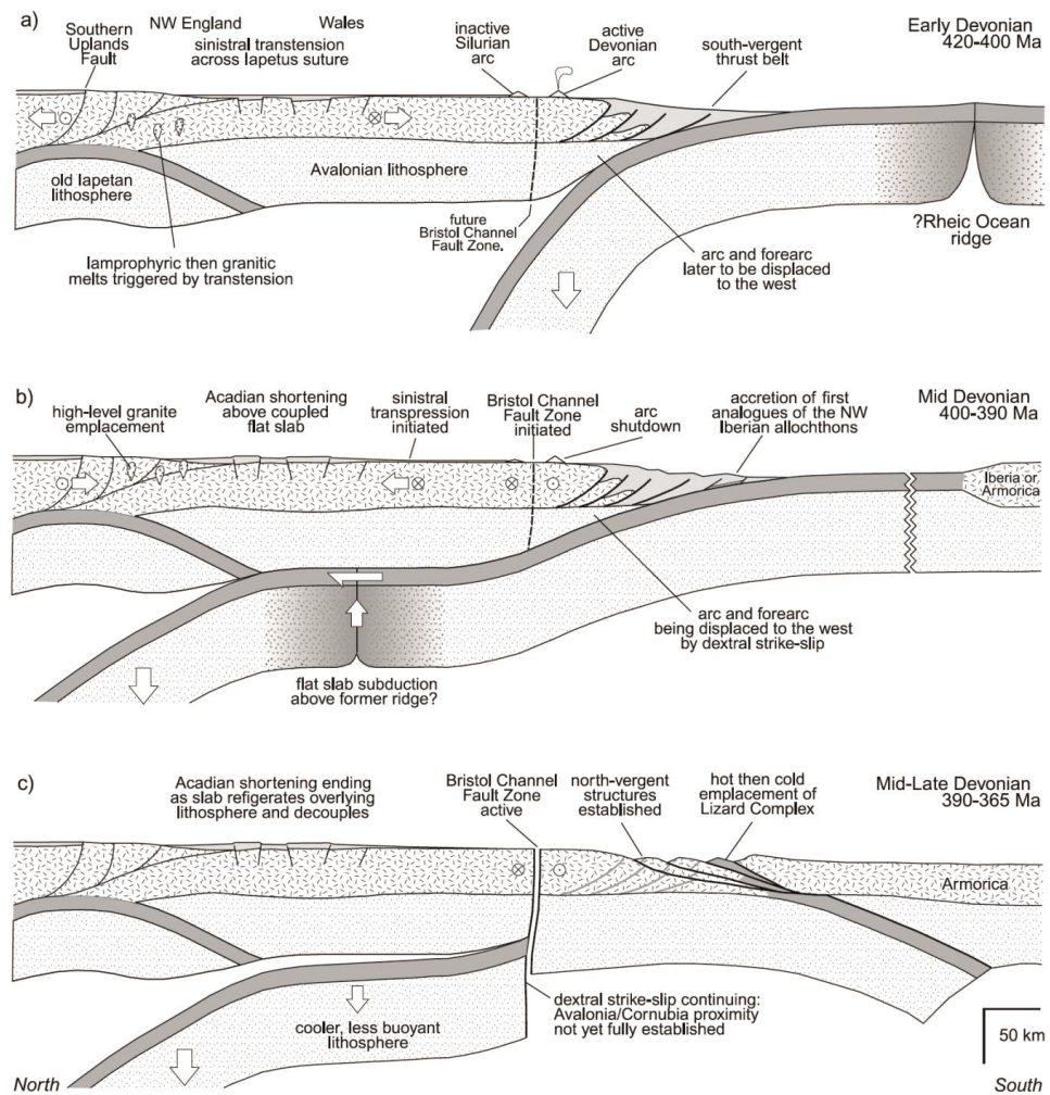
Fig. 2.15 Cross section of the convergence of Armorica with the southern margin of Avalonian during the Devonian (from Woodcock et al. (2007) after Soper et al. (1992)). The Acadian Orogeny was not an Iapetus margin process and therefore not a part of the Caledonian Orogeny. Following subduction, the Rheic Ocean crust under-plates much of the Caledonian terranes. Such a process would have promoted new melting and magmatism in that same terrane.
