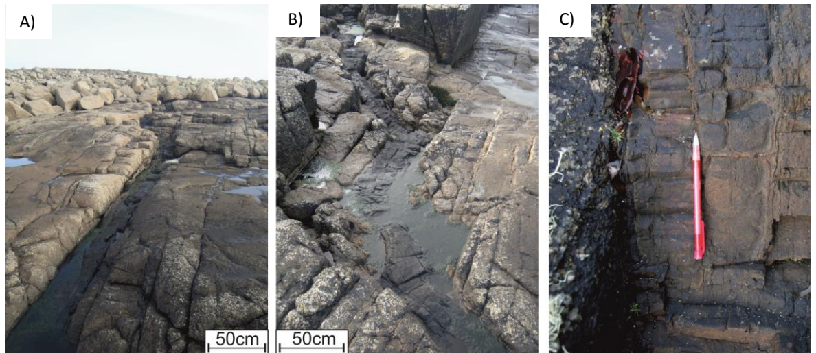
Fig. 7.13 Typical examples of Carboniferous dolerite dykes in the Omey Pluton. These typically zig-zag through the granite as they follow joint sets (A & B). All exhibit chilled margins (C).
