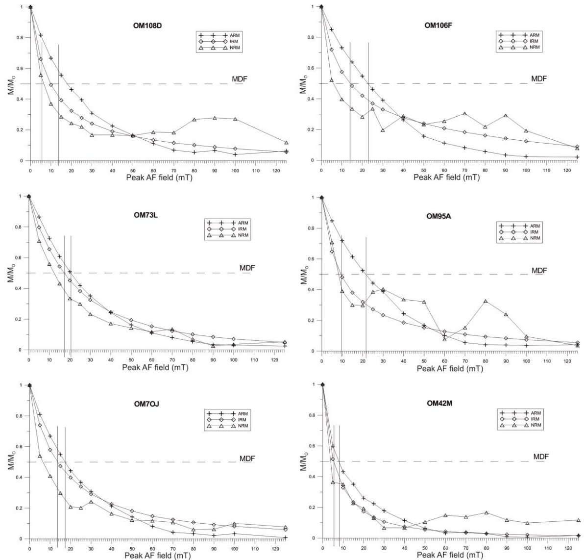
Fig. 7.22 Results of Lowrie-Fuller test as discussed in the text.
