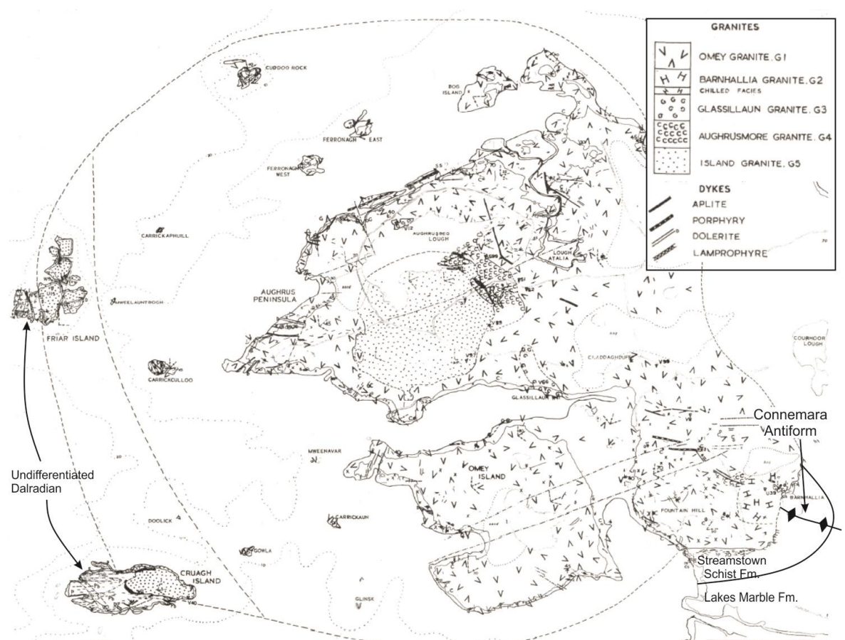
Fig. 5.2 Map of the Omev Pluton after Townend (1966). The longest axis of the pluton is parallel to the D4 Anticline and the Island Granite forms a "central plug".
