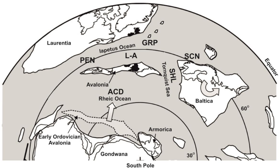
Fig. 2.4 Schematic diagram of the Iapetus Ocean during early closure (~Ordovician) modified from Woodcock and Strachan (2012). Locations of orogenic phases discussed in the text are indicated: PEN = Penobscotian, GRP = Grampian arc system, SHL = Shelveian closure of Tornquist Sea, SCN = Scandian Baltica - Laurentia collision, L-A Laurentian - Avalonian convergence, ACD = Acadian Orogeny closure of the Rheic Ocean. Gray arrows indicate direction of movement of Avalonian and Baltica during closure of Iapetus.
