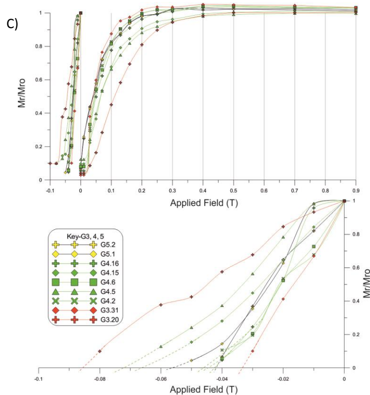
Fig. 9.14 Graphed results of SIRM and BIRM experiments. A) G1 facies return higher coercivity values than G2 (B) or G3, G4 and G5 samples (C).
