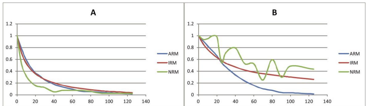
Fig. 6.11 Examples of data from the Lowrie-Fuller test carried out on two contrasting samples. In sample "A" rapid demagnetisation of ARM, IRM and NRM is consistent with the presence of magnetically soft minerals such as multidomain magnetite. Sample "B" demagnetises at a much slower rate. IRM is much more stable than ARM and the NRM demagnetisation curve contains several peaks and troughs. This is consistent with the presence of magnetically hard minerals such as haematite or single domain magnetite.
