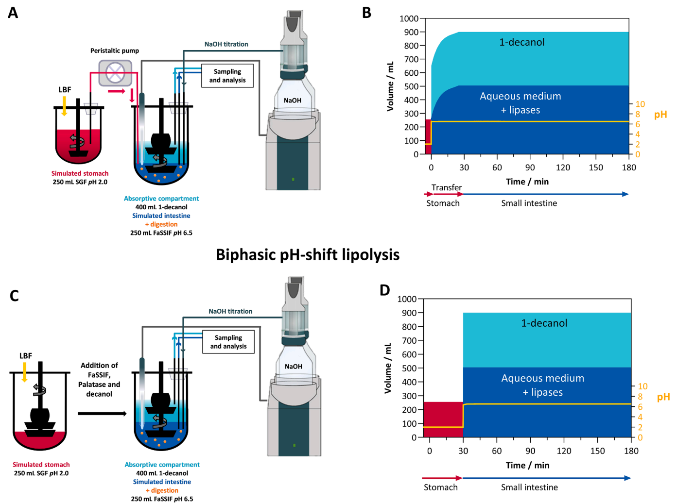
Fig. 1. Schematic representation of experimental setups A + B: The biphasic gastrointestinal transfer lipolysis setup. A is a schematic representation, including a peristaltic pump to transfer simulated stomach medium into simulated intestinal medium. B: Dissolution procedure: starting with 5 min dispersion in SGF, then the transfer into 250 mL of FaSSIF with 400 mL of decanol. C + D: The biphasic pH-shift lipolysis setup. C: The biphasic pH-shift lipolysis setup. D: Dissolution procedure: starting with 30 min dispersion in SGF, then the addition of 250 mL of FaSSIF and 400 mL of decanol. Dissolution procedures are adapted from Brenner et al. (2024).
