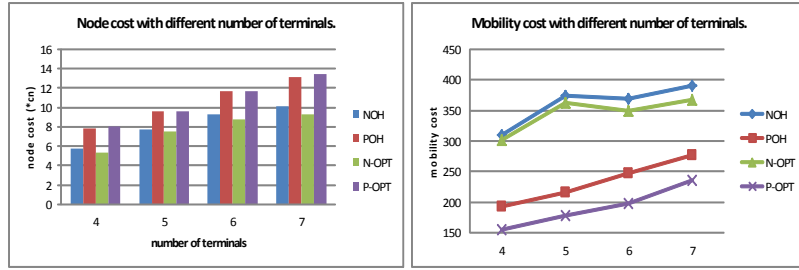
Fig. 4. Varying number of terminals
