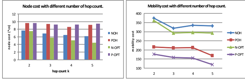
Fig. 5. Varying hop count limit k .
