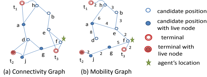
Fig. 1. Example Network Repair Problem
