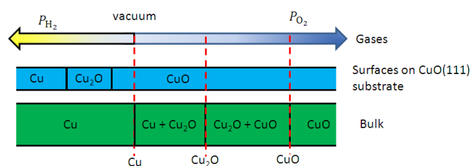
Fig. 8 Schematic phase diagram of CuO(111) reduction to metallic Cu under different oxygen and \text{H}_2 pressures. green and blue colours represent bulk and surface, respectively.
