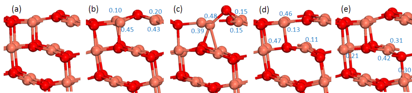
Fig. 3 Optimized structures of (2 \times 1) -CuO(111) surface with an oxygen vacancy on the surface and subsurface. (a) stoichiometric CuO(111) (b) V_{O(3)} (c) V_{O(4)} (d) V_{O(u)} (e) V_{O(d)} . Changes in Bader charge ( e^- ) relative to (a) are shown for Cu atoms.
