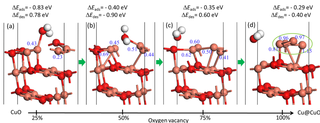
Fig. 6 Structure of the CuO(111) surface after adsorption of each \text{H}_2 molecule and formation of water, The adsorption energy of \text{H}_2 on the surface ( \Delta E_{\text{ads}} ) and desorption energy of water from the surface ( \Delta E_{\text{des}} ) are shown on the top of each subfigure. The arrows in green represent the removal of formed water molecule and introducing another \text{H}_2 on the partially reduced surface. The arrow in the bottom indicates the trend of reduction. Changes in Bader charge ( e^- ) relative to Fig. 4(a) are shown for Cu atoms in the top layer.
