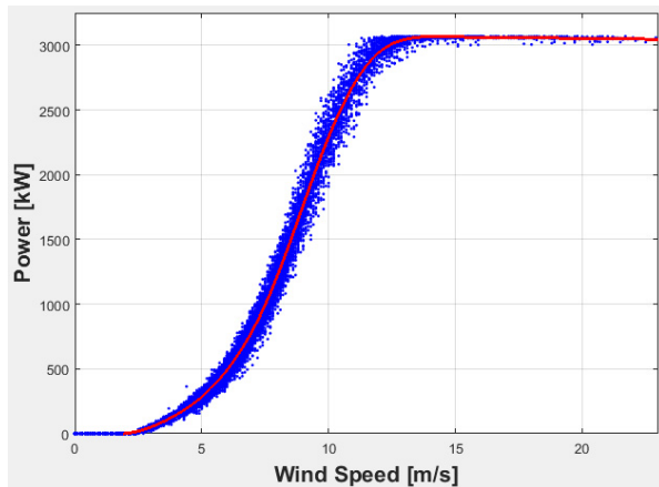
Fig. 2. Smoothing spline wind turbine power curve fitting.
