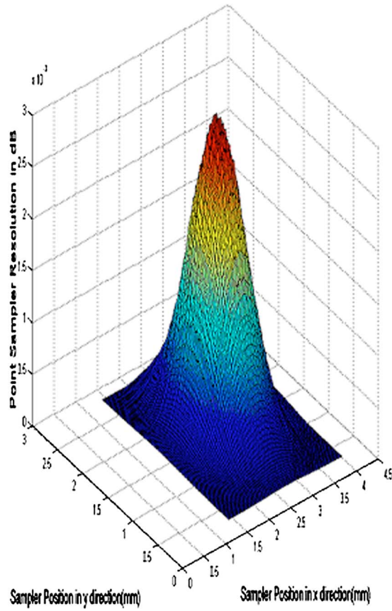
FIG. 5. (Color online) Plot showing the resolution of individual spatial samplers in the DMD™ that are used for VOA super-resolution controls. Equation (8) is used to generate this data.
