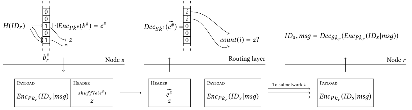
Figure 3: Operation of the private routing protocol. Node s wants to securely transmit message msg to node r . Node r belongs to subnetwork i , but s only knows r 's ID ( ID_r ). Communication proceeds as follows: s generates the SBF related to ID_r and counts the number z of non-zero values in it; the filter is then multiplied (through an homomorphic encryption operation) by the shared encrypted filter b^# . The resulting filter is then sent to the routing layer, together with z . The routing layer decrypts it, and computes the destination subnetwork i . The payload (that is, the encrypted message) is then routed to the subnetwork i and node r , either through a gateway or by broadcast. r receives the message and decrypts it.
