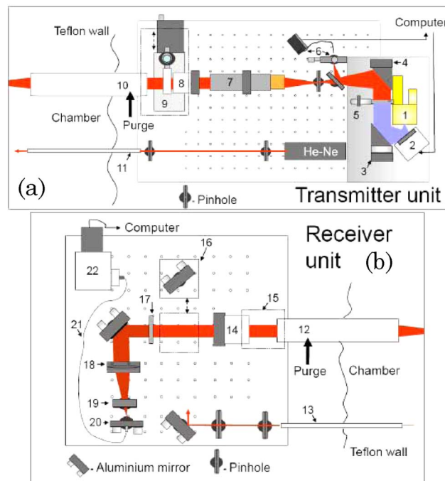
Fig. 1. (Color online) (a) Transmitter unit: 1, short-arc Xe lamp; 2, piezo-mounted plane mirror; 3,4, off-axis parabolic mirrors; 5, interference filter; 6, quadrant detector and control electronics; 7, telescope; 8, highly reflective cavity mirror; 9, low-loss optic assembly on translation stage; 10,11, stainless steel pipes for broadband beam and He-Ne laser beam, respectively. (b) Receiver unit: 12,13, stainless steel pipes for broadband beam and He-Ne laser beam, respectively; 14, highly reflective cavity mirror; 15, Teflon film joint; 16, movable mirror to couple in He-Ne laser beam; 17, color filter (RG630); 18, focusing lens; 19, short-pass filter (cutoff \sim 700 nm); 20, fiber bundle holder; 21, fiber bundle; 22, monochromator and CCD detector.
