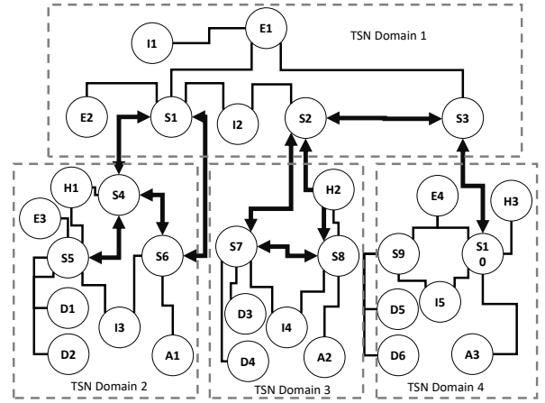
Fig. 3. QCAP redundant industrial network.
