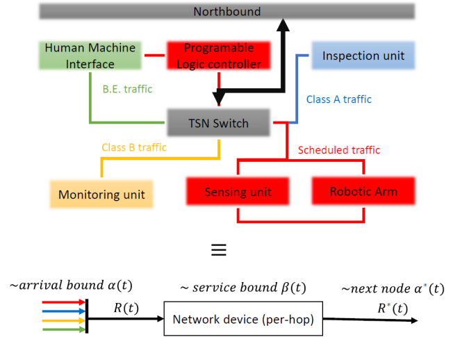
Fig. 1. Single hop model of QCAP TSN node.
