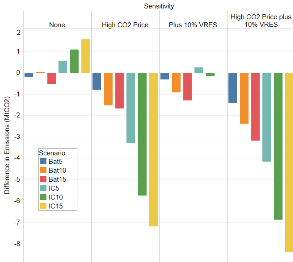
Figure 4-4: Difference in emissions compared to the relative basecase
