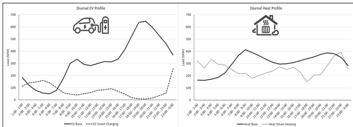
Figure I-11: Diurnal EV and Heating profiles used in the study
