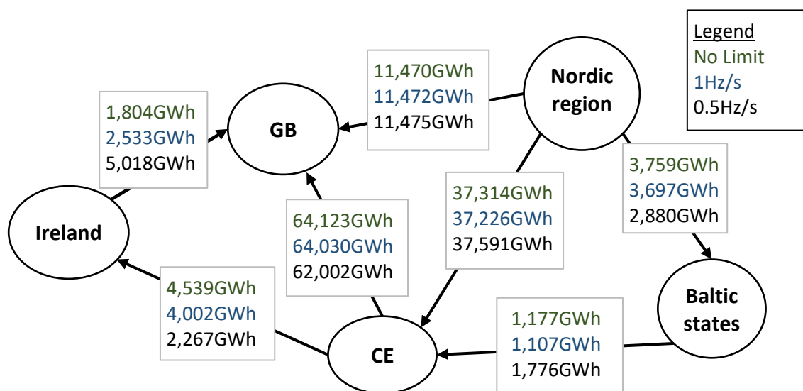
Figure 3-4: Net interchange between synchronous areas for each ROCOF level in Scenario 1
