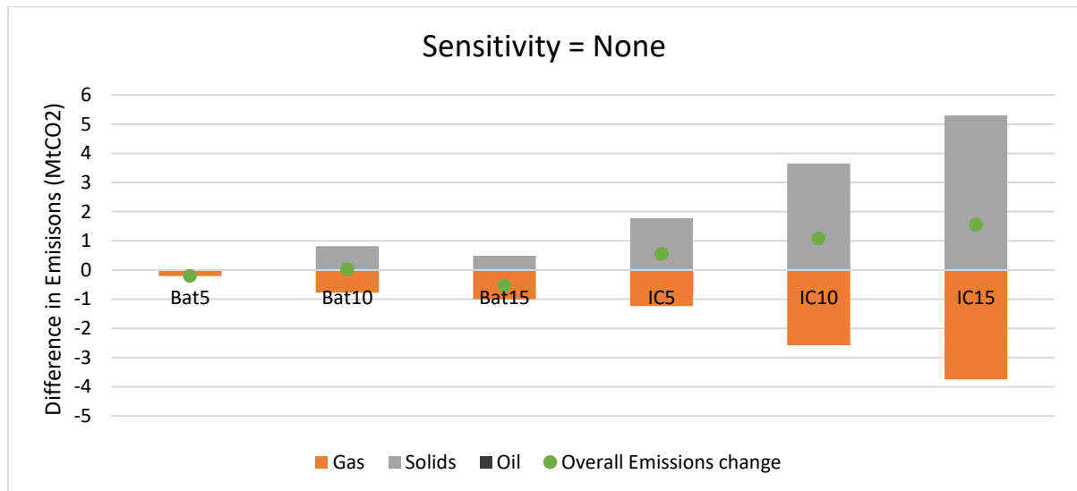
Figure 4-5: Difference in emissions production by fuel type and overall emissions for scenarios with Sensitivity = None compared to basecase
