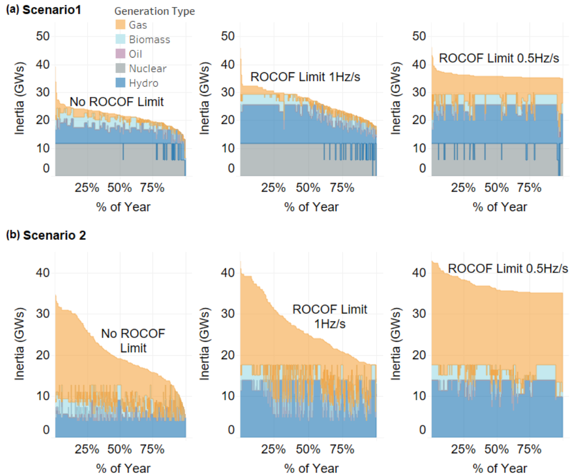
Figure 3-7: Hourly Inertia contribution by generation types for Baltic area for (a) Scenario 1 and (b) Scenario 2 ranked by total inertia as a percentage of year
