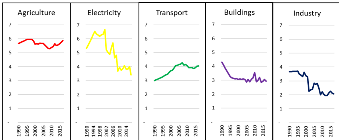
Figure I-3: Northern Ireland Greenhouse gases from 1990-2017 for major sectors of the economy
