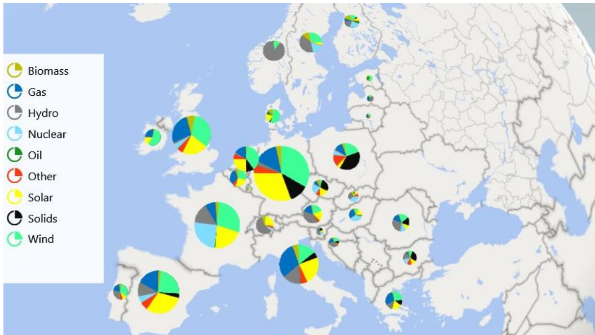
Figure I-7: EU wide power system portfolios considered in this analysis. Portfolios and interconnection capacities (except the All-Island System) are from ENTSO-E 2018 TYNDP
