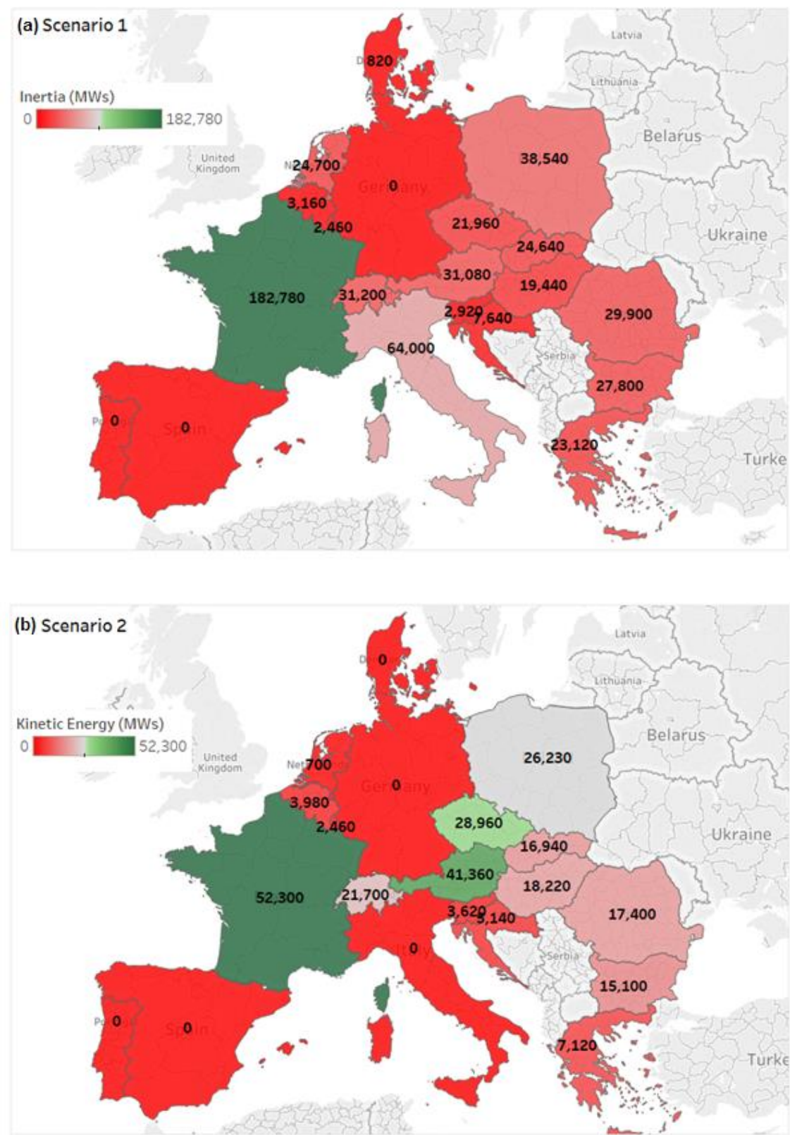
Figure 3-8: Contribution per country at lowest hourly inertia across CE for (a) Scenario 1 and (b) Scenario 2
