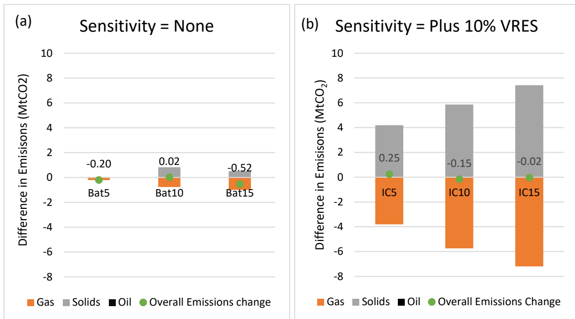
Figure 4-7: Difference in emissions production by fuel type and overall emissions compared to the relative basecase for (a) No sensitivity and (b) Plus 10% VRES capacity
