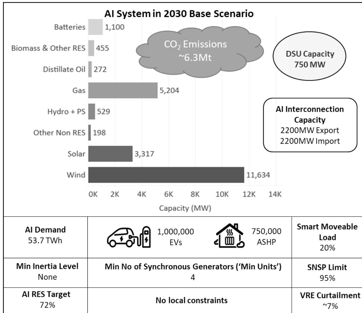
Figure I-12: Overview of 2030 Base scenario
