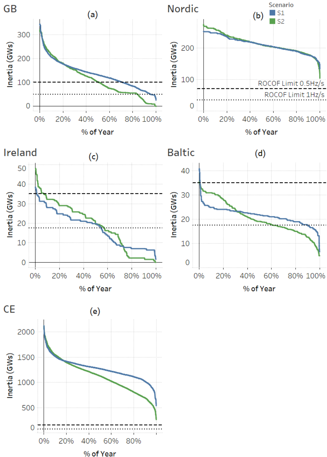
Figure 3-2: Inertia duration curves for all synchronous grids with no ROCOF limit
