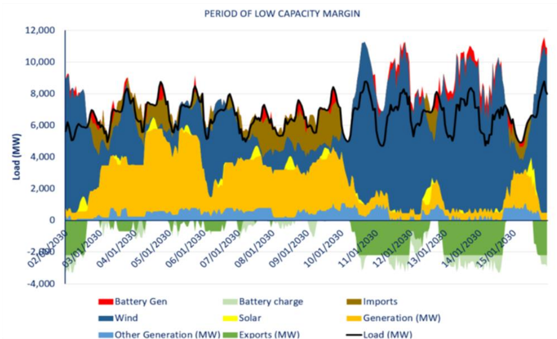
Figure I-16: Weather Years Scenario: A) High wind period, B) Low wind period, C) High gas generation period and D) Low capacity margin.
