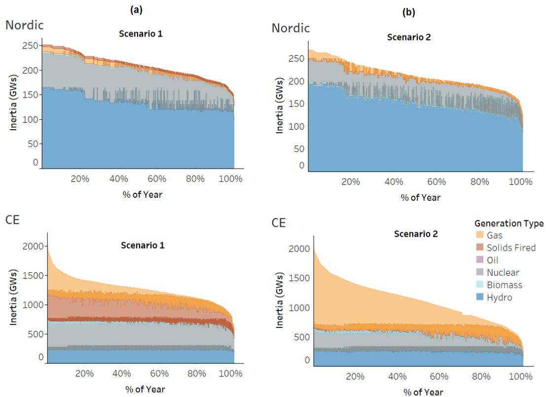
Figure 3-3: Inertia contribution by generation type for the Nordic and CE synchronous areas for (a) Scenario 1 and (b) Scenario 2 with no ROCOF Limit
