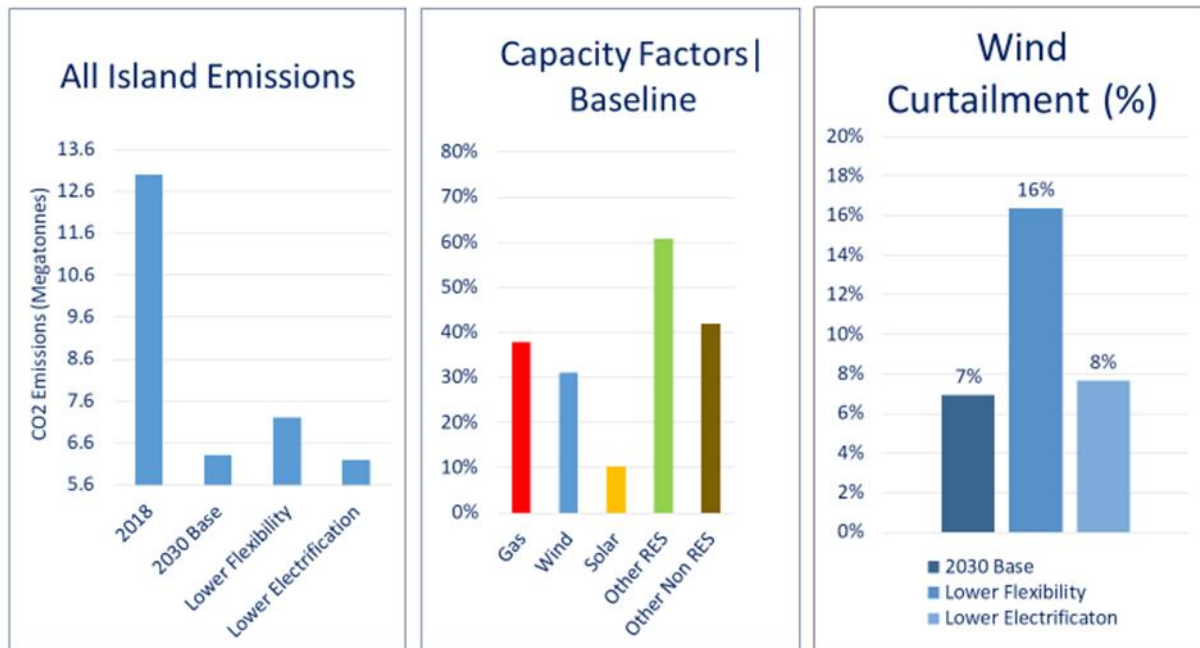
Figure I-15: CO 2 Emissions, Capacity Factors and wind curtailment for presented scenarios
