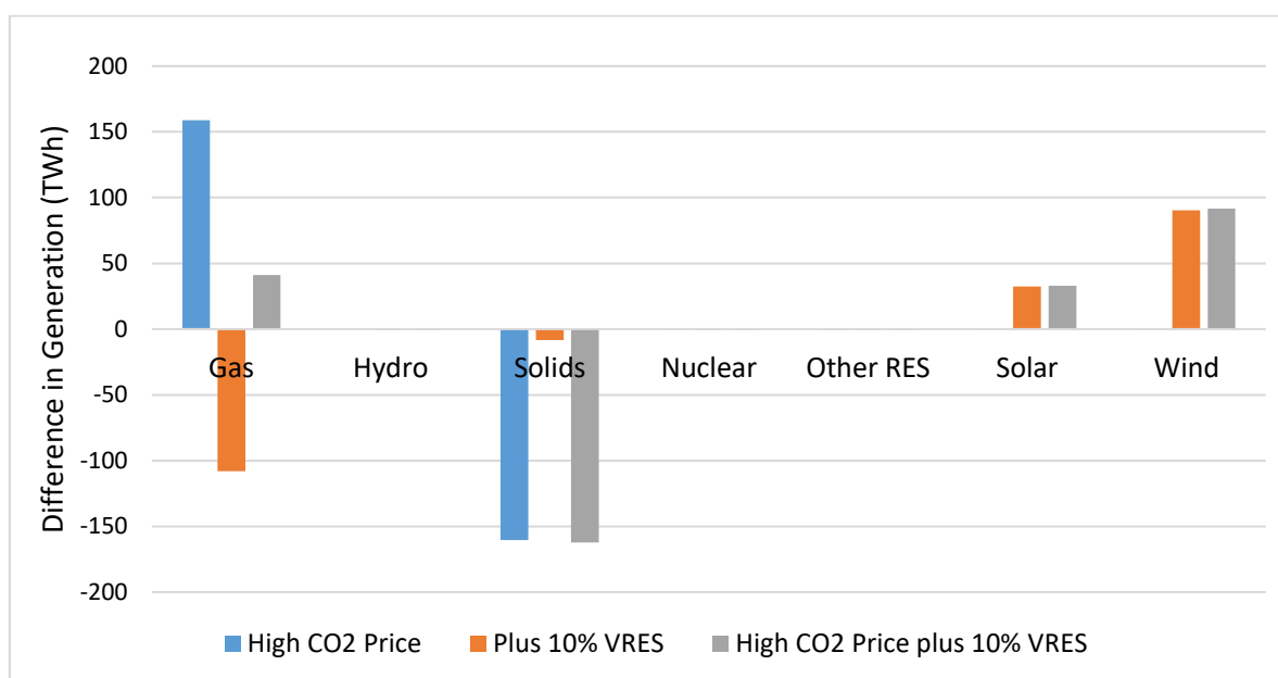
Figure 4-2: Difference in production by fuel type compared to basecase for each sensitivity
