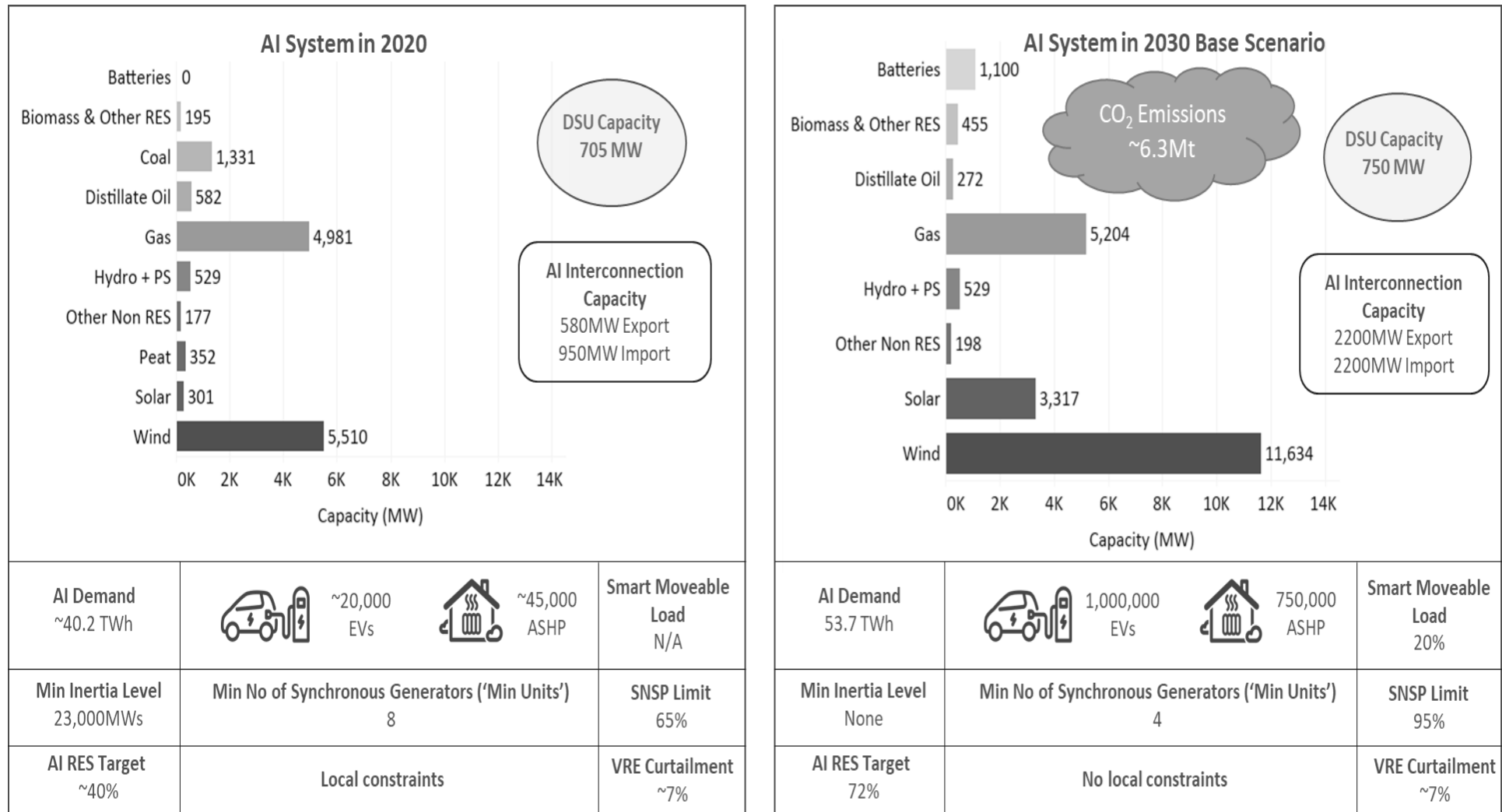
Figure A-2: Comparison of 2020 to 2030 Base Scenario
