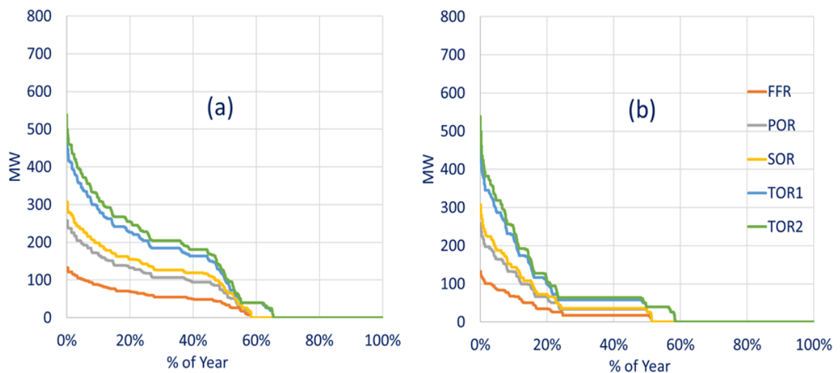
Figure I-20: Reserve available from conventional generation for (a) 2030 Base scenario and (b) 2030 Base scenario with Min Units constraint removed
