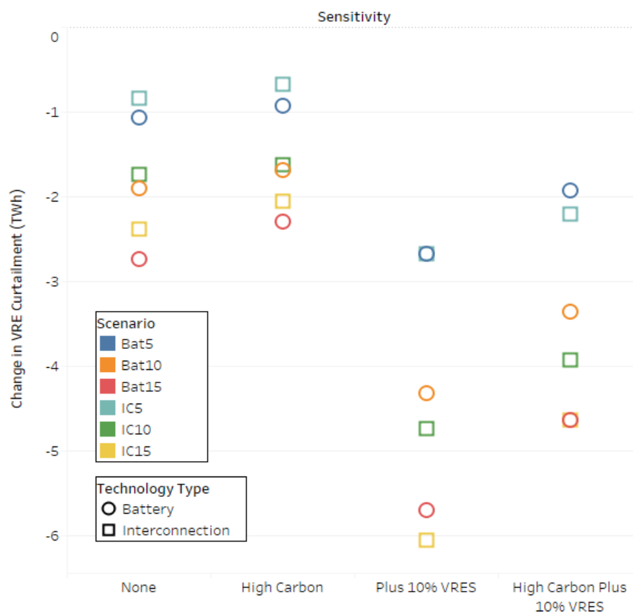
Figure 4-8: Change in VRE curtailment relative to comparable basecase and sensitivity
