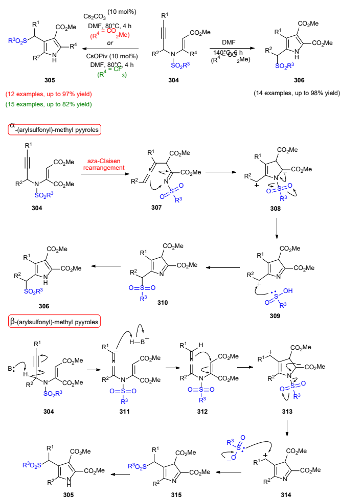
Scheme 45: 1,3- and 1,4-sulfonyl migration in the generation of both \alpha - and \beta -(arylsulfonyl)methyl pyrroles under thermal and basic conditions respectively
